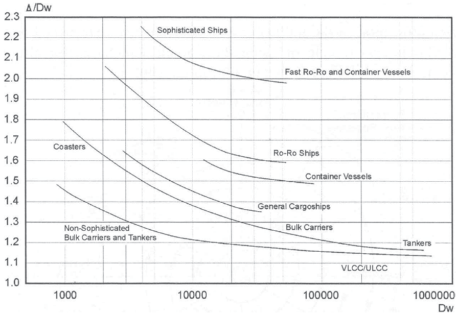
Fig. 2.3 ( \Delta/DWT ) ratios versus DWT for various ship types, Harvald (1986) (see Friis et al. 2002)
