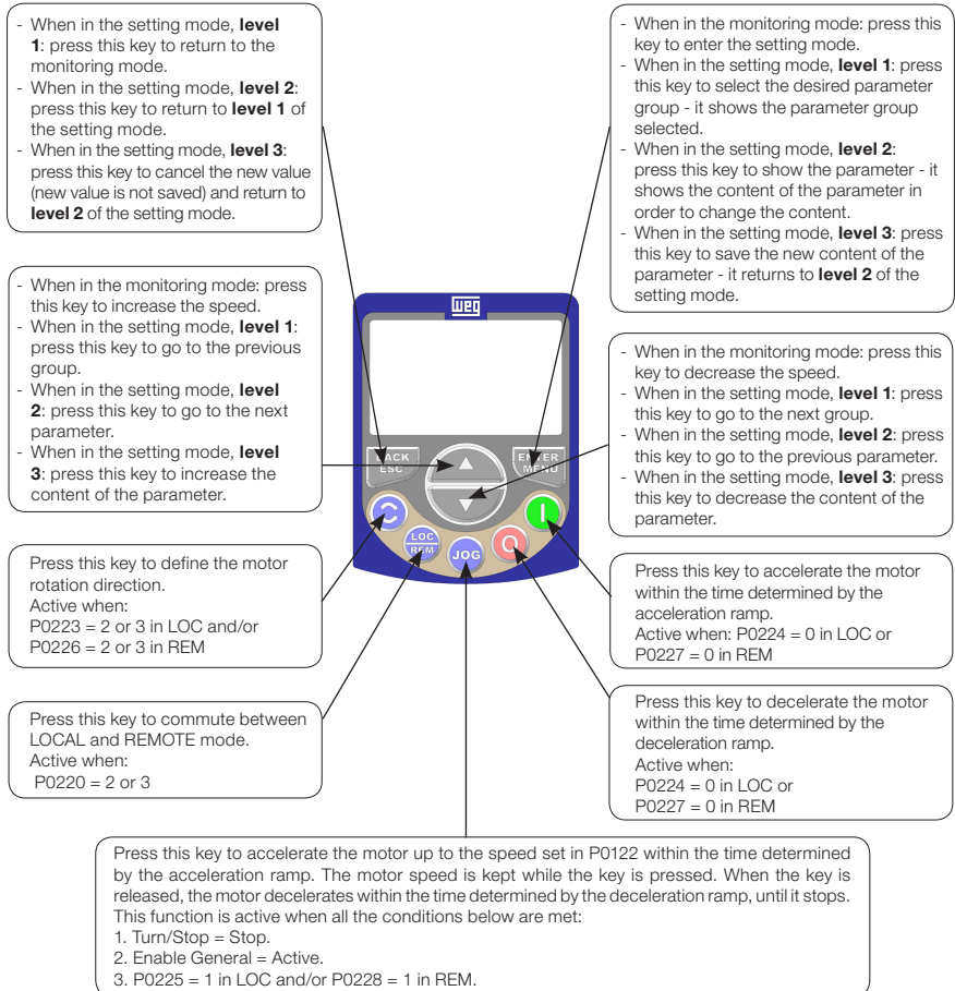
Figure 4.1: HMI Keys
