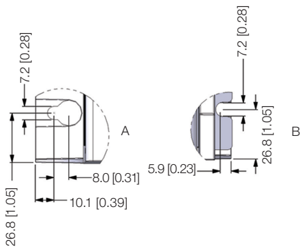
Figure B.8: Inverter dimensions in mm [in] - frame size D
