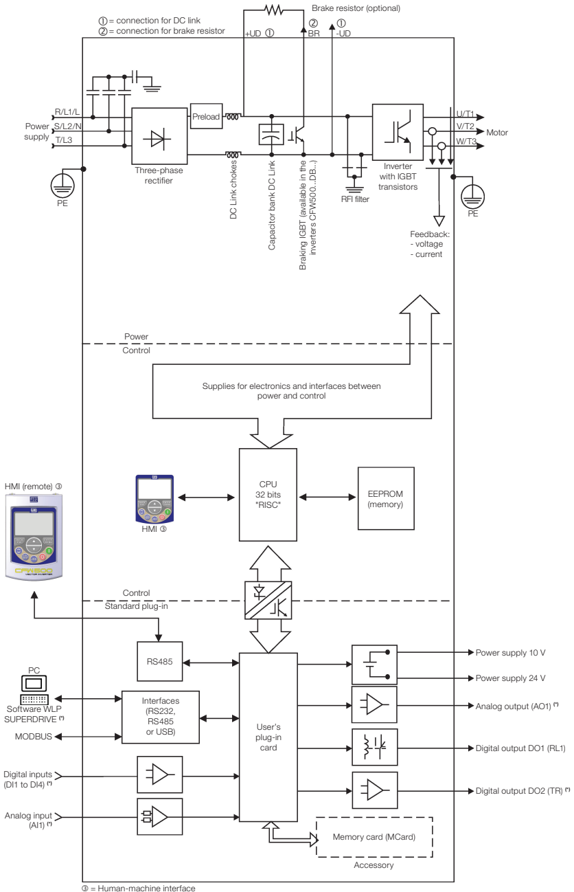
Figure 2.3: Block diagram of CFW500 for frame size F
