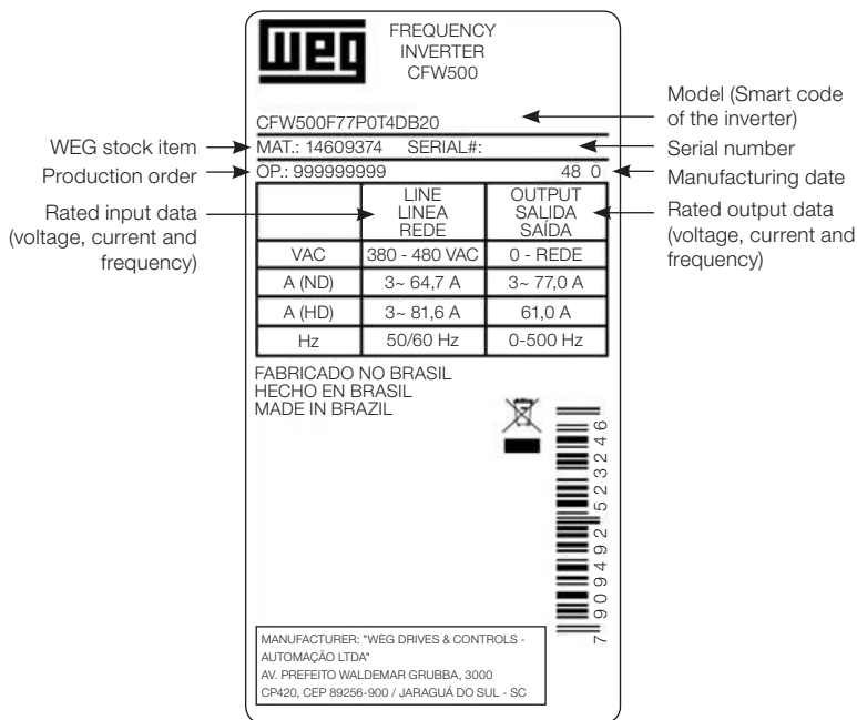
b) Side label of the CFW500 - frame size F
