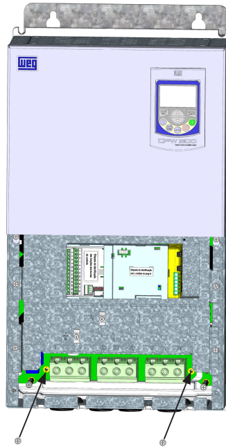
Figure A.4: Location of filter capacitors ground disconnection points - disconnection trough bolts - frame size F
