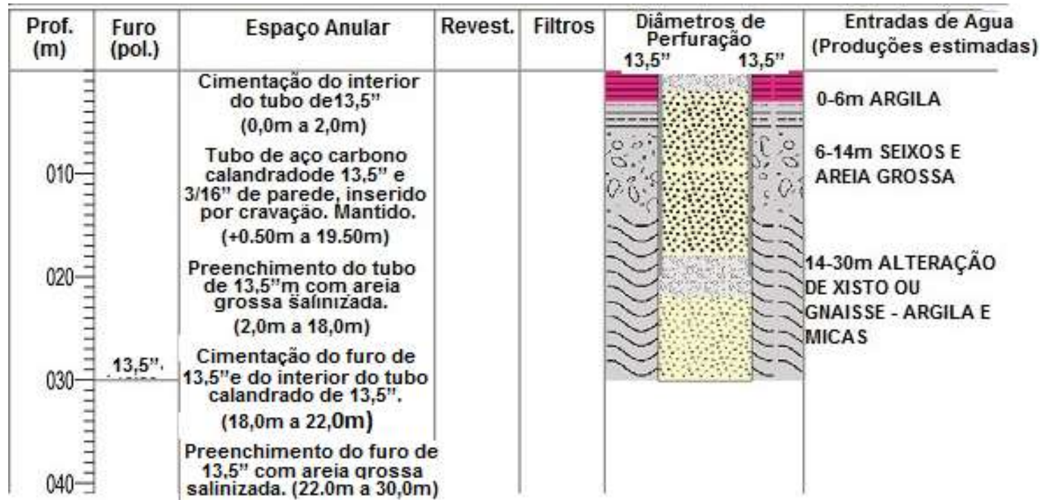
Figura 12 – Perfil do poço P4-L3, perfurado no ponto 750m da Linha B Figure 12 - Well profile P4-L3, drilled in point 750 meters of Line B
