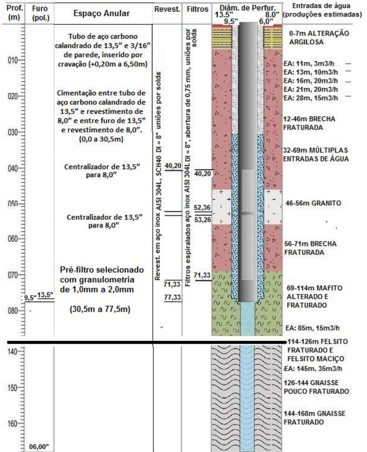
Figura 14 – Perfil do poço P3-L6, perfurado no ponto 2340m da Linha B Figure 14 - Well profile P3-L6, drilled in point 2340 meters of Line B
