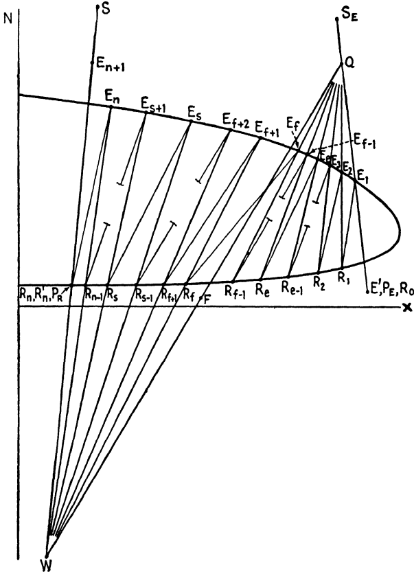
FIG. 6.56. Countercurrent multiple contact with extract and raffinate reflux, Janecke coordinates.
