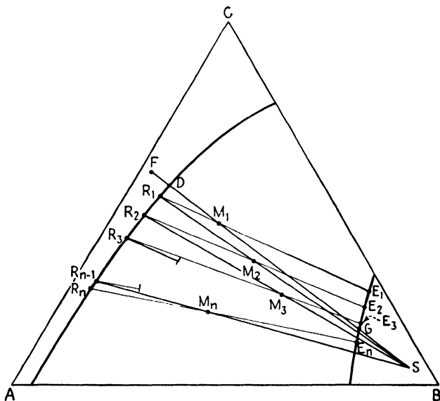
FIG. 6.19. Cocurrent multiple contact in a Type 2 system.
