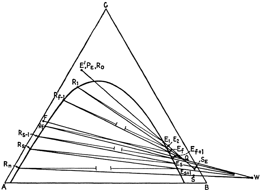
Fig. 6.62. Countercurrent extraction with extract reflux.
