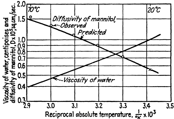
FIG. 5.5. Effect of temperature on the diffusivity of mannitol in water solution.
