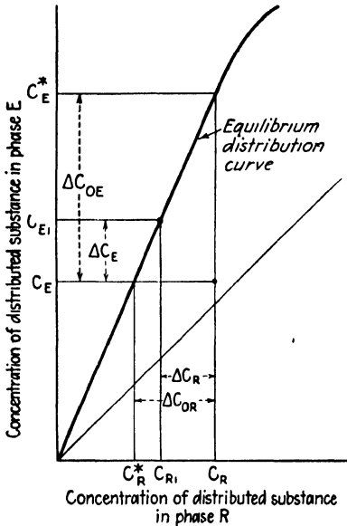
FIG. 5.9. Over-all and individual film driving forces.
