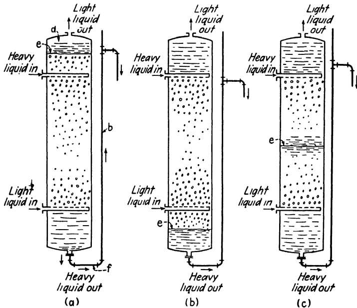
FIG. 10.1. Spray tower.
