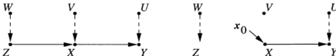
Figure 1 An example of DAG. From reference 7. The letters indicate "nodes" in the graph and stand for variables in the causal model. Arrows ("edges") represent relationships. Unobserved exogenous variables are connected by dashed arrows.
