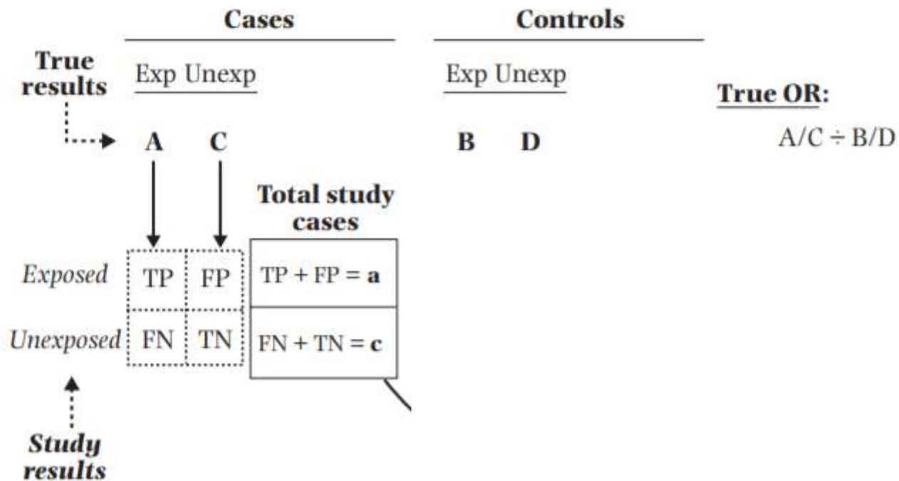
FIGURE 4-4 Application of sensitivity/specificity concepts in misclassification of exposure: schematic representation of true and misclassified relative odds. Sensitivity of exposure ascertainment = TP \div (TP + FN) ; specificity of exposure ascertainment = TN \div (TN + FP) .
