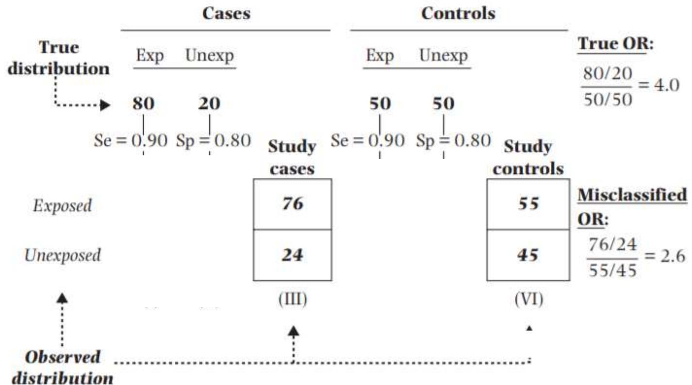
EXHIBIT 4-3 Effects of nondifferential misclassification on the odds ratio (sensitivity = 0.90; specificity = 0.80).
