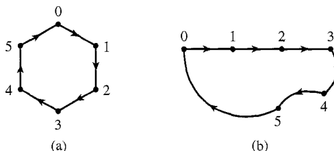
7.8 Figure Two digraphs for \mathbb{Z}_6 with S = \{1\} using \xrightarrow{1} .
