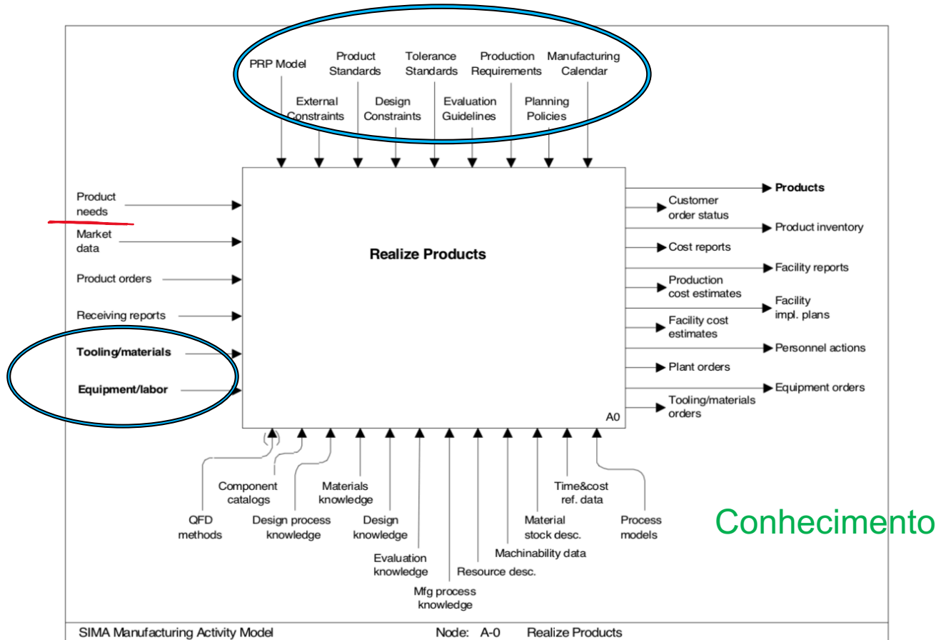
Figure 1. High-level View of Product Realization Activities
