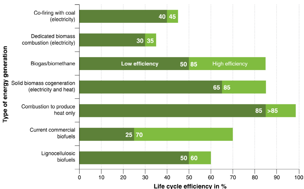
Figure 12.2. Net efficiency range of biomass-to-energy pathways on a life cycle basis from harvested crop to power, heat, and biofuels considered by the (EEA 2013) for current applications and developing lignocellulosic biofuels. Reproduced with permission from EEA.
