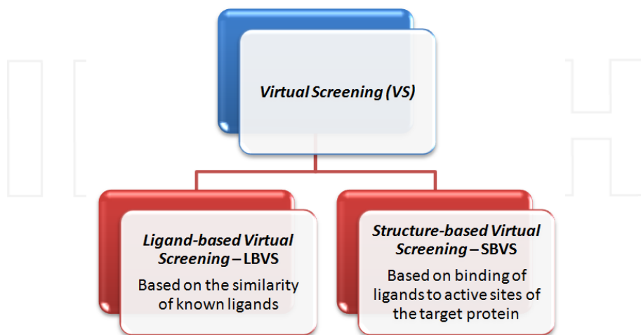
Figure 1. Virtual screening can be divided into ligand-based virtual screening (LBVS) and structure-based virtual screening (SBVS).
