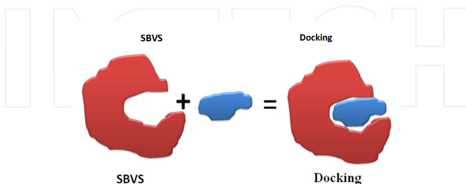
Figure 8. Diagram illustrating the docking of a ligand to a receptor to produce a complex.
