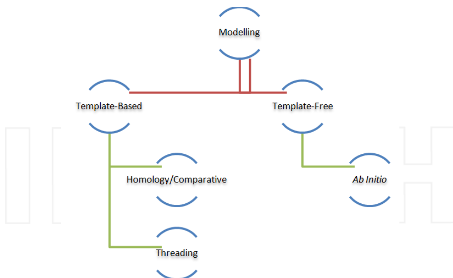
Figure 3. Modelling methods can be classified into template-based methods (homology/comparative modelling) and template-free methods ( ab initio ).
