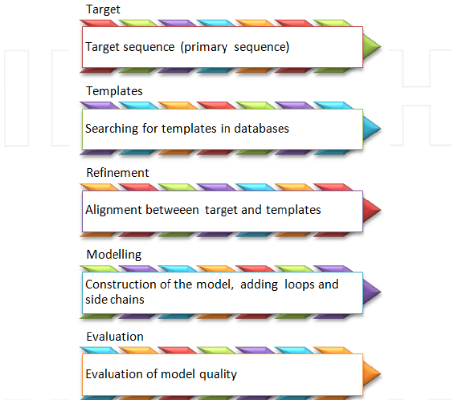
Figure 4. Steps in the comparative modelling process.
