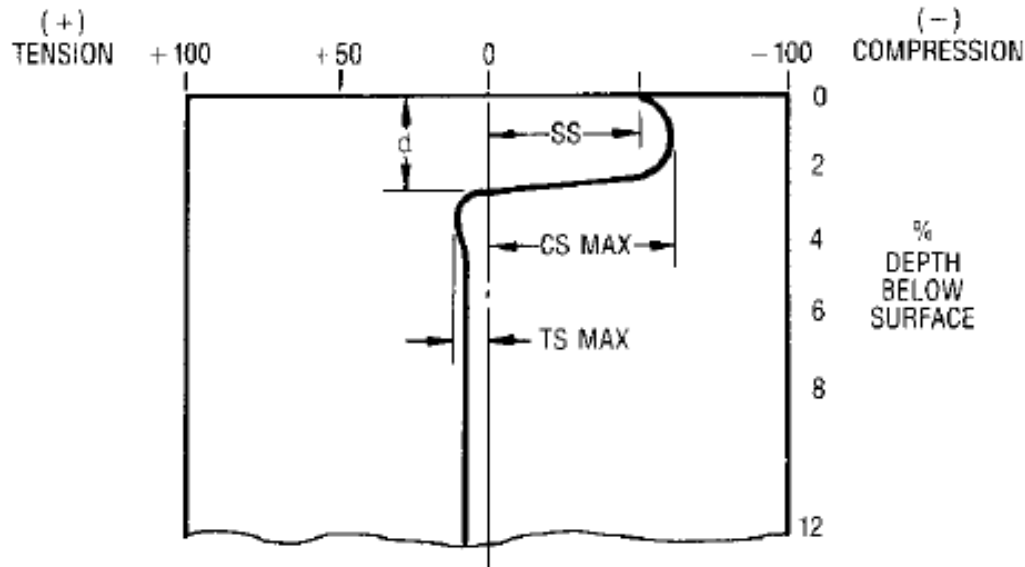
Example of Residual Stress Profile Created by Shot Peening
