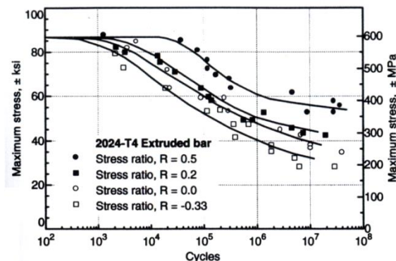
Fig. 15 2024-T4 unnotched axial fatigue (extruded bar). Unnotched axial specimens with 9-7/8 in. surface radius and 0.158 in. minimum diameter. Source: Alcoa, 1954
