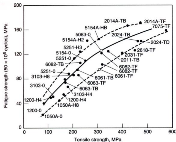
Fig. 5 Relationships between the fatigue strength and tensile strength of some wrought aluminum alloys
