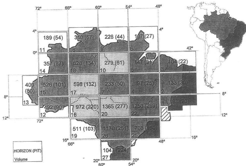
Fig. 2. Localization of the area surveyed by the RADAMBRASIL project. Extent of the area described in each volume, number of the horizon analyzed and, in brackets, number of the corresponding pit.
