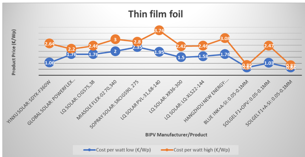
Fig. 13. BIPV thin-film foil products vs steel + IL (0.05–0.1 mm).
