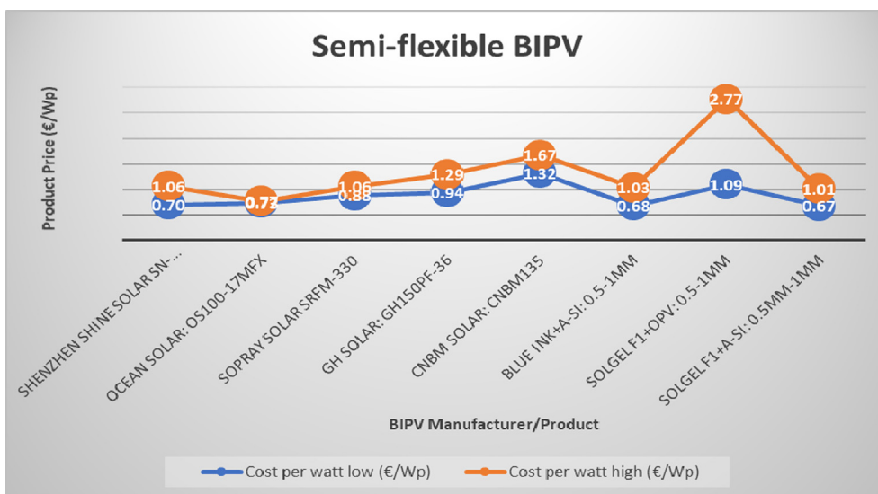
Fig. 12. BIPV semi-flexible products vs steel + IL (0.5–1 mm).
