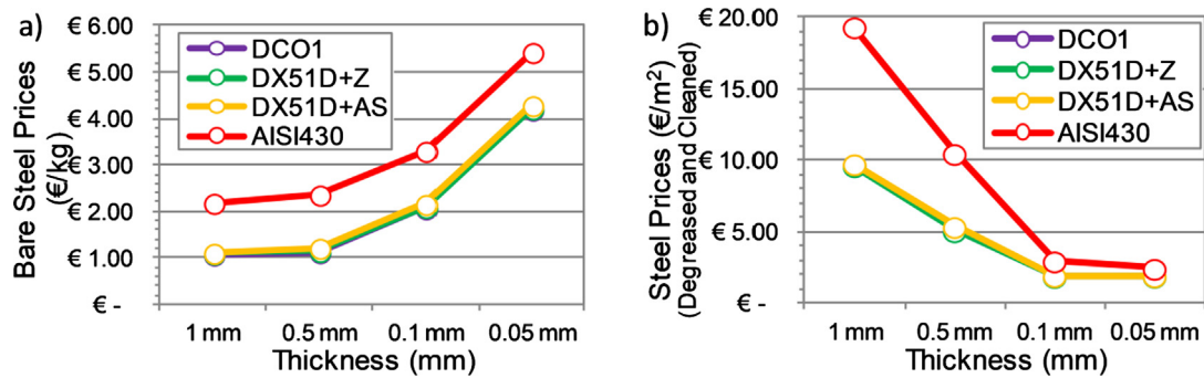
Fig. 8. Steel prices [55]: (a) Price per kg for bare steel; and (b) Price per m 2 for prepared steel ready for IL processing.
