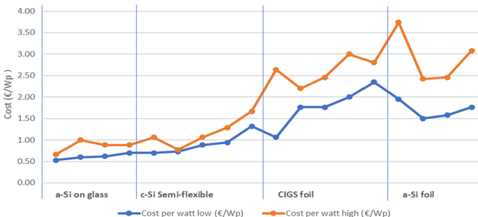
Fig. 5. Factory gate price distribution of BIPV by product category in €/W p as of March 2018.
