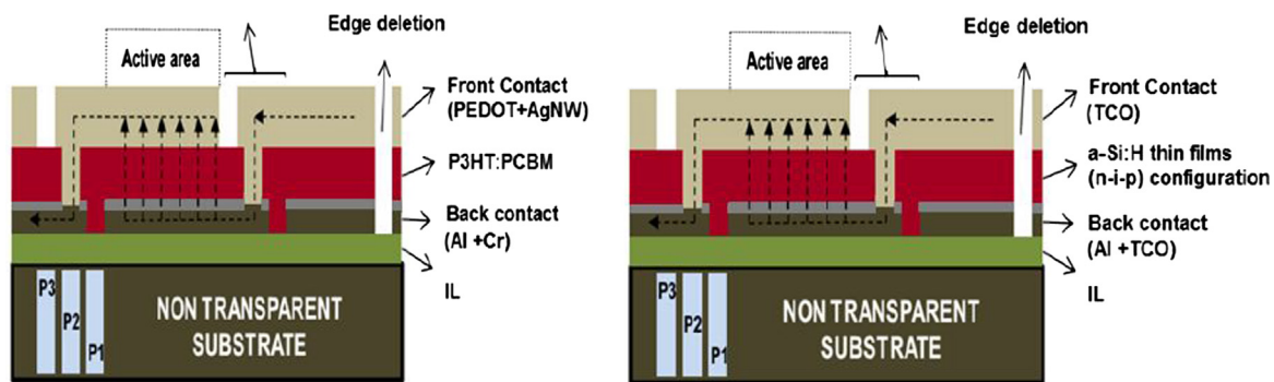
Fig. 1. (a) PV structure of an OPV example, where PEDOT = poly(3,4-ethylenedioxythiophene), AgNW = silver nanowires, P3HT = Poly(3-hexylthiophene), PCBM = [6,6]-phenyl-C61-butyrac methyl ester, Al = Aluminium, Cr = Chromium and IL = Intermediate layer and (b): PV structure of an a-Si example where TCO = transparent conducting oxide.
