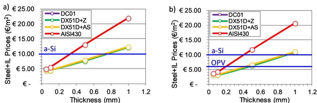
Fig. 10. Processed Steel + IL substrate prices showing the target prices for PV technologies: (a) Blue Ink (a-Si only); (b) SolGel F1 (OPV & a-Si). (For interpretation of the references to colour in this figure legend, the reader is referred to the web version of this article.)
