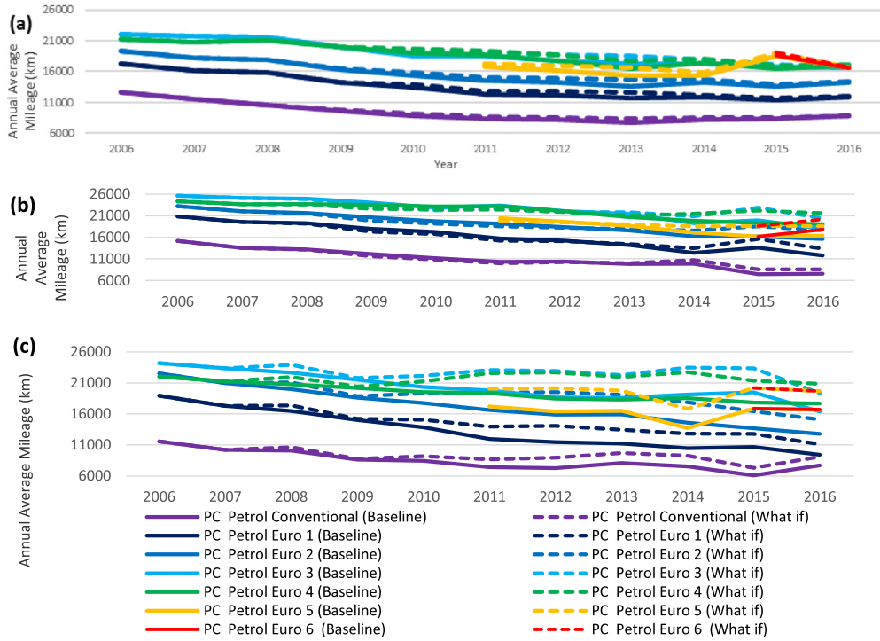
Fig. 7. Annual average mileage for petrol powered PC: (a) <math>< 1.4\text{ L}</math>; (b) <math>1.4\text{--}2\text{ L}</math>; (c) >2 L
