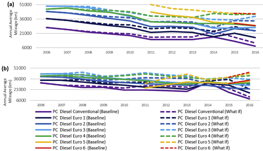
Fig. 8. Annual average mileage for diesel powered PC: (a) <math>< 2\text{ L}</math>; (b) >2 L
