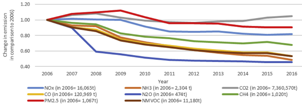
Fig. 9. Emissions in 'what-if' scenario.
