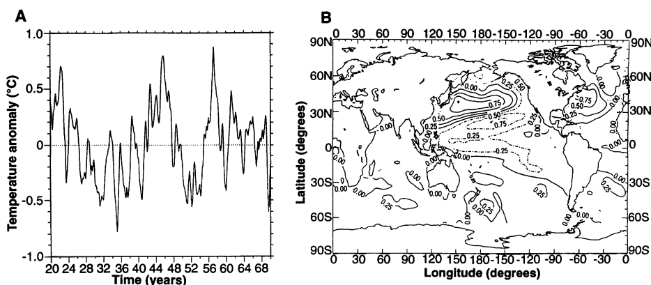
Fig. 1. (A) Time series of the coupled model's anomalous SST (°C) averaged over the region from 150°E to 180°E and 25°N to 35°N. The time series was smoothed with a 9-months running mean filter. (B) Spatial distribution of linear regression coefficients between the index time series shown in (A) and SST values. The pattern was scaled so that the maximum SST anomalies were to 1°C.
