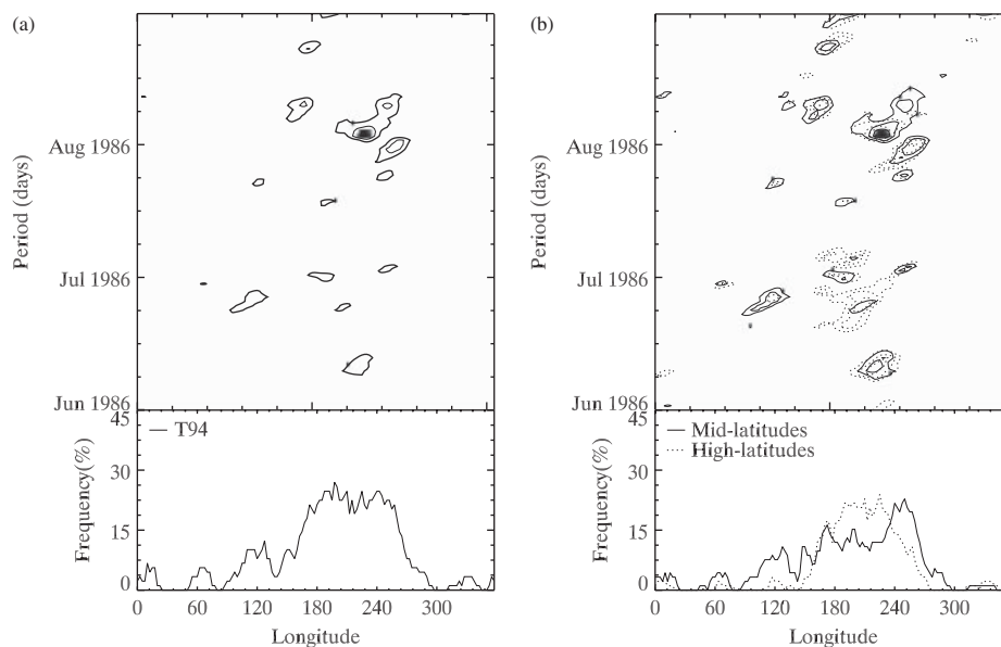
Figure 2. Hovmöller diagrams (longitude-time) of the strength of the blocking flows ( m^{\circ} latitude) and their respective frequencies per longitude for the austral winter of 1986: (a) T94 scheme; (b) mid-latitude (solid lines) and mid-high (dotted lines) latitude references of blocking index (see text for further details).
