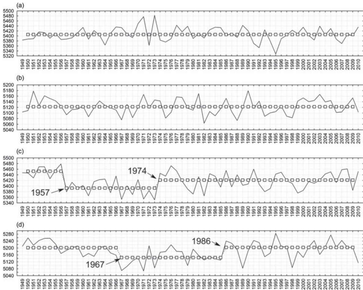
Figure 1. Mean fields of 500-hPa geopotential height (solid lines) with a stepwise trend (squared lines) for 180° of longitude at (a) mid-latitudes (35°S–50°S) and (b) mid-high latitudes (55°S–70°S) and for 135° of longitude at (c) mid-latitudes (35°S–50°S) and (d) mid-high latitudes (55°S–70°S) from the period 1950 to 2010.
