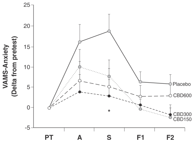
Figure 1 Visual Analogue Mood Scale (VAMS) anxiety factor scores in each phase of the simulated public speaking test (SPST) for groups treated with cannabidiol (CBD) 150, 300, and 600 mg or placebo (points in the curve refer to mean scores and vertical lines refer to mean standard errors). * Lower anxiety levels in the group treated with CBD 300 mg relative to the placebo phase ( p = 0.042 ). PT = pre-test; A = anticipatory anxiety; S = speech; F1 = post-test 1; F2 = post-test 2.
