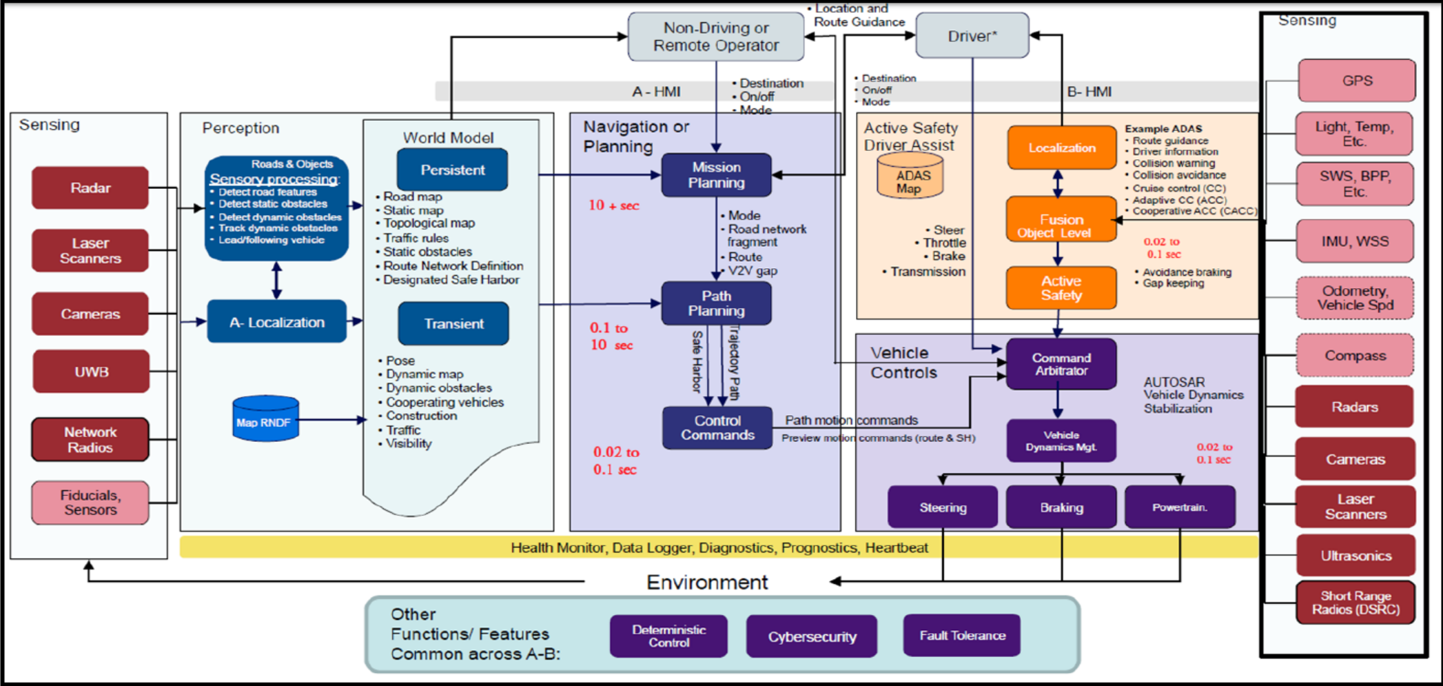
Figure 2. SAE International Autonomous Mode Functional Architecture Flow Diagram (Underwood, 2016)
