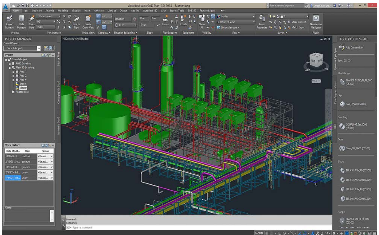
Figure 24: Federated model for process plant
