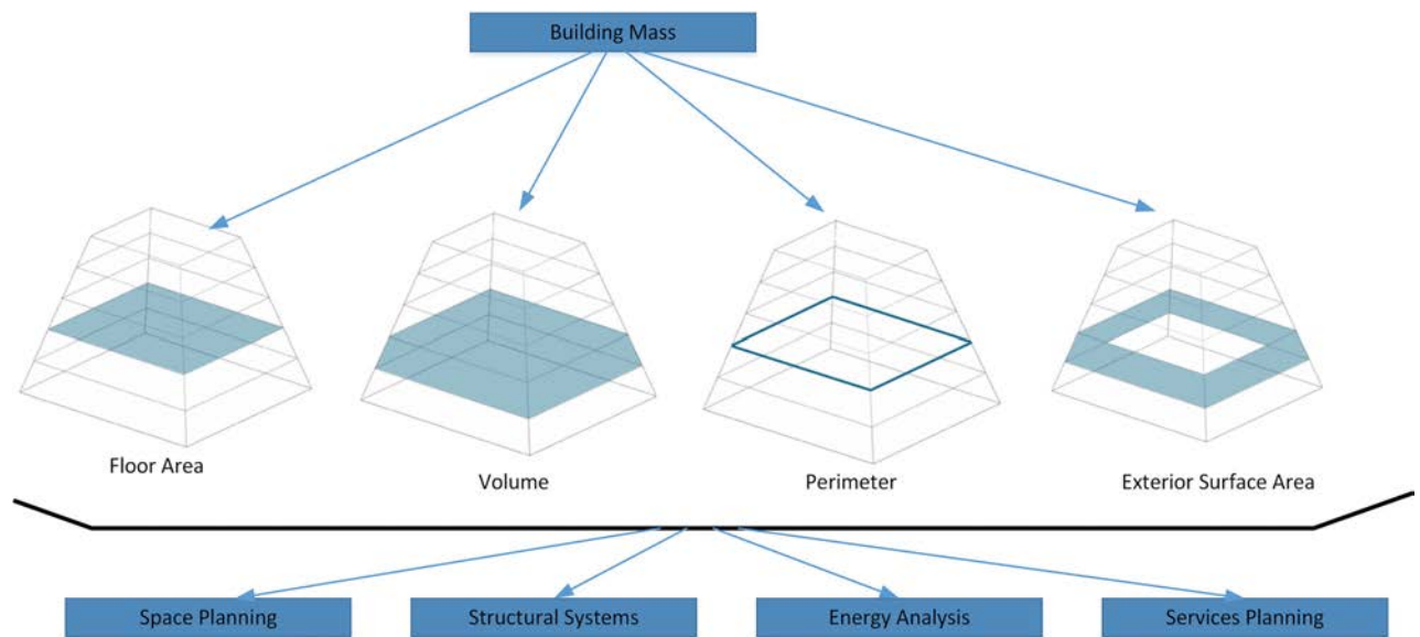
Figure 45: Workflow for analysis using a mass model
