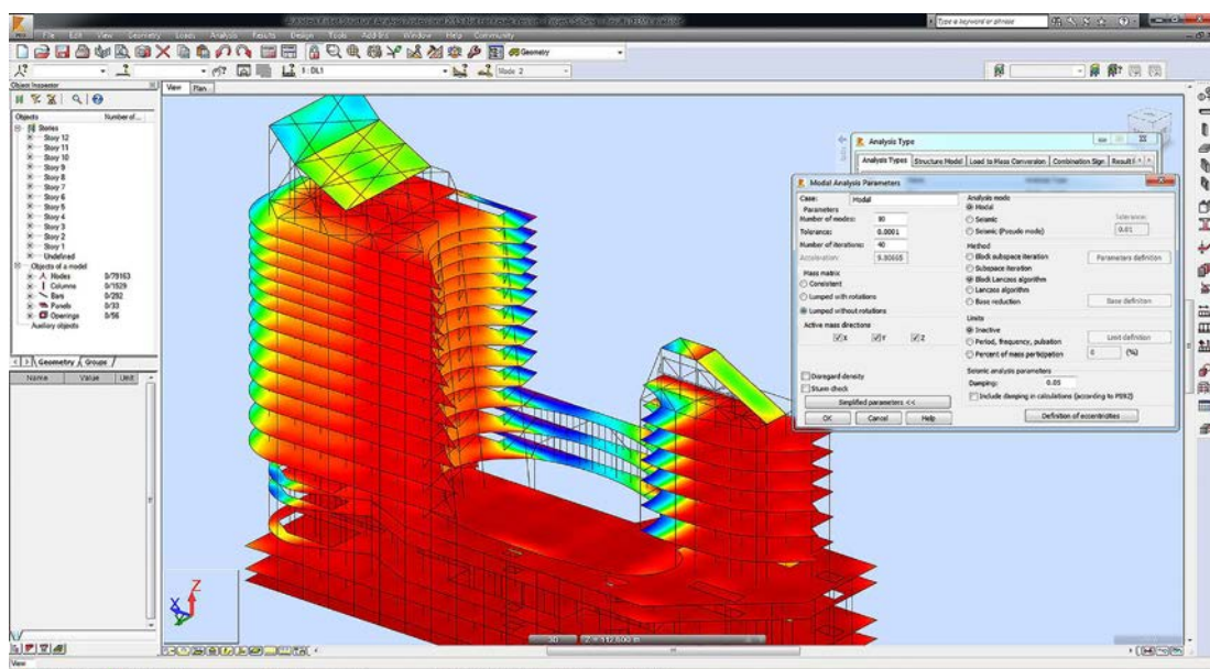
Figure 47: Structural analysis using concept-stage model
