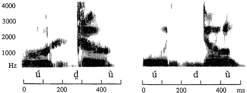
Figure 2.8 Spectrograms illustrating the difference between a laminal dental \mathfrak{d} and an apical alveolar d in Isoko in the words \acute{u}\mathfrak{d}\grave{u} 'farm' and \acute{u}\mathfrak{d}\grave{u} 'chest'.
