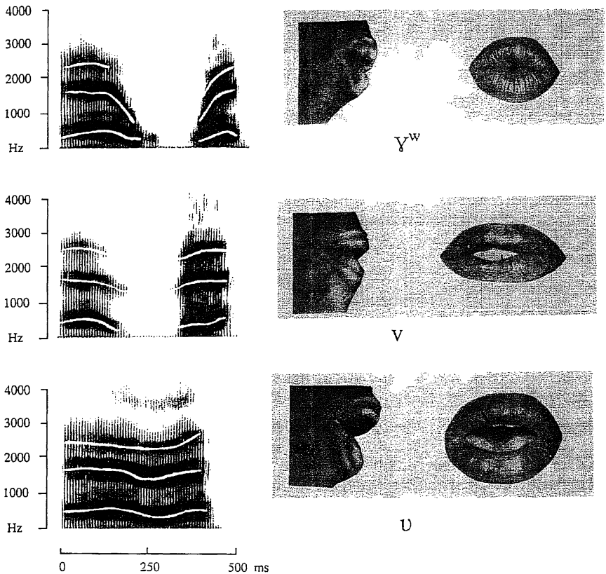
Figure 9.33 Photographs of the lips in the Isoko words éy w é 'hoe', évé 'how' and éuvé 'breath'. The photographs were determined to be in the middle of the consonants by observing the click of the camera shutter on a simultaneous recording. The spectrograms on the left are of repetitions of these words recorded immediately after the photographic session. Center formant frequencies have been outlined in white.
