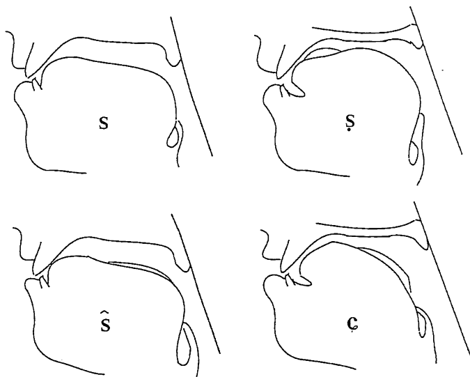
Figure 5.18 The four contrasting gestures for the sibilant fricatives in the Bzyb dialect of Abkhaz, based on x-ray tracings from Bgazhba (1964) and interpretive comments by Catford ( ms in preparation ).
