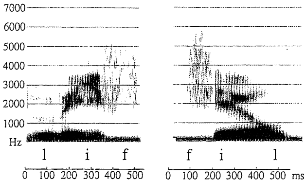
Figure 10.20 Spectrograms of an American English speaker's pronunciation of leaf , feel using velarized laterals in both words.
