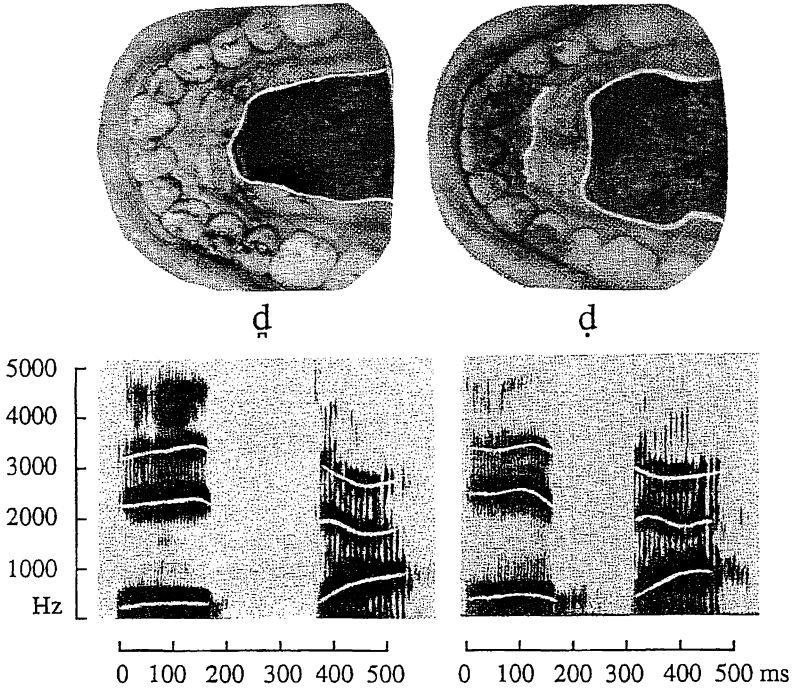
Figure 2.10 Spectrograms and palatograms illustrating the difference between laminal denti-alveolar \text{ɗ} and apical retroflex \text{ɗ̡} in Ewe in the phrases \text{é ɗ̡} 'he throws' and \text{é ɗ̡} 'he cooks', based on Ladefoged (1968).
