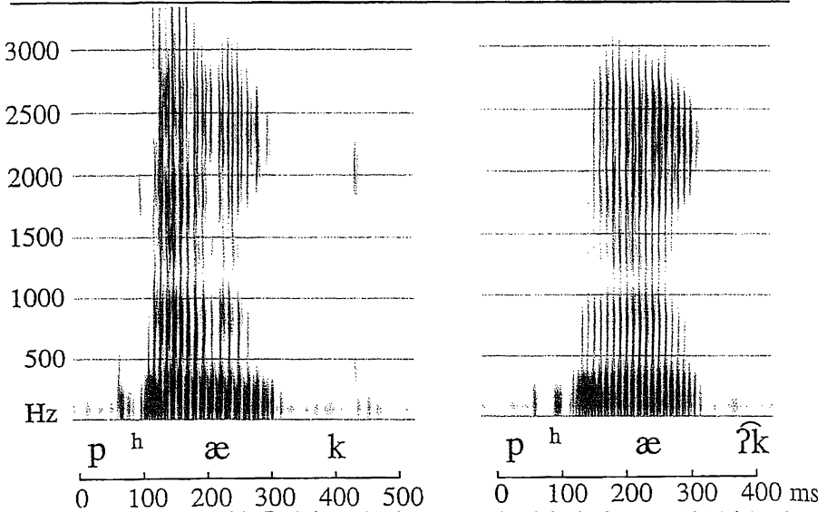
Figure 3.12 Spectrograms of the English word pack pronounced with final velar stop with (right) and without (left) accompanying glottal closure.
