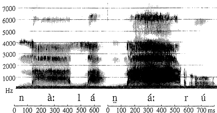
Figure 4.4 Spectrograms of Tsonga modal and breathy voiced nasals in the words nàlá 'enemy' and nárú 'three', as spoken by a male speaker.
