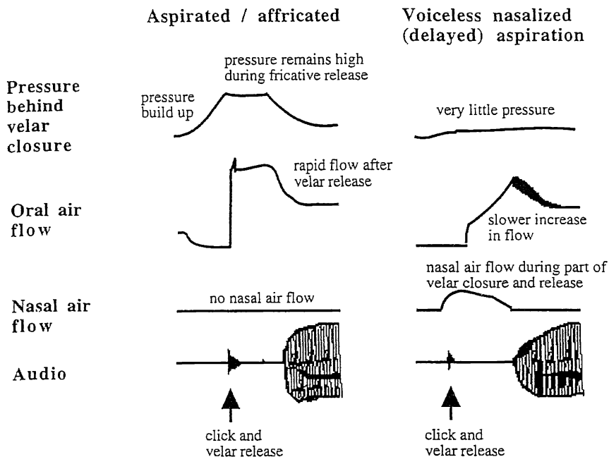
Figure 8.9 Aerodynamic records (retouched) illustrating the difference between the aspirated (velar affricated) and voiceless aspirated nasalized (delayed aspirated) clicks in the Nama words k^h'o 'play music' and \eta^h'o 'push into', pronounced as citation forms. Only the beginning of each word is shown.
