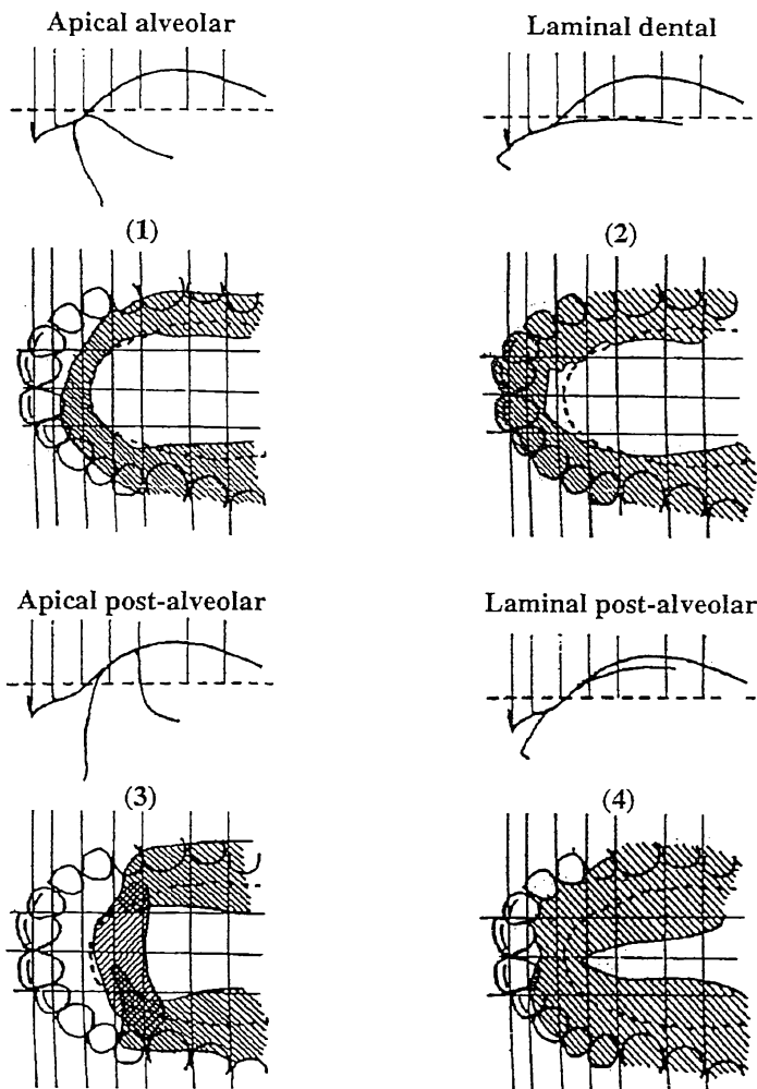
Figure 2.12 Palatograms and inferred articulatory positions for intervocalic coronal stops in Eastern Arrernte (courtesy of Andrew Butcher). The words illustrated are (1) aṭamə 'burst', (2) aṭamə 'grind', (3) kwəṭə 'smoke', (4) aṭaməjə 'mother's father'.
