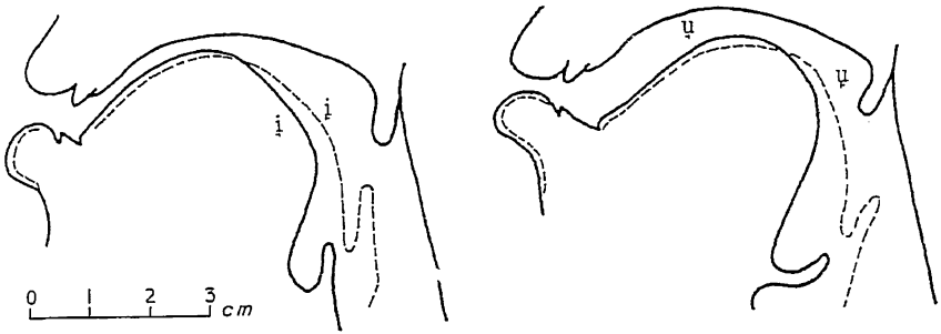
Figure 9.16 Tracings from x-ray cinematography films of Igbo vowels i as in óbi ( óbi in the standard Igbo orthography) 'heart'; i as in ɥbi ( ɥbi ) 'poverty of ability'; ɥ as in jɥ ( ibu ) 'weight'; and ɥ as in ɔbɥ ( obu ) 'it is'. In accordance with current IPA usage ɥ and ɔ are used to indicate Advanced and Retracted Tongue Root, respectively.
