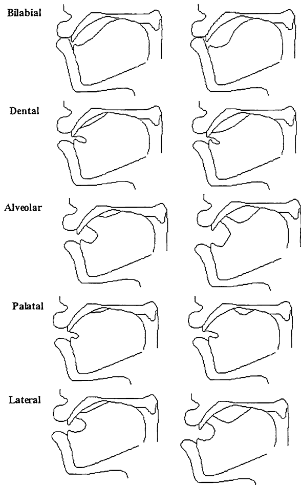
Figure 8.2 The positions of the vocal organs at the onset of the click closure (left column), and just before the release of the click closure (right column) in the five click types of !Xóó, based on cine-radiology data published in Traill (1985).
