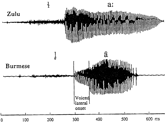
Figure 6.10 Waveforms illustrating differences between a voiceless lateral fricative in the Zulu syllable ʈa: and a voiceless lateral approximant in the Burmese syllable ʎa. The lower amplitude and the anticipation of the voicing in the approximant are apparent.
