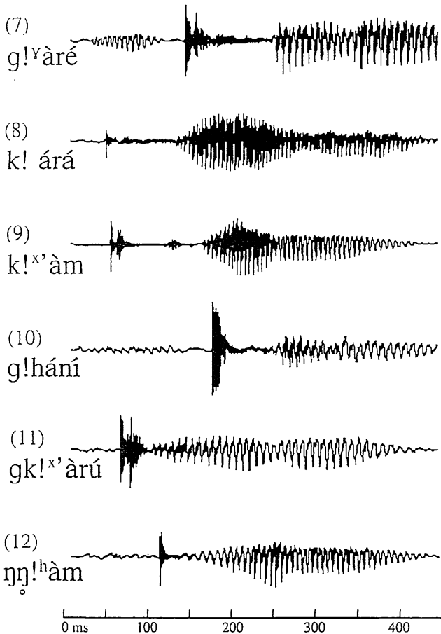
Figure 8.20 Waveforms of the last six Zhuǎhōasi alveolar clicks in table 8.5.
