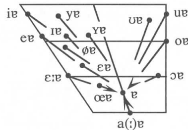
[ɐ] Diphthongs
