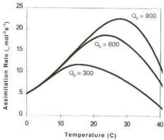
FIGURE 14.5. Temperature response of photosynthesis at three PAR levels for C_{4i} of 240 \mu\text{mol mol}^{-1} .
