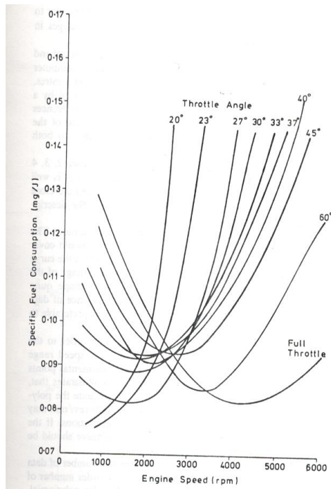
FIGURE 3.4 Specific fuel consumption of 1.6l engine
