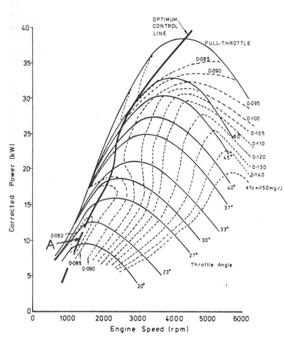
FIGURE 3.5 Characteristics of 1.6l engine
