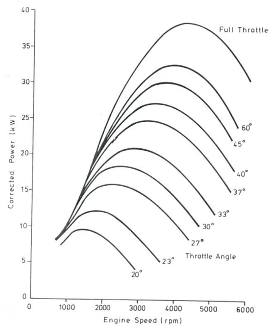
FIGURE 3.3 Engine power curves for 1.6l engine
