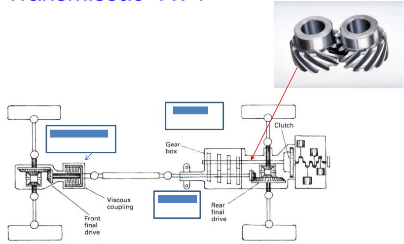
Fig. 7.40 Rear mounted engine four wheel drive system
