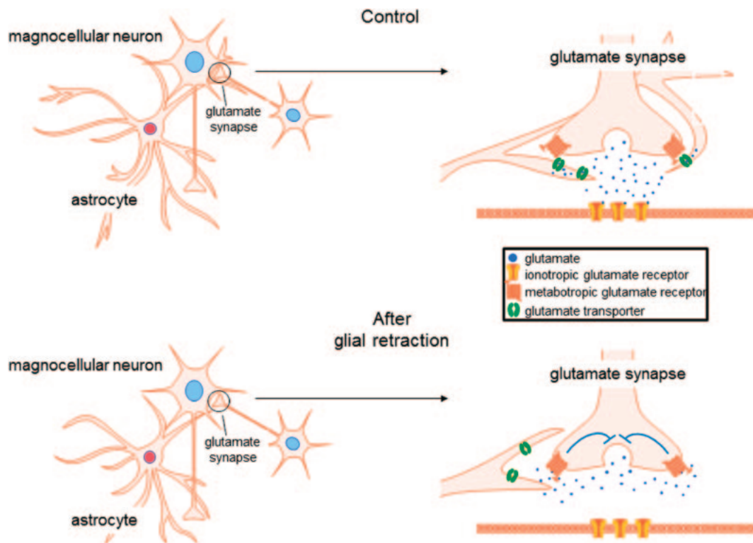
Fig. 4. Glial regulation of glutamate modulation of magnocellular neurons. Under baseline conditions, astrocytes regulate the activation of presynaptic metabotropic glutamate receptors by uptake of extracellular glutamate by glial transporters, which prevents glutamate access to the receptors. Glial retraction uncovers the presynaptic receptors and allows their activation by glutamate, which provides a feedback autoinhibition of glutamate release.
