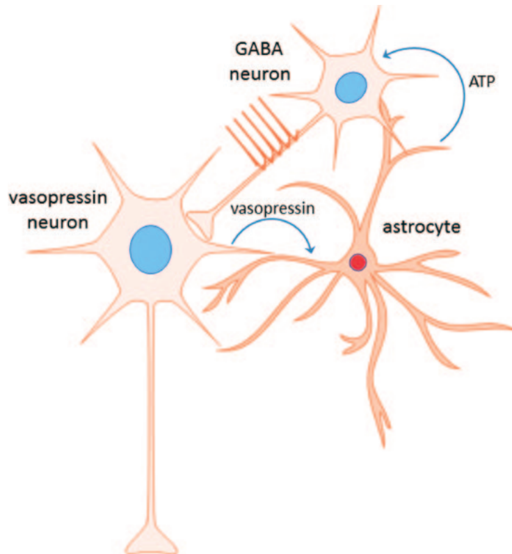
Fig. 6. Model of putative retrograde neuronal-glia-neuronal circuit. Dendritic release of vasopressin stimulates astrocytes, which signal to presynaptic GABA neurons via ATP release. The upstream GABA neurons respond with action potentials and an increase in GABA release back on the vasopressin neurons.
