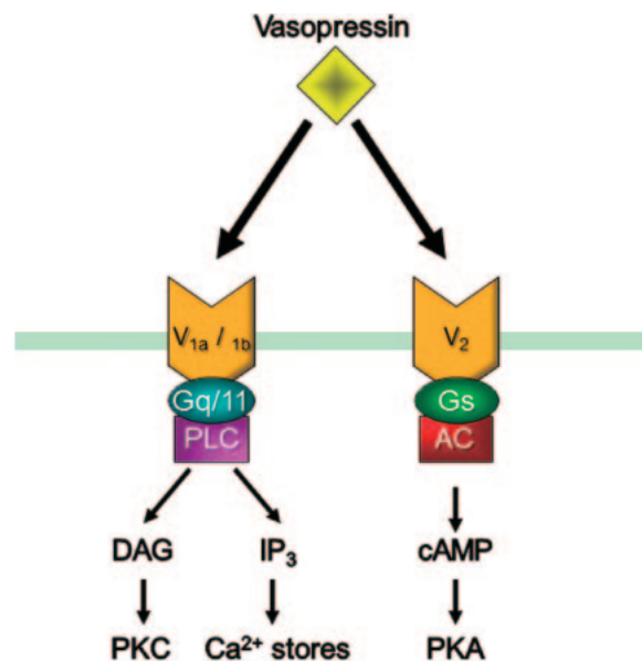
Fig. 2. Vasopressin receptors. There are three known vasopressin receptors, V1a, V1b and V2 receptors, all of which are G protein-coupled receptors. V1a and V1b are coupled to Gq/11 and the IP3/DAG signaling pathway, and V2 receptors are coupled to Gs and the cAMP signaling pathway.
