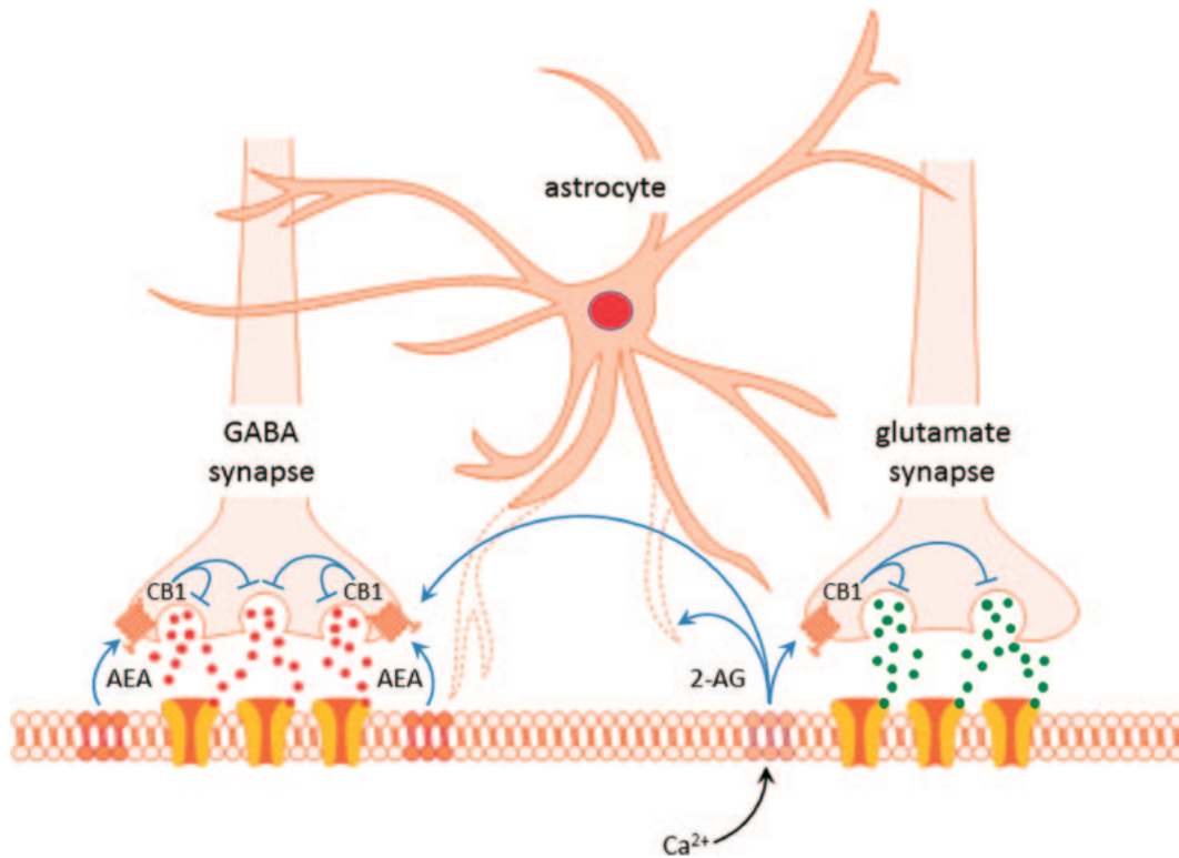
Fig. 5. Synapse-specific actions of endocannabinoids controlled by glial coverage of synapses. Tonic release of anandamide (AEA) provides a retrograde inhibitory tone on GABA release by activating CB1 receptors specifically at GABA synapses on magnocellular neurons. Release of 2-AG evoked by Ca-dependent signaling retrogradely suppresses glutamate release via CB1 receptor activation specifically at glutamatergic excitatory synapses. Physiological or pathological stimulation leads to retraction of astrocyte processes, which allows 2-AG spillover onto GABA synapses and further suppression of GABA release. Tonic AEA actions are not regulated by glial coverage and are limited to GABA synapses.
