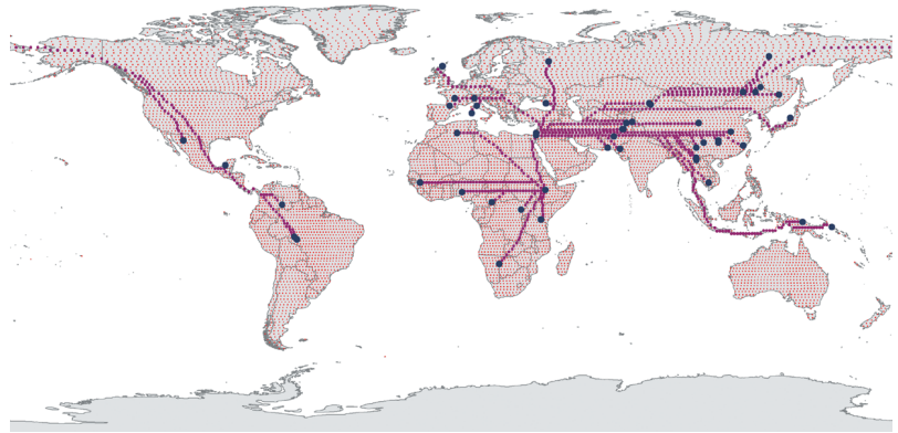
Figure 1. Shortest routes (in purple) through landmasses and specified land bridges between the 51 populations analysed (blue dots) and a hypothetical East African origin. Geographic distances have been computed as paths connecting vertices (in purple) on land with a newly developed algorithm based on graph theory (see Supplemental data).
