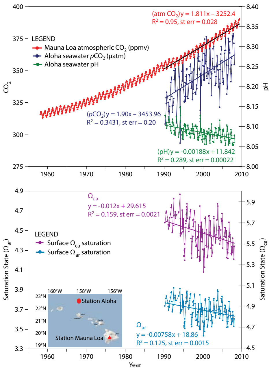
Figure 1. (Top) Time series of atmospheric CO 2 at Mauna Loa (ppmv) and surface ocean pH and pCO 2 (µatm) at Ocean Station Aloha in the subtropical North Pacific Ocean (see inset map). Note that the increase in oceanic CO 2 over the period of observations is consistent with the atmospheric increase within the statistical limits of the measurements. (Bottom) Calcite and aragonite saturation data for surface waters. Mauna Loa data: Pieter Tans, NOAA/ESRL, http://www.esrl.noaa.gov/gmd/ccgg/trends . HOT/ALOHA data: David Karl, University of Hawaii, http://hahana.soest.hawaii.edu . Updated from Doney et al. (2009). See also Dore et al. (2009).
