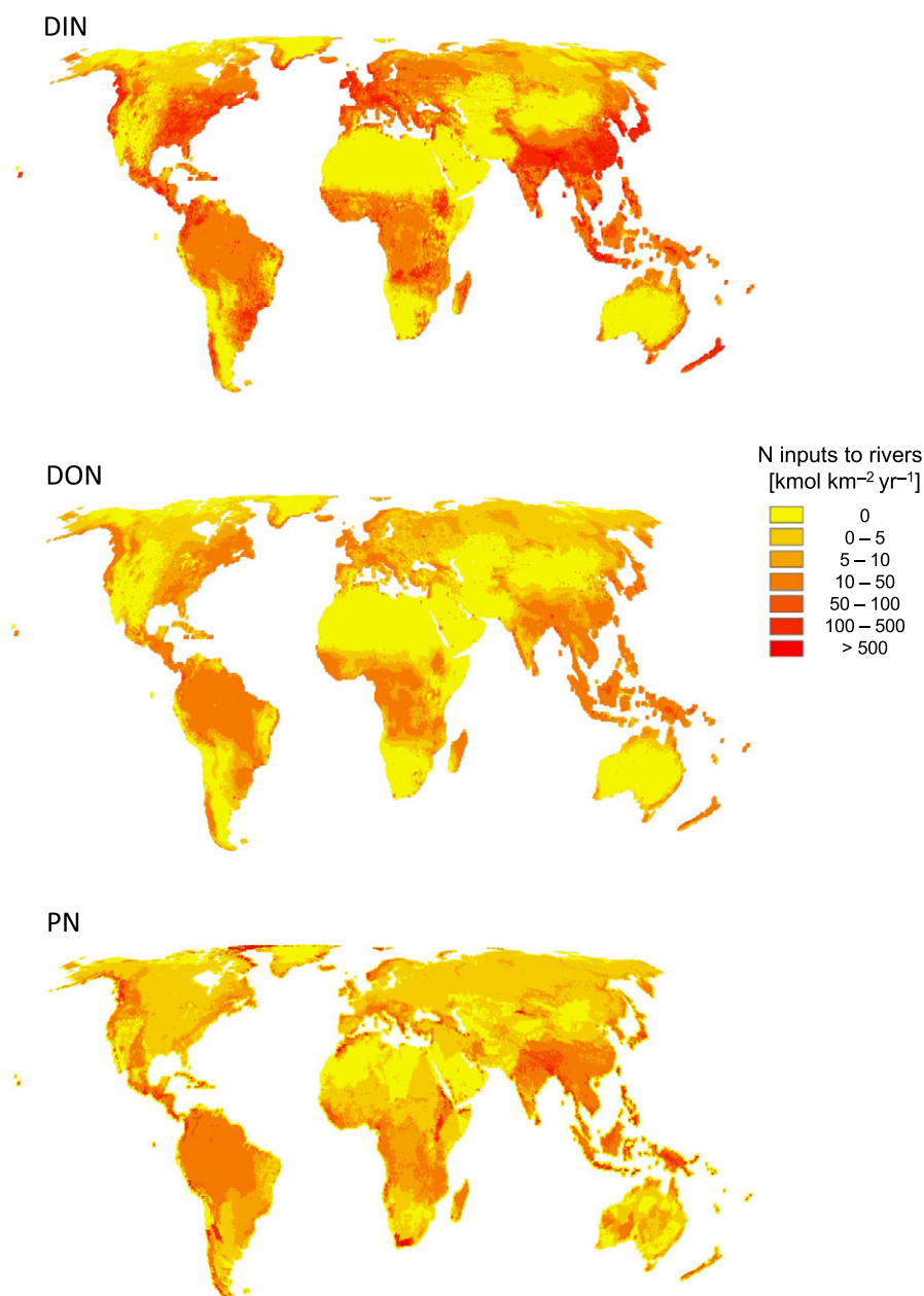
FIGURE 2 Mobilization of DIN, DON and PN to the river network as prescribed by Global-NEWS, after Van Drecht et al. (2009) and Bouwman et al. (2009), re-distributed at 0.5-degree resolution [Colour figure can be viewed at wileyonlinelibrary.com ]
