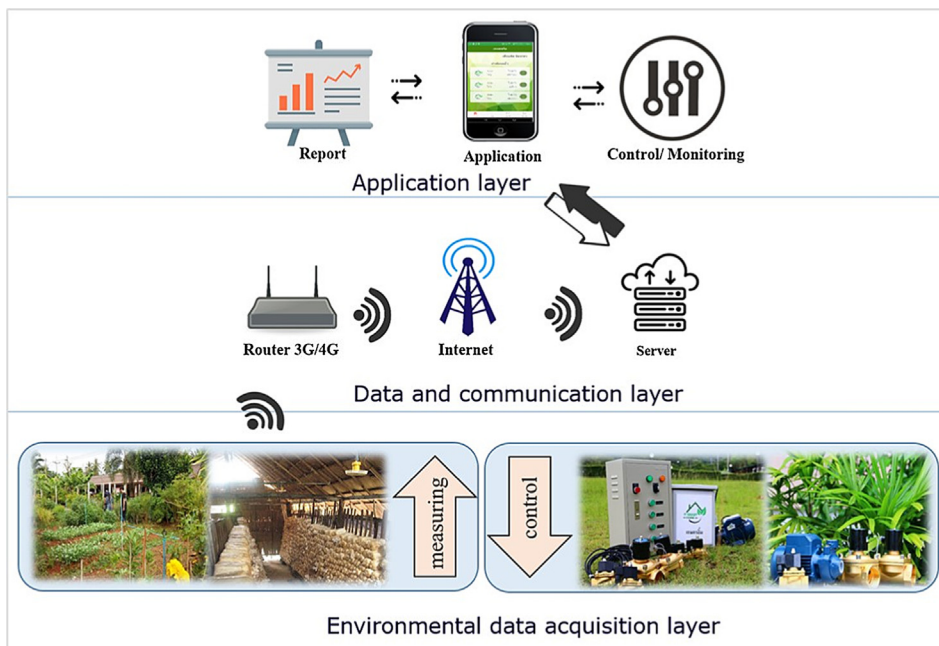
Fig. 6. The architecture of the control system.
