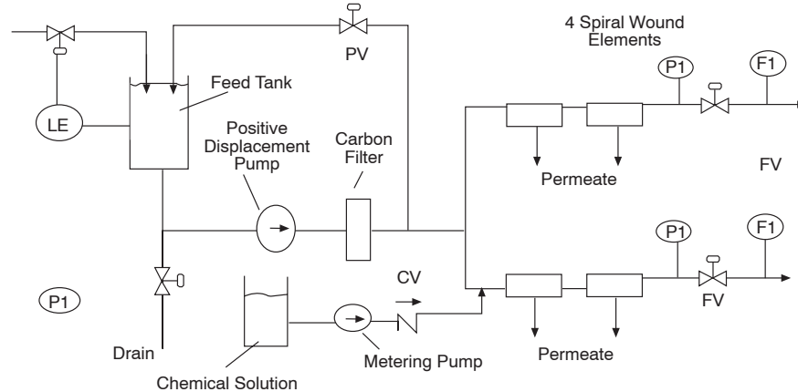
b. Element Test Unit
