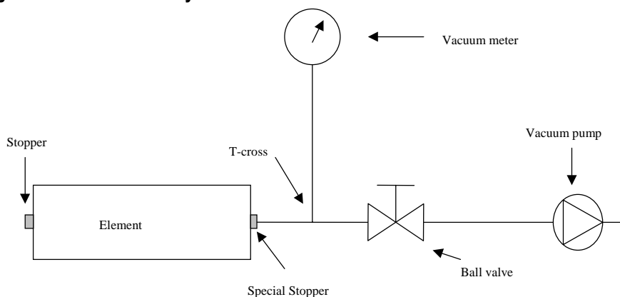
Figure 8.3 Vacuum decay test
