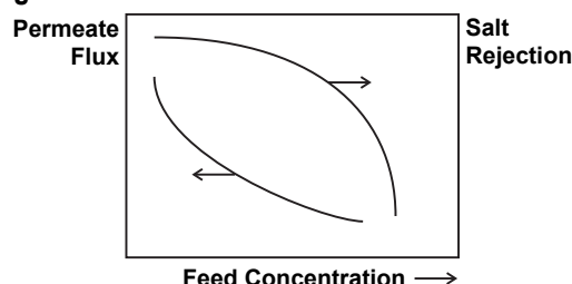
Figure 1.9 Performance vs. feedwater salt concentration
