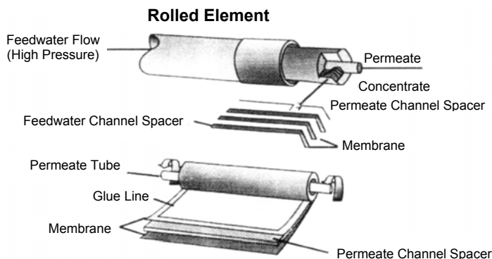
Figure 1.13 Construction of spiral wound FILMTEC RO membrane element
