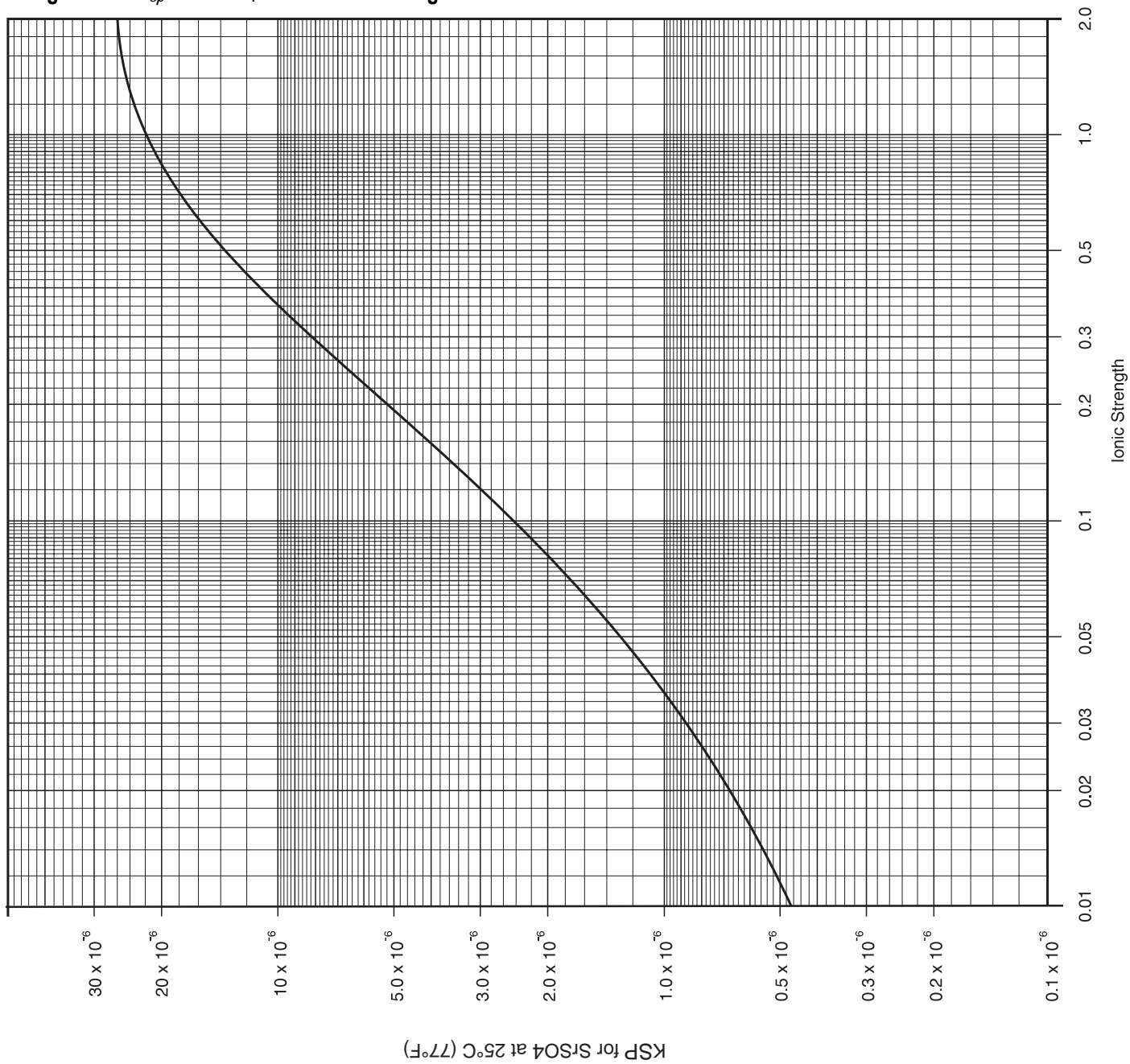
Figure 2.8 K_{sp} for SrSO_4 versus ionic strength /10/
