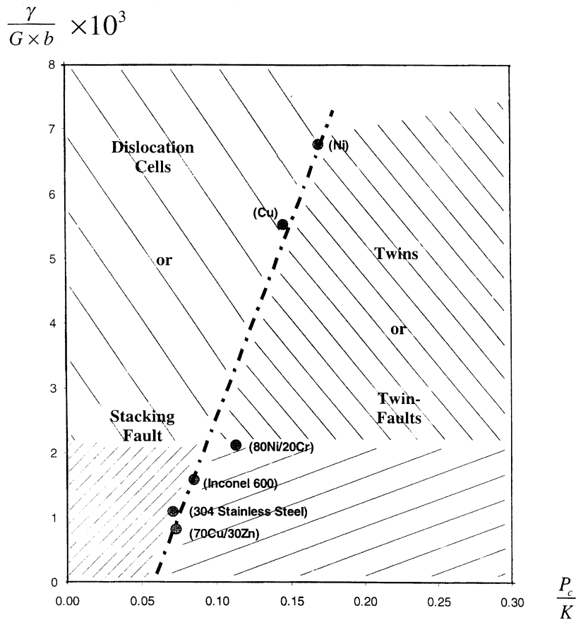
Fig. 22. Normalized pressure/stacking fault energy plot showing twinning and dislocation domains (adapted from Murr [90]).
