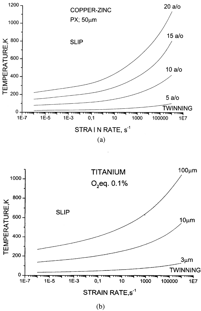
Fig. 9. (a) Calculated slip–twinning transition for polycrystal Cu–Zn brasses with grain size 50 µm; (b) calculated slip–twinning transition for titanium with different grain sizes.
