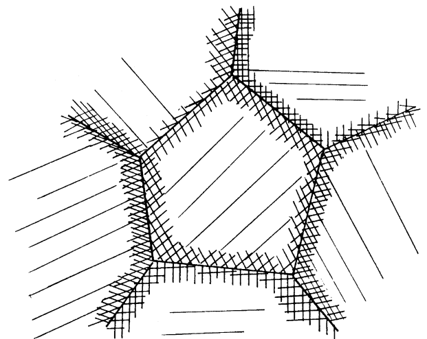
Fig. 12. Schematic configuration of slip in polycrystalline aggregate, at the first stage of plastic flow: notice activation of multiple slip in grain-boundary regions and single slip in grain interiors.
