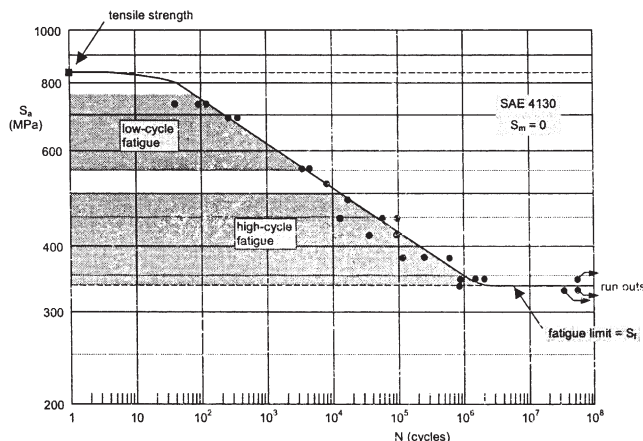
Fig. 11. Fatigue test results of unnotched specimens of a low alloy steel (NACA TN 2324, 1951). Regions of low-cycle and high-cycle fatigue.
