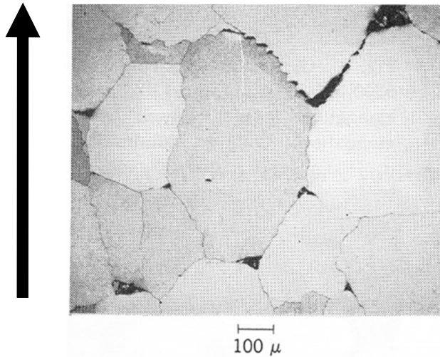
Fig. 8. Aluminum-20% zinc alloy tested in creep rupture at 500°F. Rupture life, 12 hr. Stress direction is vertical.
