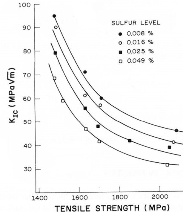
Figure 7.27 Variation of fracture toughness K_{Ic} with tensile strength and sulfur content in a steel. (Adapted with permission from A. J. Birkle, R. P. Wei, and G. E. Pellissier, Trans. ASM , 59 (1966) 981, p. 982)
