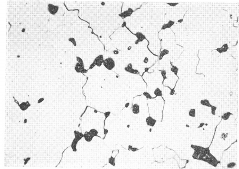
Fig. 12. Cavities in grain boundaries of chromium (27% extension at 3.2 \times 10^{-3} %/hr at 950°C). (After Wilms. 72 )
