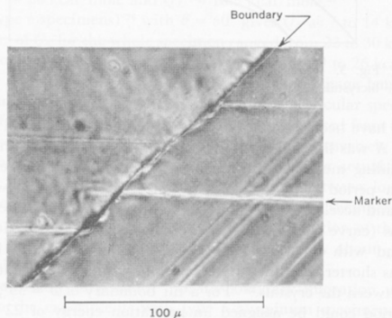
Fig. 2. Sliding at boundary of lead bicrystal. Phase contrast, unetched.
