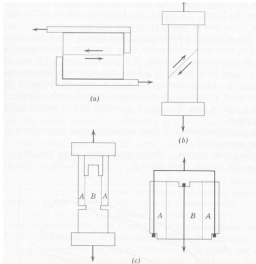
Fig. 1. Types of bicrystal used to study sliding.
