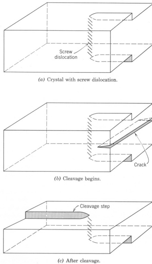
Fig. 4. Creation of cleavage step by screw dislocations.
