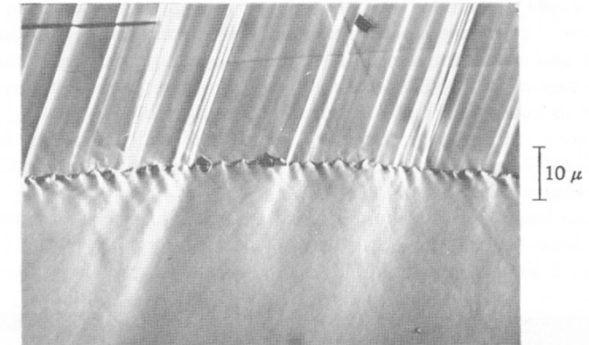
Fig. 9. Grain-boundary corrugations caused by creep at 400°F and 6800 psi in aluminum-1.9% magnesium alloy. Preliminary creep elongation, 9.4%, followed by repolishing and 10.2% additional elongation. Oblique illumination.
