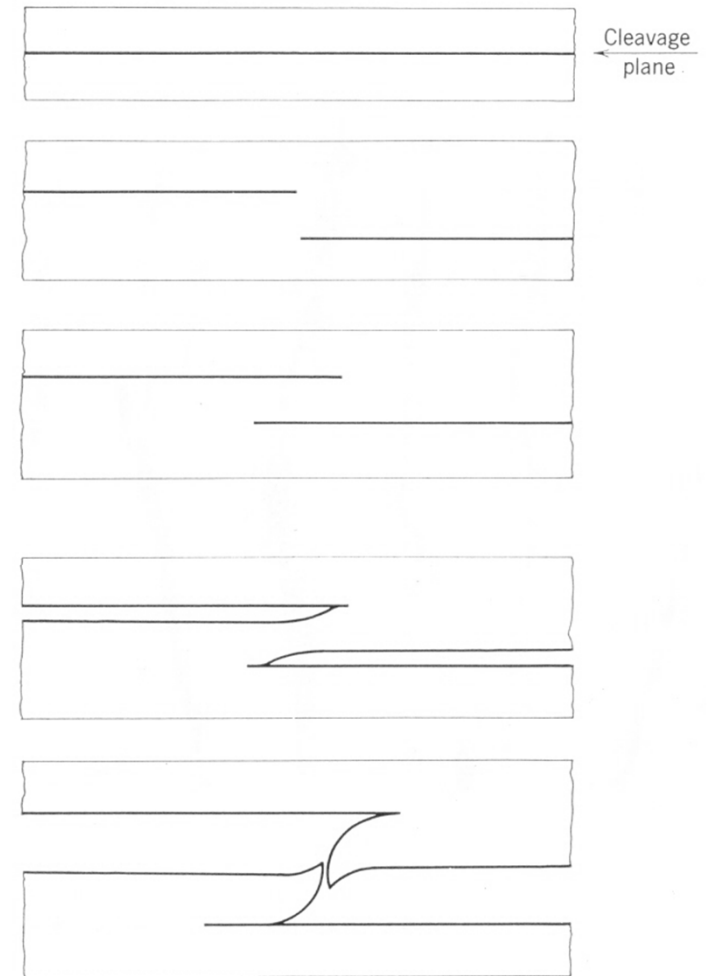
Fig. 2. Schematic representation of cleavage step formation between two parallel cleavage cracks on differing crystal planes. Ductile fracture shown is one mode of parting to form steps; for others, see Gilman 2 and Berry. 3
