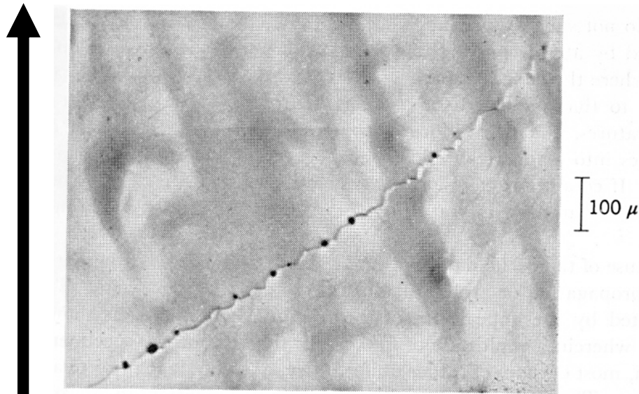
Fig. 11. Aluminum-2% magnesium alloy tested in creep rupture at 500°F and 4000 psi. Rupture life, 5 hr. Stress direction is vertical.
