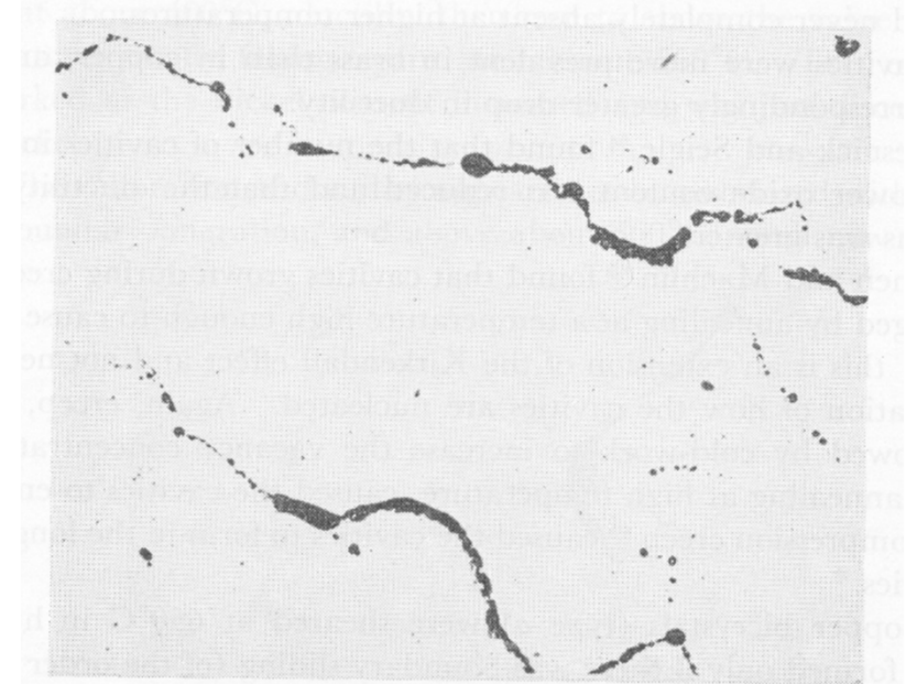
Fig. 9. Cavities in grain boundaries of copper (7% extension at 0.2%/hr at 300°C). (After Greenwood, Miller, and Suiter. 63 )
