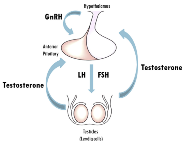
Fig. 1. Hypothalamic-pituitary-gonadal axis.
