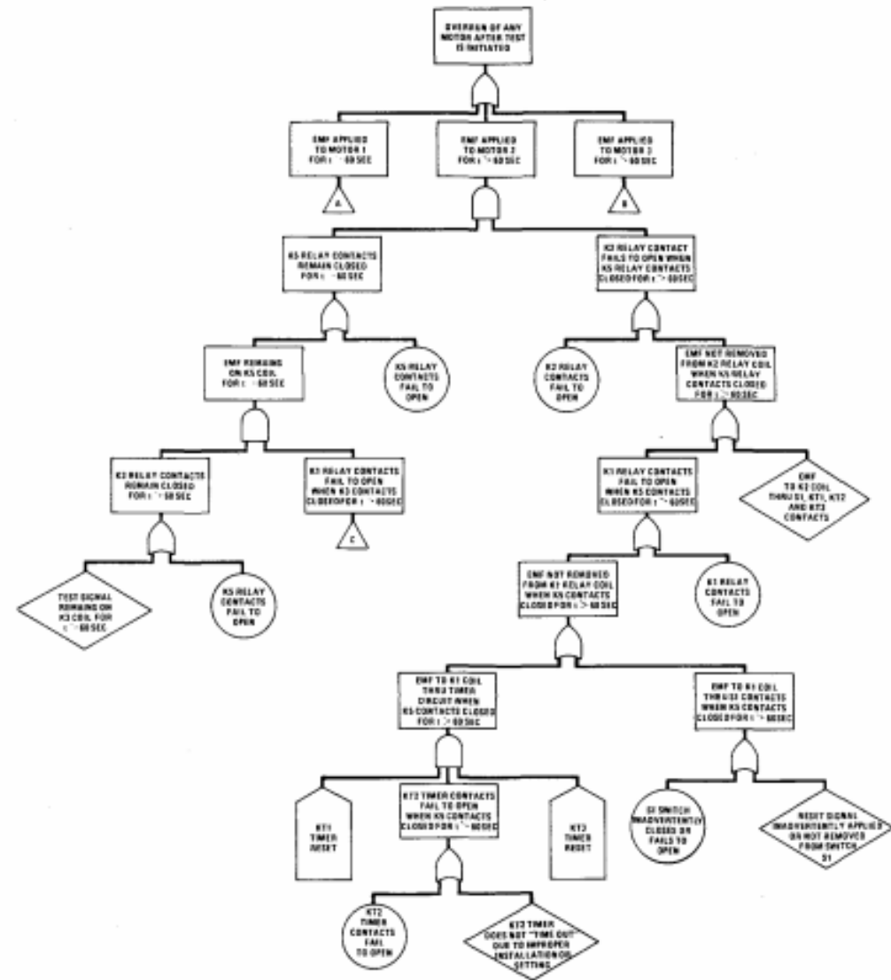
Figure IV-1. Typical Fault Tree
