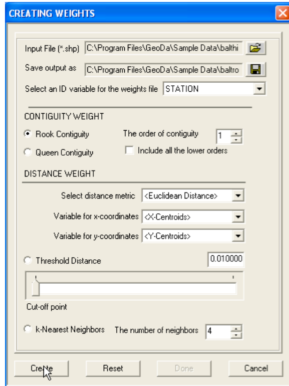
Figure 23.3: Rook contiguity weights for Baltimore Thiessen polygons.
