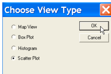
Figure 10.1: Conditional plot function.
