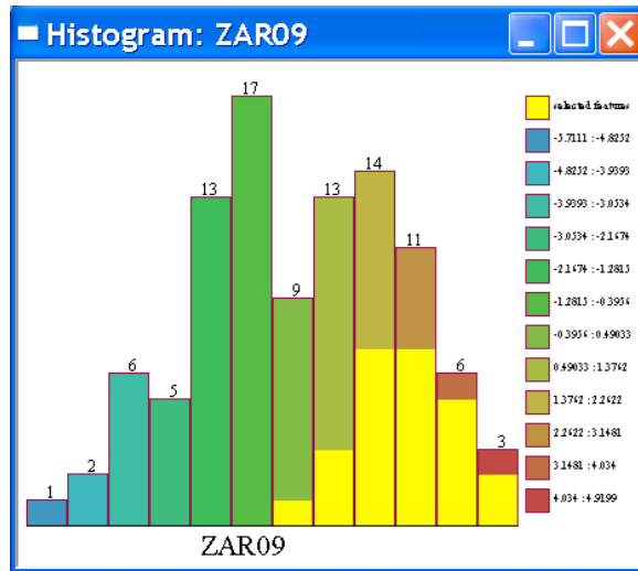
Figure 7.10: Histogram with 12 intervals.
