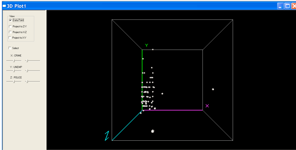
Figure 10.10: Three dimensional scatter plot (police, crime, unemp).
