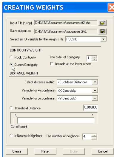
Figure 15.12: Queen contiguity.
