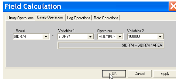
Figure 3.11: Rescaling the SIDS death rate.
