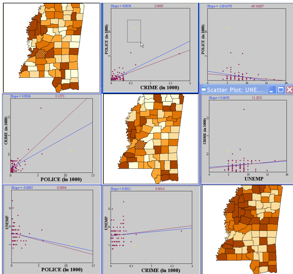
Figure 9.4: Brushing the scatter plot matrix.
