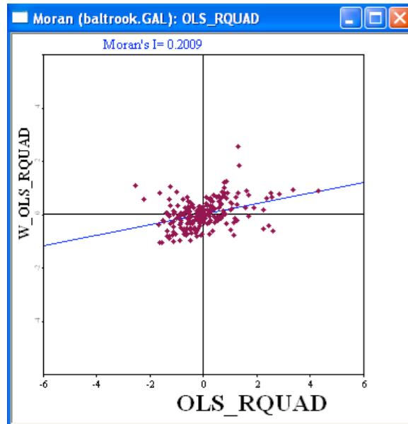
Figure 23.19: Moran scatter plot for quadratic trend surface residuals.
