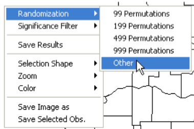
Figure 19.12: LISA randomization option.
