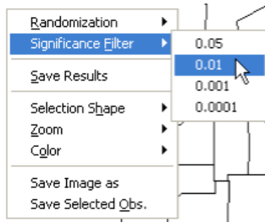
Figure 19.14: LISA significance filter option.
