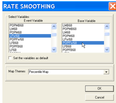
Figure 13.3: Selecting variables for event and base.
