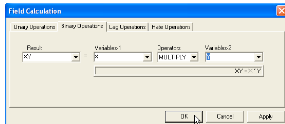
Figure 23.4: Calculation of trend surface variables.
