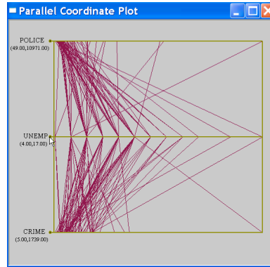
Figure 9.10: PCP with axes moved.
