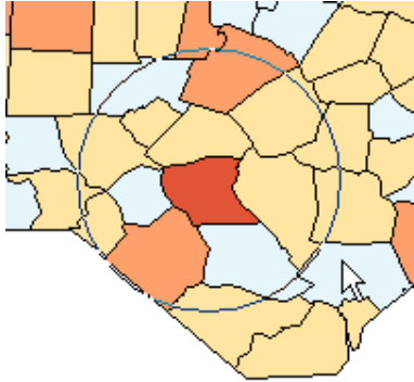
Figure 2.6: Circle selection.
