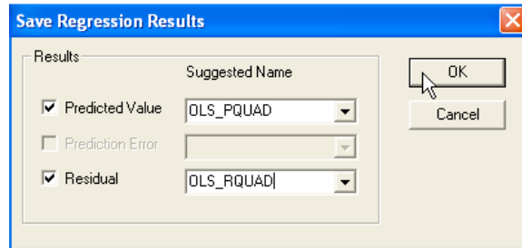
Figure 23.13: Quadratic trend surface residuals and predicted values.
