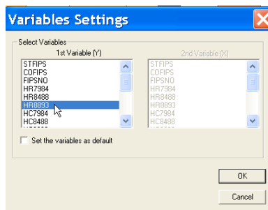
Figure 7.12: Box plot function.
