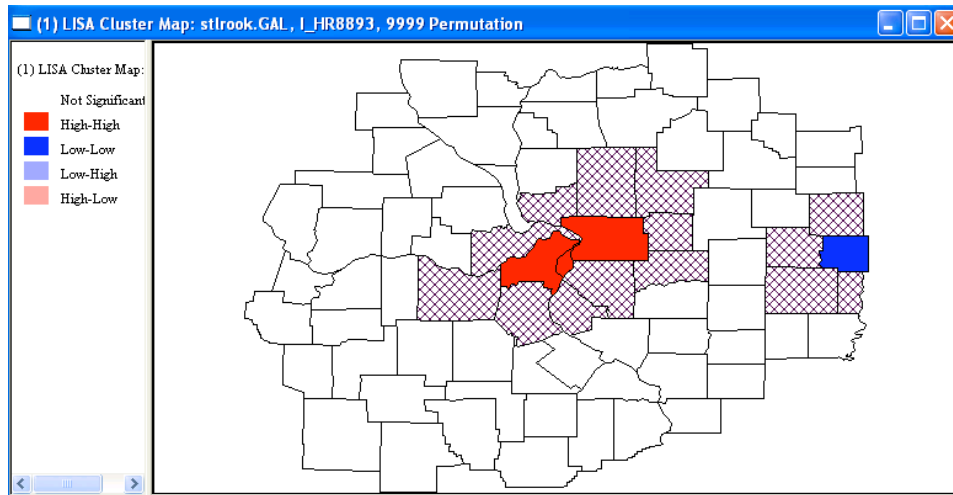
Figure 19.16: Spatial clusters.
