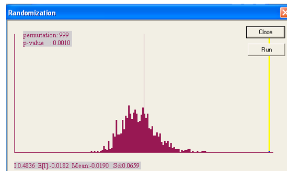
Figure 18.10: Randomization option dialog in Moran scatter plot.
