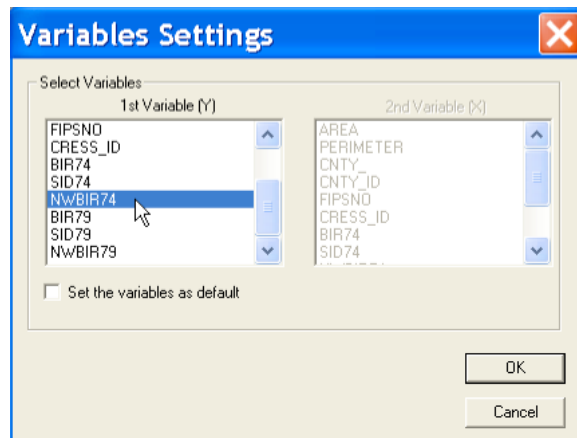
Figure 2.1: Variable selection.
