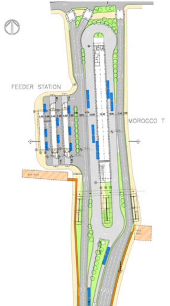
Fig. 11.95 In this proposed terminal in Dar es Salaam, the feeder platforms are slightly separated from the trunk platform. Image courtesy of the Dar es Salaam City Council
