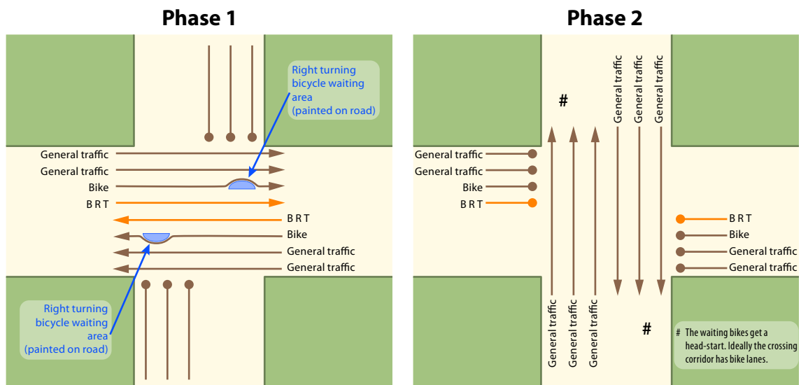
Fig. 9.27 A median cycleway and median busway can an effective solution to provide safe and efficient movements for both modes. In this case, a priority wait area for bicycles helps cyclists to get a head start over motorised vehicles in terms of negotiating a turn.
