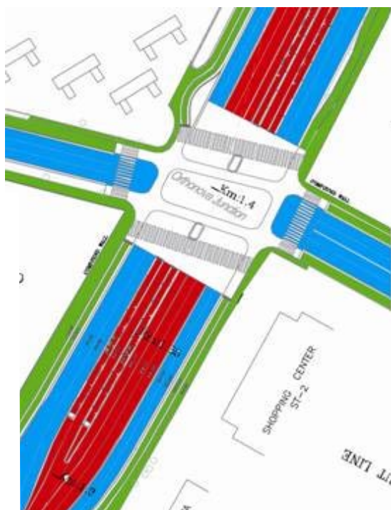
Fig. 9.47 Given the wide amount of right-of-way in this section of the Delhi BRT system, intersection section stations have been proposed in order to maximise pedestrian convenience.
