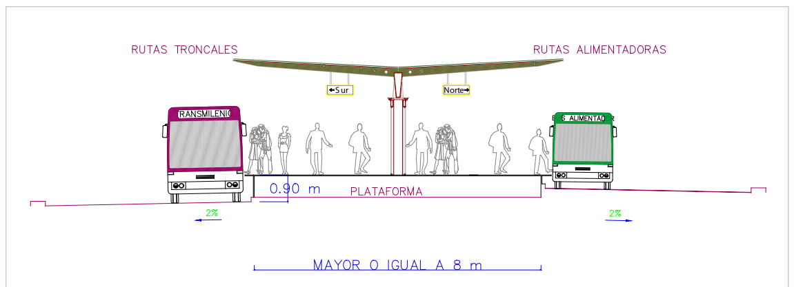
Fig. 11.94 Schematic showing the simple transfer from a trunk vehicle (on the left) to a feeder vehicle (on the right). Image courtesy of Steer Davies Gleave
