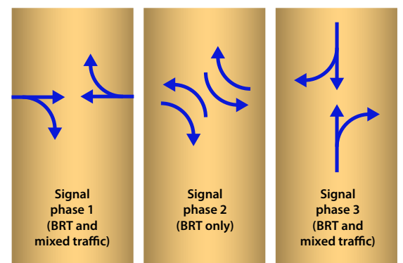
Fig. 9.32 In order to permit the BRT turning movements suggested in Figure 9.31, a three-phase traffic signal would be required.
