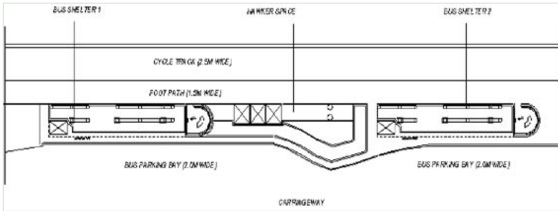
Fig. 11.77 Schematic of bus shelter with integrated space for vendor activity.
