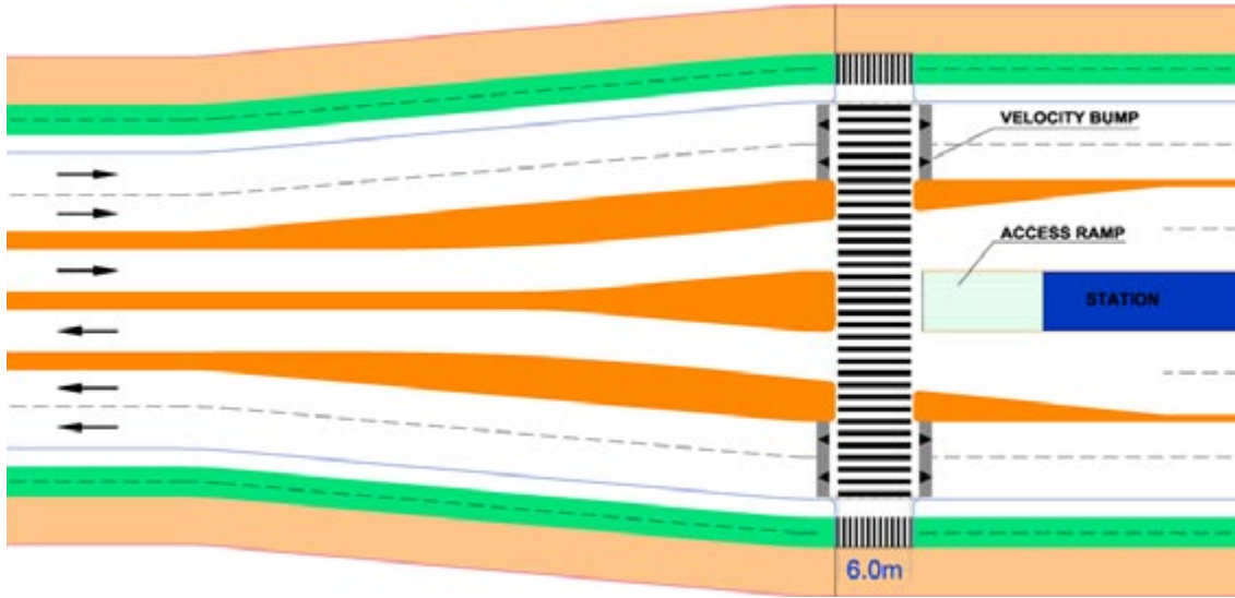
Fig. 13.57 When passing lanes are required at stations, it is recommended to include pedestrian islands between the busway and mixed traffic lanes.
