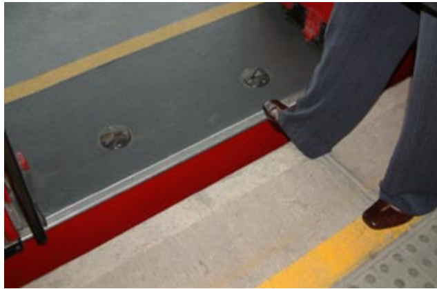
Fig. 8.25 If the vehicle can be aligned to the platform within 10 cm, then customers can safely board and alight with a gap entry.
