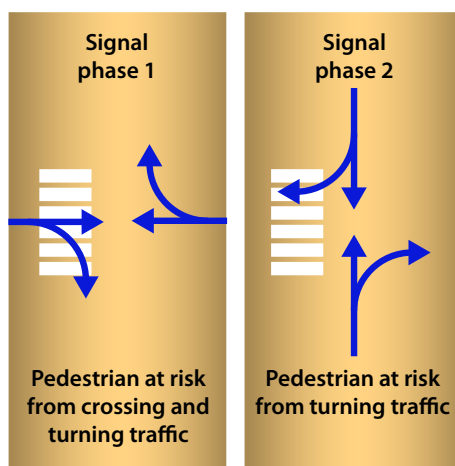
Fig. 9.21 In a standard two-phase traffic signal, pedestrians are potentially at risk during both phases.
