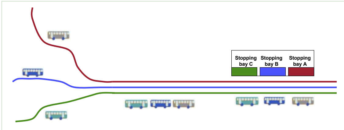
Fig. 8.39 Convoying systems work by permitting multiple routes to come together as a “train” of vehicles along a trunk corridor.
