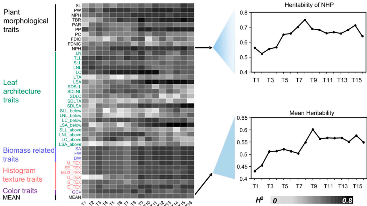
Figure 3. Phenotypic trait heritability during 16 growth stages. The heat map shows broad-sense heritability ( H^2 ) of the investigated phenotypic traits over 16 time points (left) as exemplified by the digital volume for natural plant height (top right) and for mean H^2 (bottom right). Trait identifiers are given as in the heat map and colored according to their classification as indicated: black, plant morphological traits; green, leaf architecture traits; blue, biomass-related traits; pink, histogram texture feature; purple, color trait. MEAN, H^2 of the mean value for all traits.
