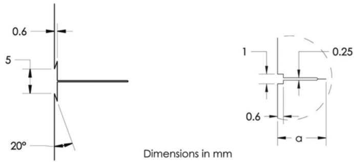
Square notch configuration for ring-type CMOD gage
