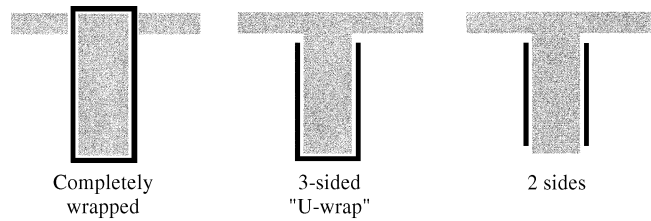
Fig. 11.1—Typical wrapping schemes for shear strengthening using FRP laminates.
