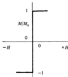
Fig. 7.18 Idealized hysteresis loop of a crystal measured parallel to an easy axis.
