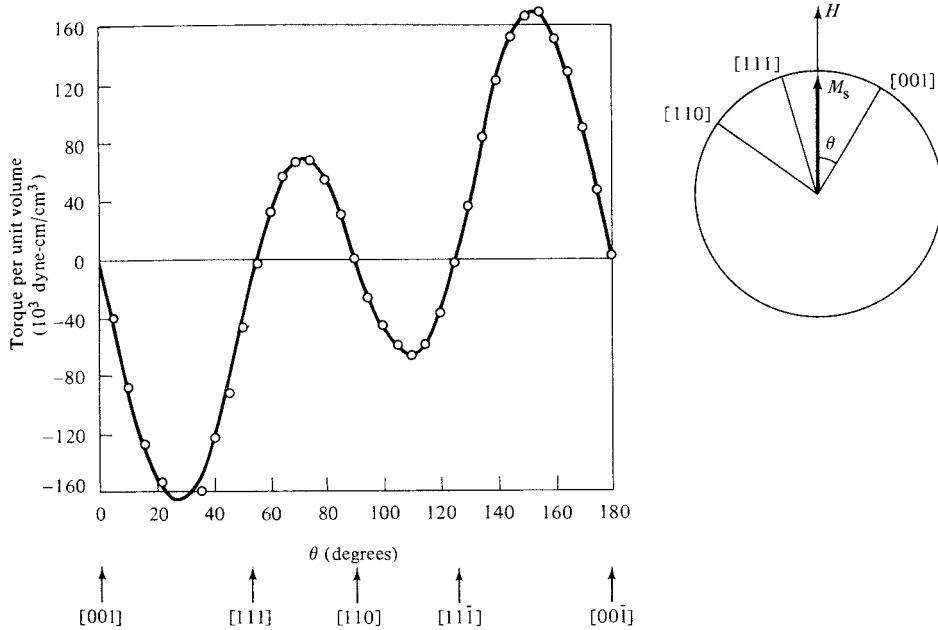
Fig. 7.15 Measured torque of a \{011\} disk of an Fe + 3.85 wt% Si alloy. The fitted curve is drawn for K_1 = 2.87 \times 10^5 erg/cm 3 and K_2 = 1 \times 10^5 erg/cm 3 . [R. M. Bozorth, Ferromagnetism , reprinted by IEEE Press (1993).]
