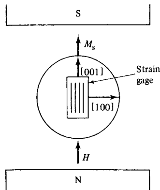
Fig. 8.4 Magnetostriction measurement on a single crystal using a strain gage.
