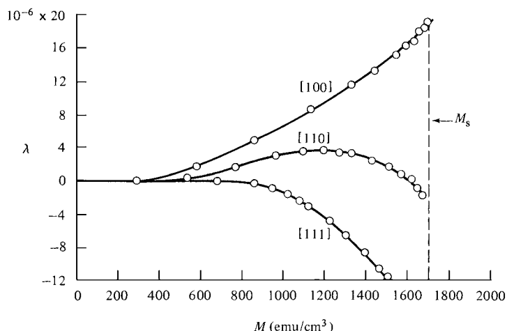
Fig. 8.5 Magnetostriction as a function of magnetization in single crystal iron rods. Each rod had a different crystallographic axis. [W. L. Webster, Proc. R. Soc. , A109 (1925) p. 570.]
