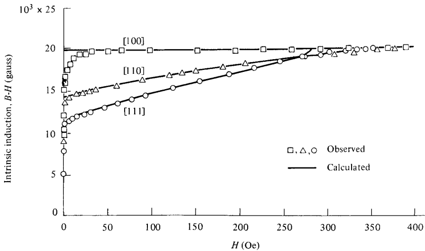
Fig. 7.22 Calculated and measured magnetization curves for Fe–Si crystals. [R. M. Bozorth, Ferromagnetism , reprinted by IEEE Press (1993).]
