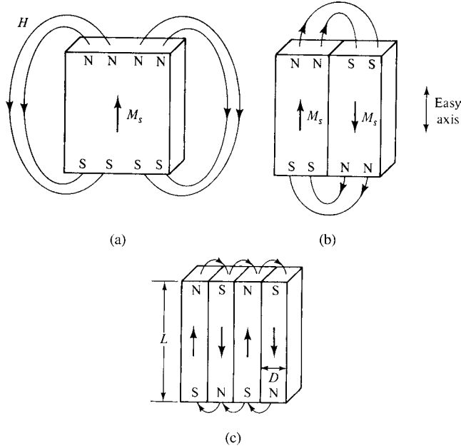
Fig. 9.16 Division of a crystal into domains. Only external H fields are shown.
