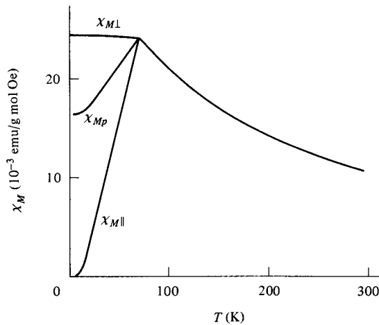
Fig. 5.9 Temperature variation of the molar susceptibility of MnF 2 . The central curve (below T_N ) is for a powder sample, and the other two curves are for a single crystal. [H. Bizette and B. Tai, Compt. Rend. , 238 (1954) p. 1575.]
