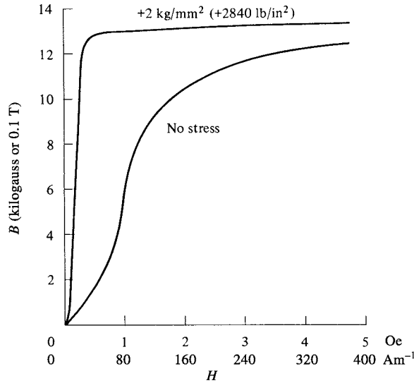
Fig. 8.17 Effect of applied tensile stress on the magnetization curve of 68 permalloy. [R. M. Bozorth, Ferromagnetism , reprinted by IEEE Press (1993).]
