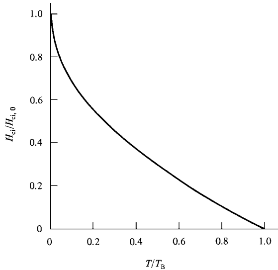
Fig. 11.21 Theoretical temperature dependence of the coercivity of single-domain fine particles. T_B = blocking temperature.
