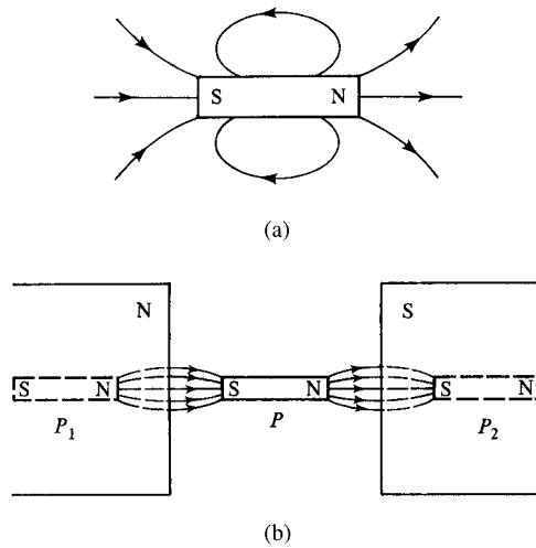
Fig. 2.40 Image effect. (a) field due to magnetized sample in empty space; (b) field due to magnetized sample placed between two soft iron pole pieces.
