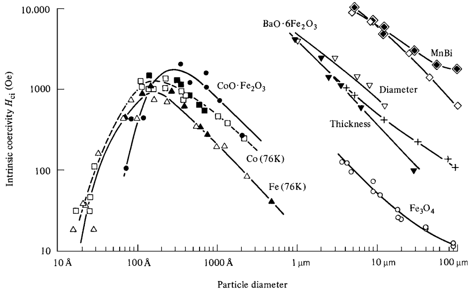
Fig. 11.1 Variation of coercivity with particle size, for particles whose coercivity depends on crystal anisotropy. [F. E. Luborsky, J. Appl. Phys. , 32 (1961) p. 171S.]
