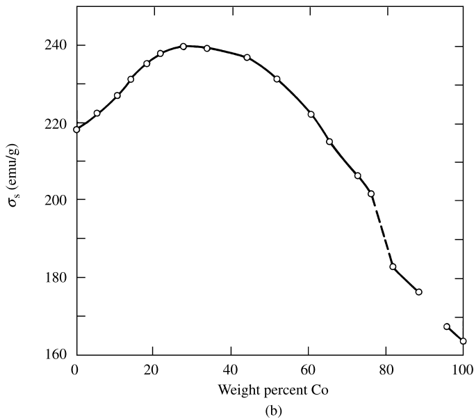
Fig. 4.21 (a) Fe-Co binary phase diagram. (b) Variation of \sigma_s at room temperature with composition.
