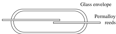
Fig. 13.23 Reed relay.
