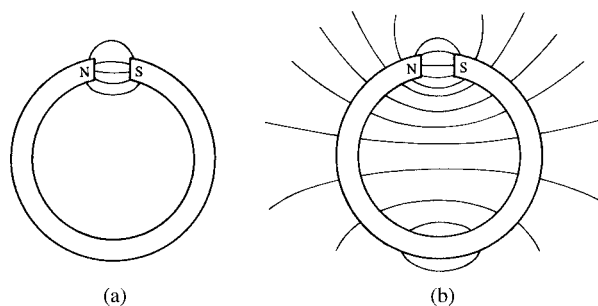
Fig. 14.5 Ring magnet showing (a) fringing and (b) leakage flux.
