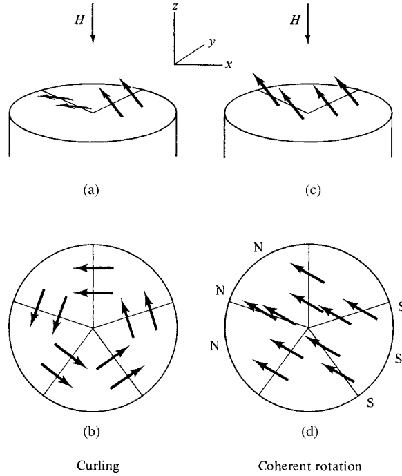
Fig. 11.8 (a) and (c) are curling and coherent-rotation modes. (b) and (d) are cross sections normal to the z axis after a 90^\circ rotation from the +z direction.
