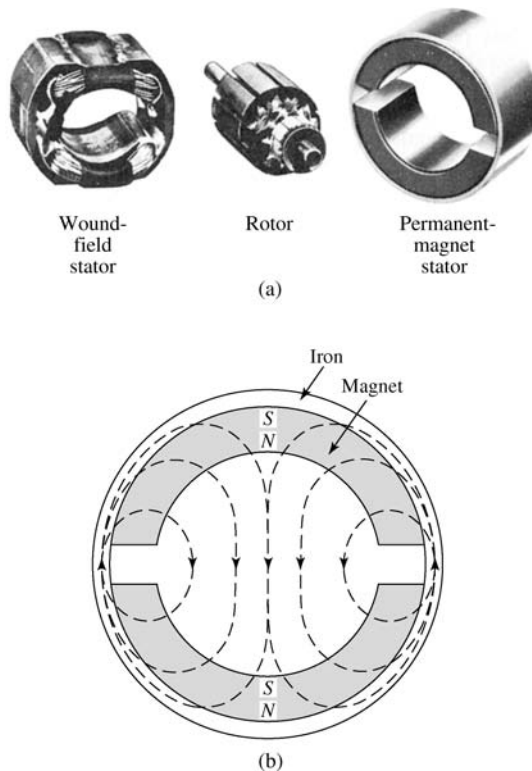
Fig. 14.18 Permanent magnet motor. (a) Comparison of a wound-field stator with a permanent magnet stator, with the same rotor; (b) the construction of the permanent magnet stator.
