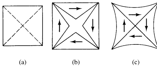
Fig. 8.11 Strains in a demagnetized single crystal.
