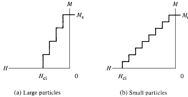
Fig. 11.17 Demagnetization curves of assemblies of particles.
