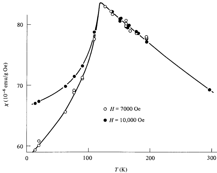
Fig. 5.8 Temperature variation of the susceptibility of MnO powder. [H. Bizette, C. F. Squire, and B. Tai, Compt. Rend. , 207 (1938) p. 449.]
