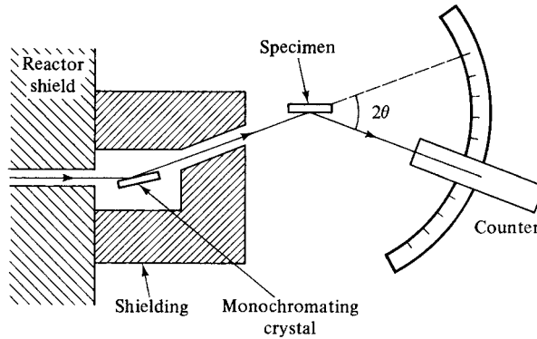
Fig. 5.13 Neutron diffractometer (schematic).
