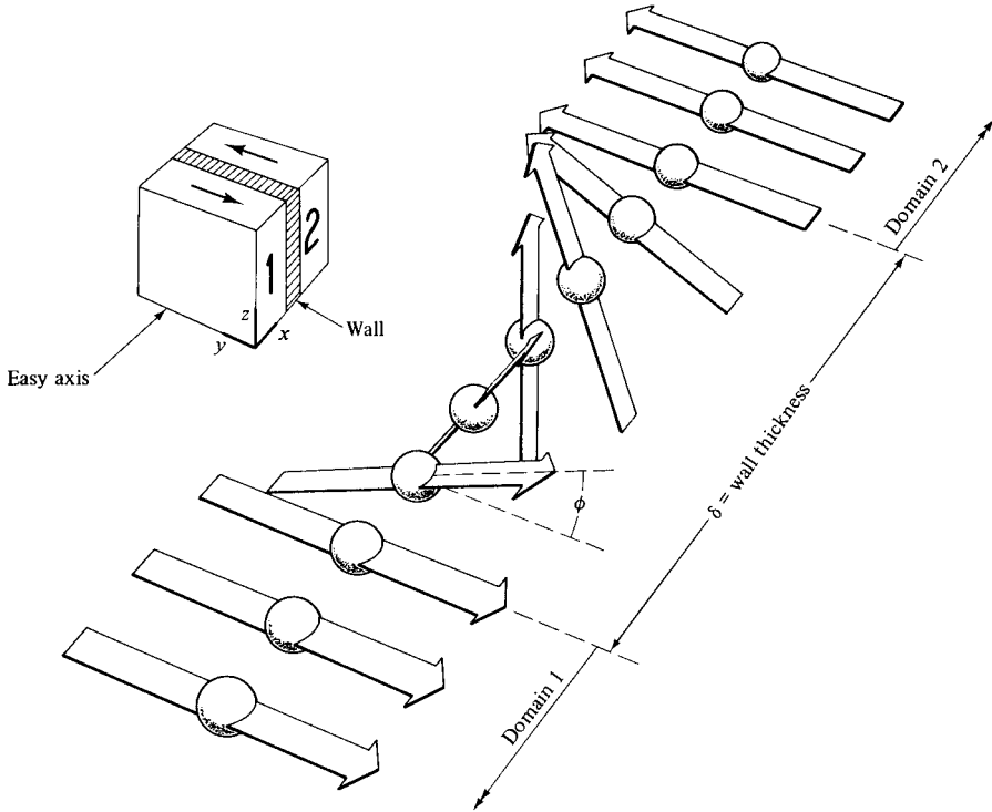
Fig. 9.2 Structure of a 180° domain wall.
