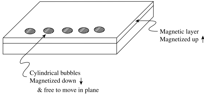
Fig. 15.9 Magnetic bubbles.
