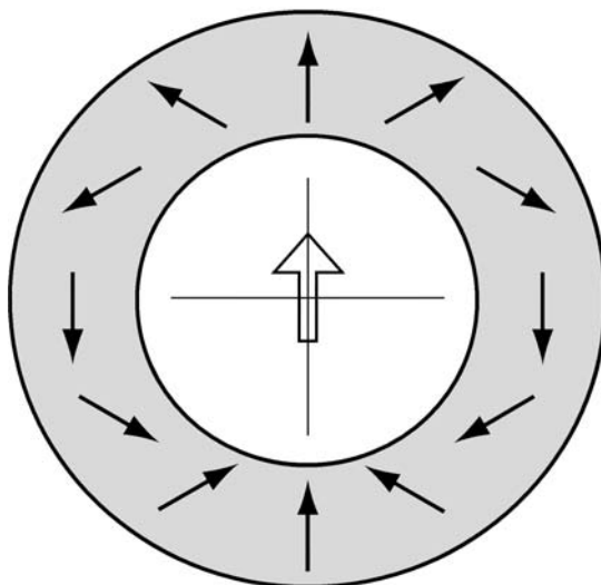
Fig. 2.12 Halbach cylinder. Solid arrows show direction of local magnetization. The open arrow is the resulting field.
