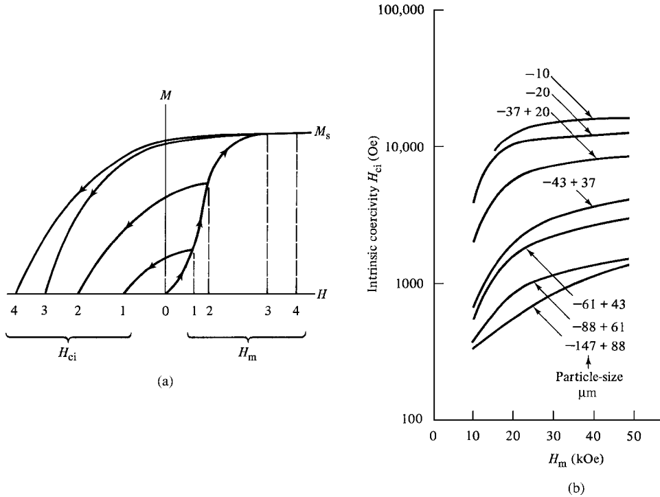
Fig. 11.15 Dependence of coercivity on maximum value H_m of magnetizing field. (a) Schematic. (b) Experimental results on aligned particles of \text{SmCo}_5 . [J. J. Becker, J. Appl. Phys. , 39 (1968) p. 1270.]
