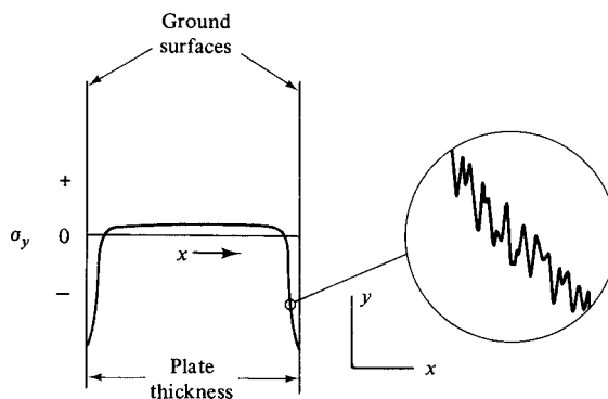
Fig. 9.30 Residual stress distribution due to grinding.
