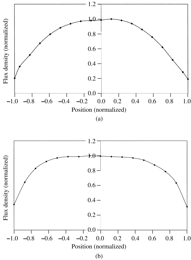
Fig. 2.23 (a) Measured flux density vs position in a steel bar magnet. (b) Same for an alnico bar magnet. The two magnets had similar length/area ratios.
