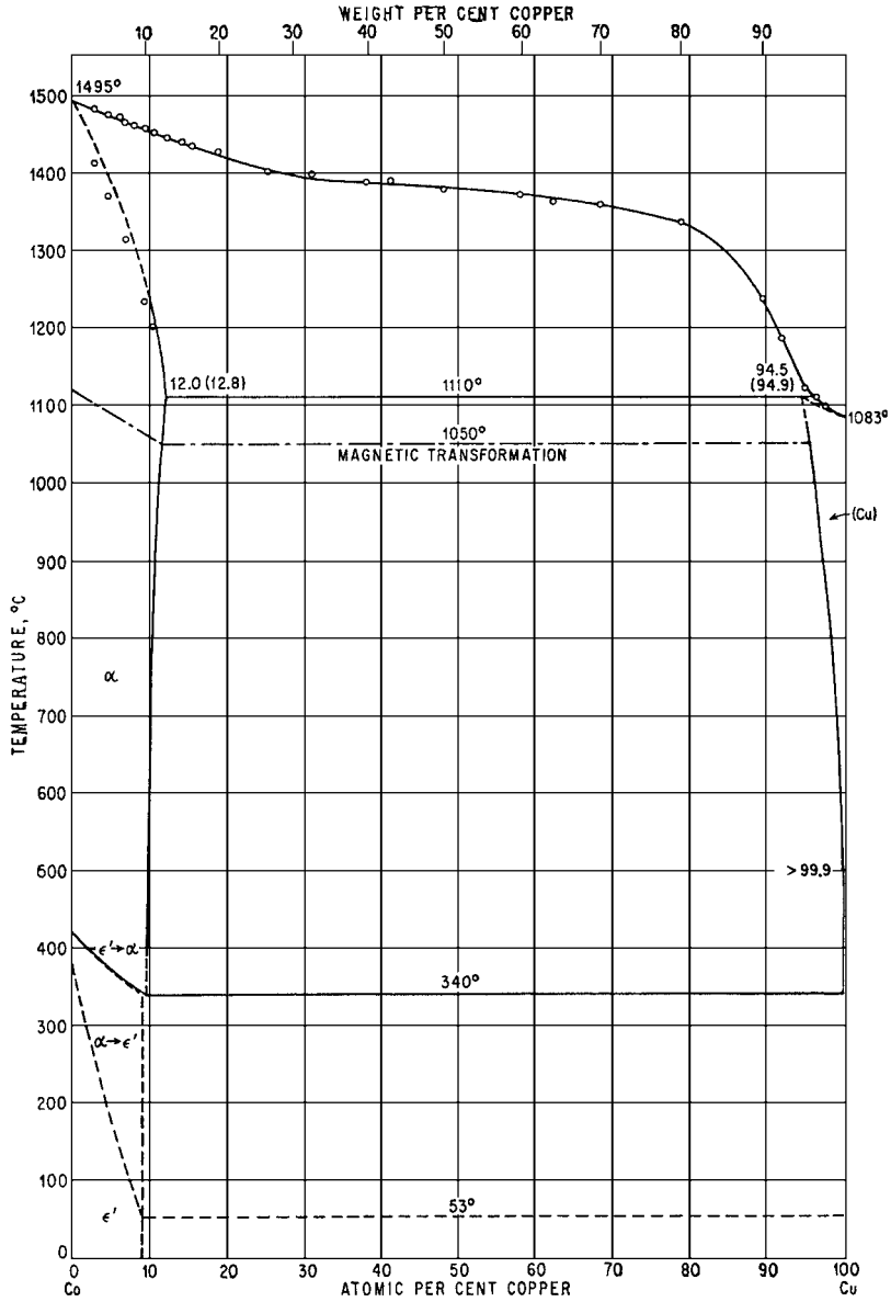
Fig. 11.22 Copper-cobalt equilibrium diagram ( ASM Handbook ).
