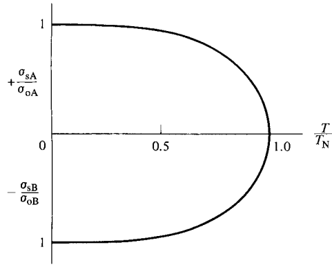
Fig. 5.4 Spontaneous magnetizations of the A and B sublattices at temperatures below T_N (schematic).
