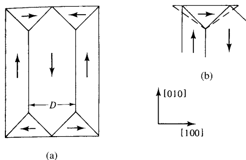
Fig. 9.18 Closure domains in a cubic crystal with \langle 100 \rangle easy axes.
