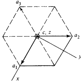
Fig. 8.8 Hexagonal and orthogonal axes in a hexagonal crystal.
