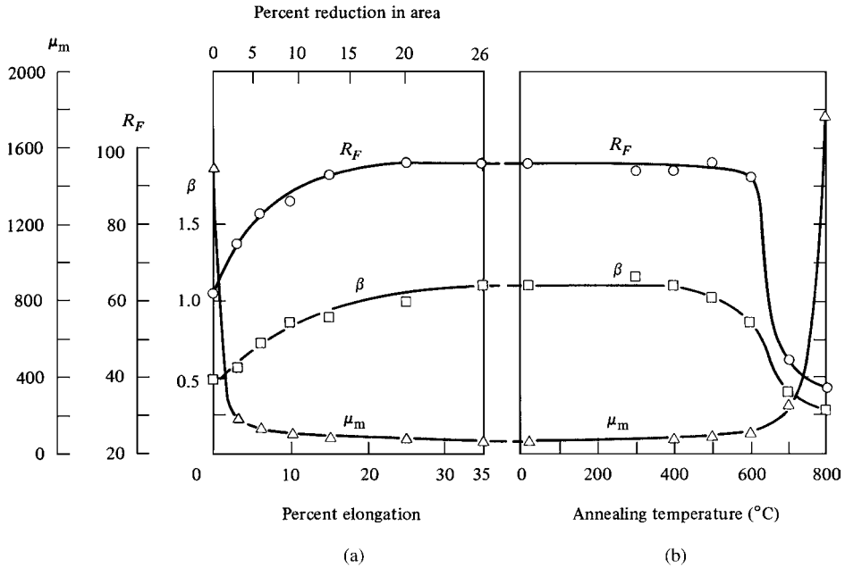
Fig. 9.46 Changes in physical properties of nickel during tensile deformation and subsequent annealing. R_F = hardness on Rockwell F scale; \beta = width (degrees) of the (420) X-ray line, using Cu K_{\alpha 1} radiation; \mu_m = maximum permeability. [H. Chou and B. D. Cullity, unpublished.]
