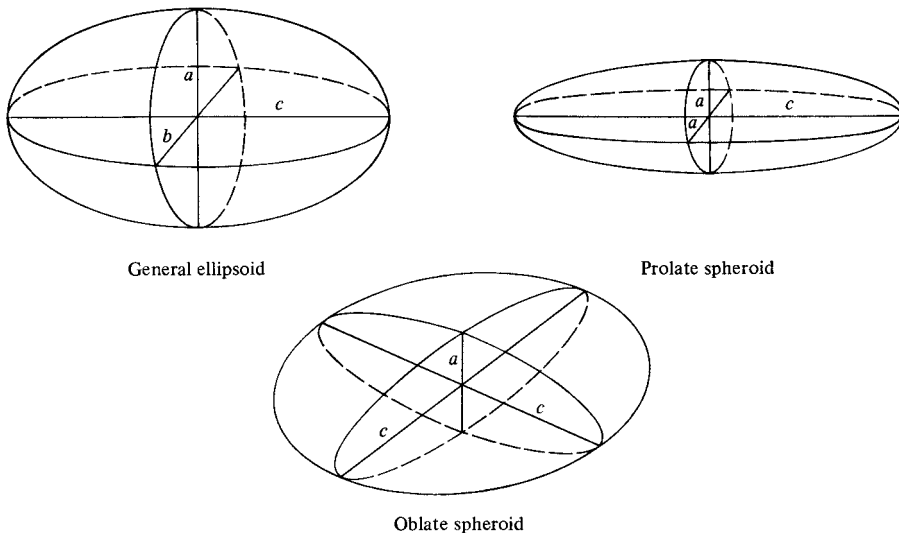
Fig. 2.27 Ellipsoids.
