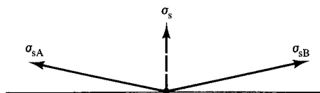
Fig. 5.18 Canted spins.
