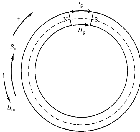
Fig. 14.2 Open magnetic circuit.
