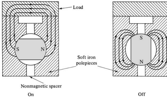
Fig. 14.20 Permanent magnet chuck.
