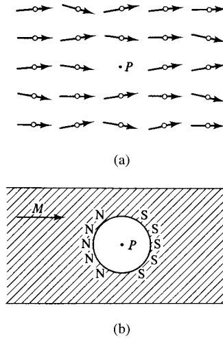
Fig. 4.12 Field at an interior point due to surrounding magnetized material.
