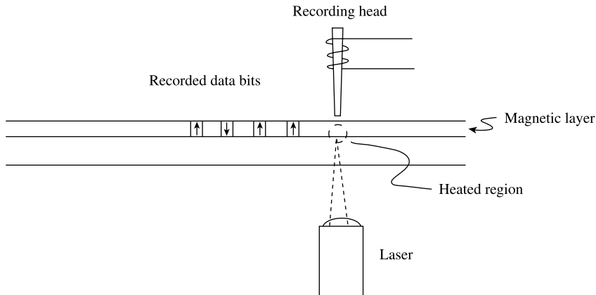
Fig. 15.8 Magneto-optic recording.
