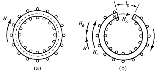
Fig. 2.42 Magnetic circuits. (a) closed, (b) open.
