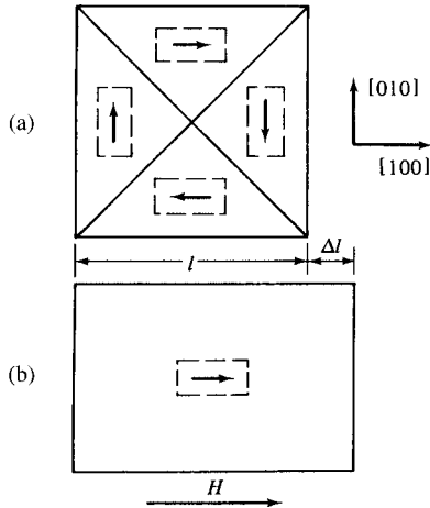
Fig. 8.2 Magnetostriction of an iron crystal in the [100] direction.
