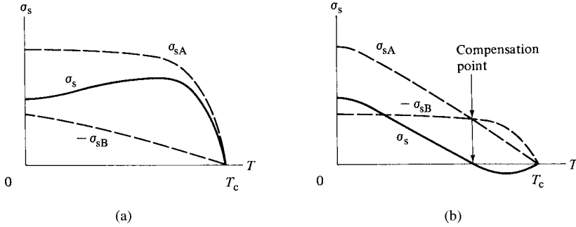
Fig. 6.9 Unusual \sigma_s vs T curves for cubic ferrimagnets.
