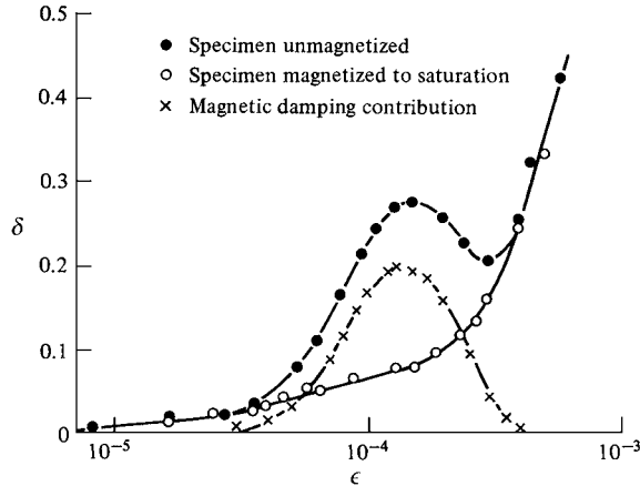
Fig. 12.17 Damping \delta (logarithmic decrement) as a function of maximum shear strain amplitude \epsilon at the surface of polycrystalline nickel at -40^\circ\text{C} . Torsion pendulum measurements at about 1 Hz [J. T. A. Roberts and P. Barrant, Acta. Metallurg. 15 (1967) p. 1685.]
