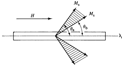
Fig. 8.24 Partial magnetization.
