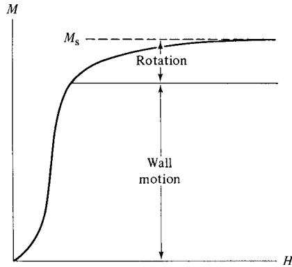
Fig. 9.25 Magnetization processes.
