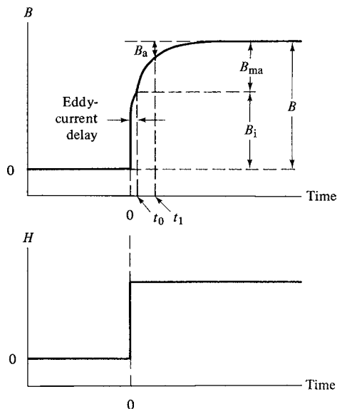
Fig. 12.13 Magnetic after-effect.
