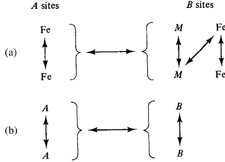
Fig. 6.5 Exchange interactions between ions in an inverse cubic ferrite.
