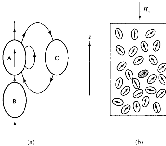
Fig. 11.4 Particle interactions.
