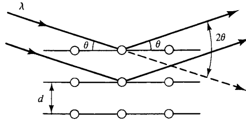
Fig. 5.10 Diffraction geometry.
