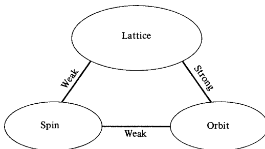
Fig. 7.8 Spin–lattice–orbit interactions.
