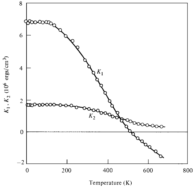
Fig. 7.25 Temperature dependence of anisotropy constants of cobalt [Y. Barrier, R. Pauthenet, and G. Rimet, Cobalt , 15 (1962) p. 1].
