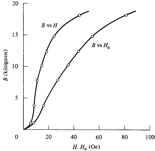
Fig. 2.34 Measured and corrected magnetization curves of cold-worked iron, from the data of Table 2.2.
