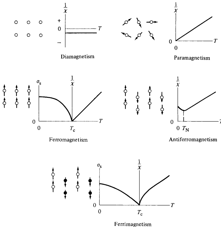
Fig. 6.14 Kinds of magnetism.
