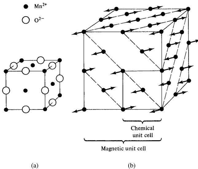
Fig. 5.16 Structure of MnO . (a) Chemical unit cell of Mn and O ions. (b) Chemical and magnetic units cells, Mn ions only.
