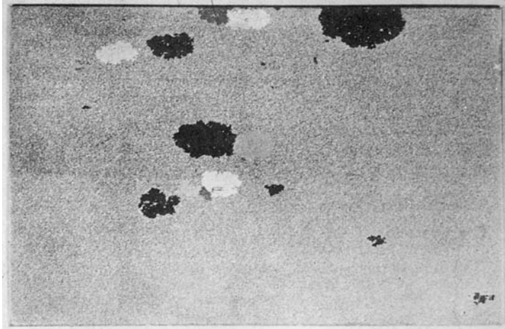
Fig. 13.13 Partial secondary recrystallization in silicon iron. A few large secondary grains are growing in a matrix of primary grains during a 900°C anneal. About actual size. [C. G. Dunn, Cold Working of Metals , ASM (1949) p. 113.]
