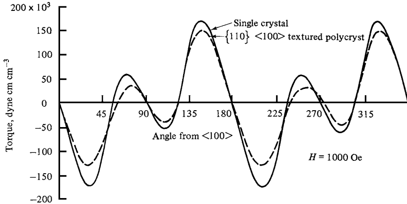
Fig. 13.15 Torque curves of a single crystal in the \{110\} plane and of a disk cut from a sheet of grain-oriented silicon steel having a strong cube-on-edge, \{110\} \langle 100 \rangle texture. [C. D. Graham, Magnetism and Metallurgy , Volume 2, Academic Press (1969).]
