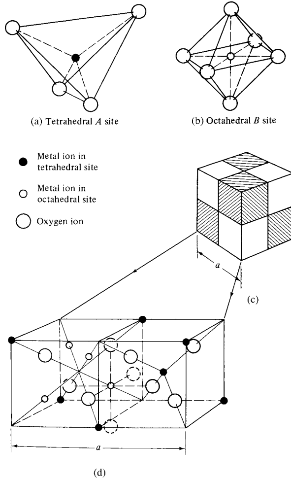
Fig. 6.2 Crystal structure of a cubic ferrite.
