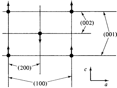
Fig. 5.15 Projection of the MnF_2 unit cell on a (010) face. Only the Mn ions are shown.
