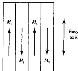
Fig. 7.6 Domain structure of a uniaxial crystal.
