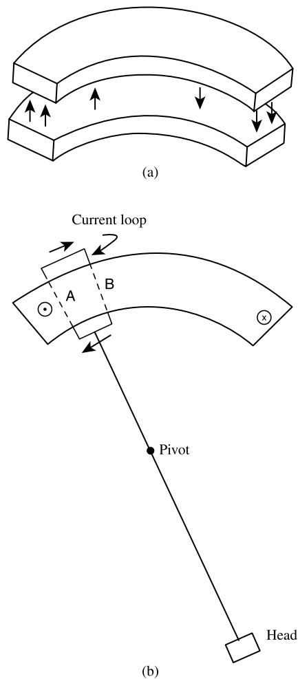
Fig. 14.19 Hard drive head positioner. (a) Magnet configuration; (b) current loop in magnet field, with head at the other end of the pivoted arm.
