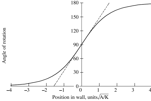
Fig. 9.3 Variation of magnetization direction through a 180° domain wall. Dashed line shows definition of wall width.
