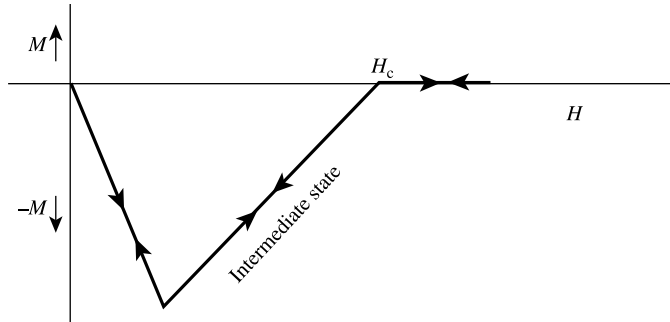
Fig. 16.2 Magnetic behavior of an ideal type I superconductor with nonzero demagnetizing factor N .
