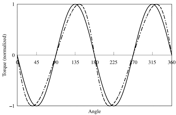
Fig. 7.12 Variation of torque with angle \psi between easy axis c and field H for a uniaxial crystal. The dashed curve is for H = 2K_1/M_s ; solid curve for H \gg 2K_1/M_s .
