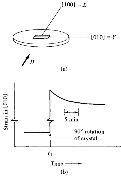
Fig. 10.10 Experiment to determine the preferred interstitial sites in iron. [After DeVries et al. Physica , 25 (1959) p. 1131.]
