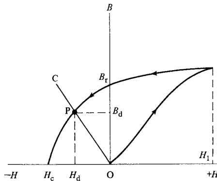
Fig. 14.1 Initial magnetization and demagnetization curve of a permanent magnet. B_r is the residual induction; point P is the operating point.
