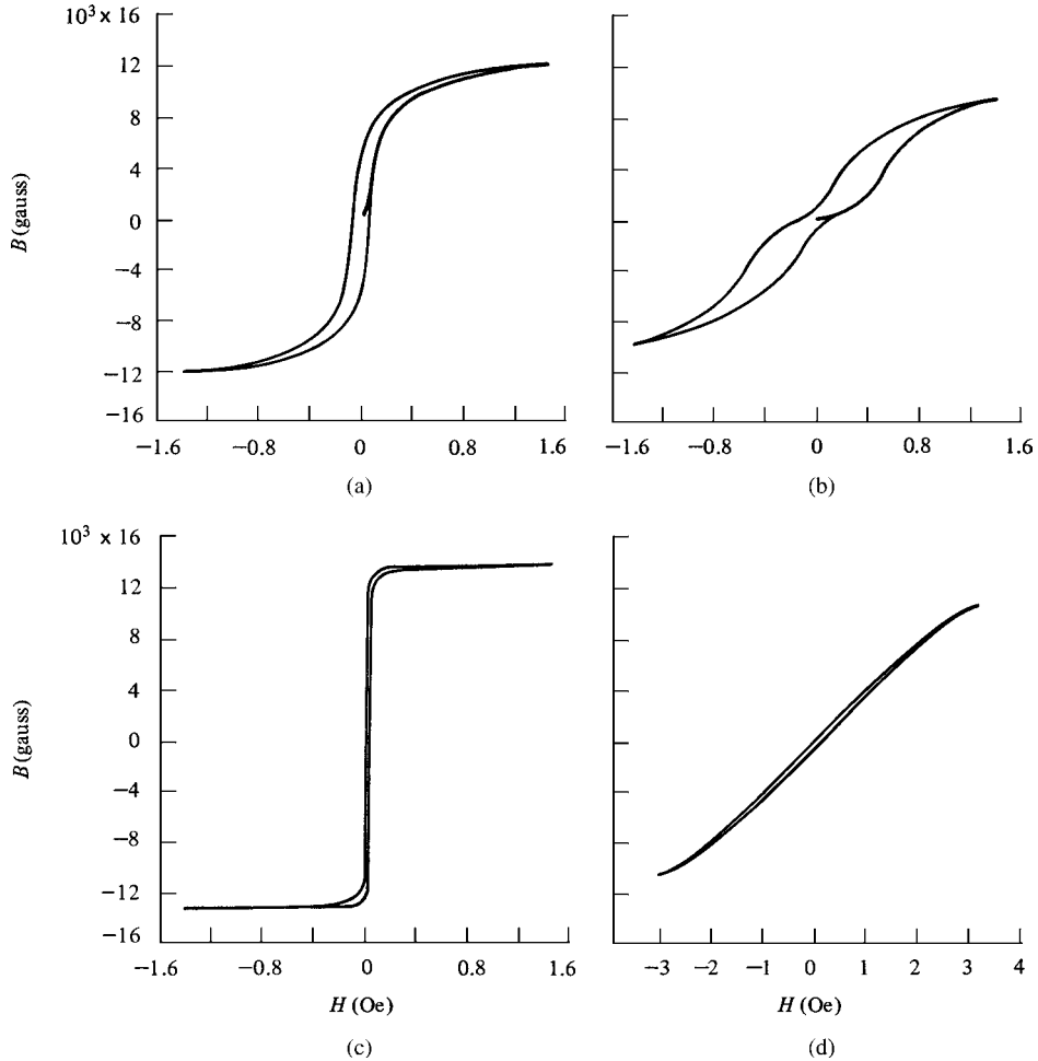
Fig. 10.2 Hysteresis loops of a 65 Ni–35 Fe alloy after various heat treatments: (a) annealed at 1000°C and cooled quickly, (b) annealed at 425°C or cooled slowly from 1000°C, (c) annealed at 1000°C and cooled in a longitudinal field, (d) same as (c) but with a transverse field. [R. M. Bozorth, Ferromagnetism , reprinted by IEEE Press (1993).]
