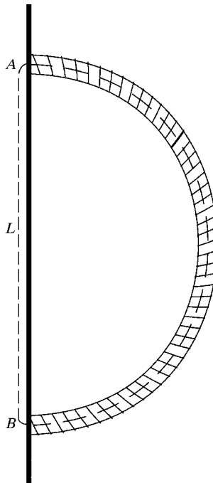
Fig. 2.18 Sketch of Chattock coil or magnetic potentiometer.
