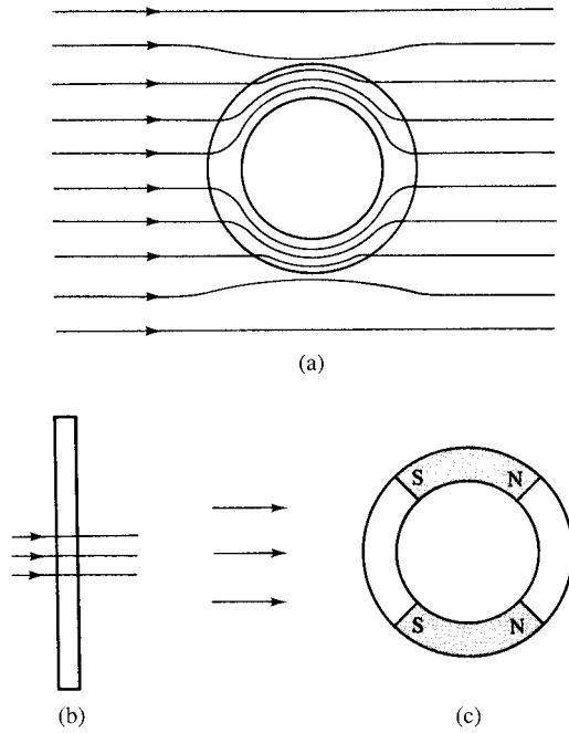
Fig. 2.25 Magnetic shielding.
