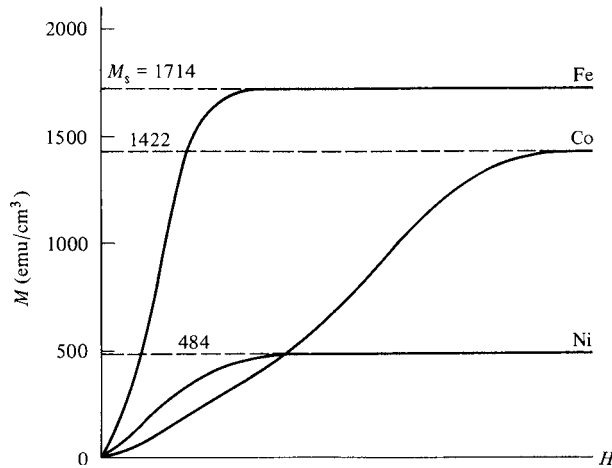
Fig. 4.1 Magnetization curves of iron, cobalt, and nickel at room temperature ( H -axis schematic). The SI values for saturation magnetization in A/m are 10^3 times the cgs values in emu/cm 3 .
