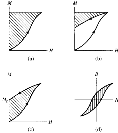
Fig. 7.23 Work done in magnetization.
