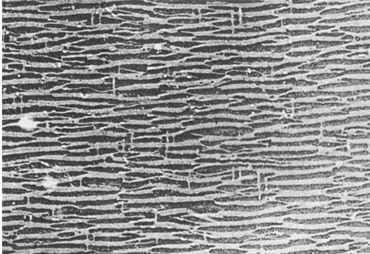
Fig. 14.9 Electron micrograph (oxide replica) from a single crystal of field-annealed alnico. The field during annealing was directed horizontally; 50,000\times [K. J. De Vos, Magnetism and Metallurgy , Volume 2, Academic Press (1969)].
