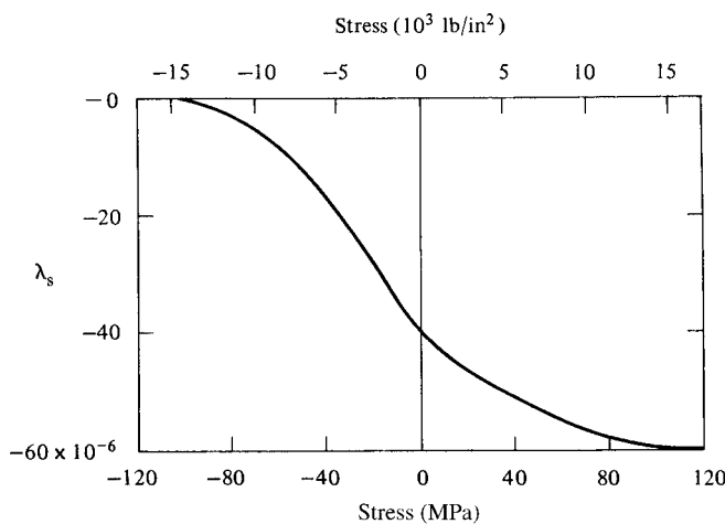
Fig. 8.23 Saturation magnetization of nickel under tension and compression. [H. Kirchner, Ann. Phys. , 27 (1936) p. 49.]
