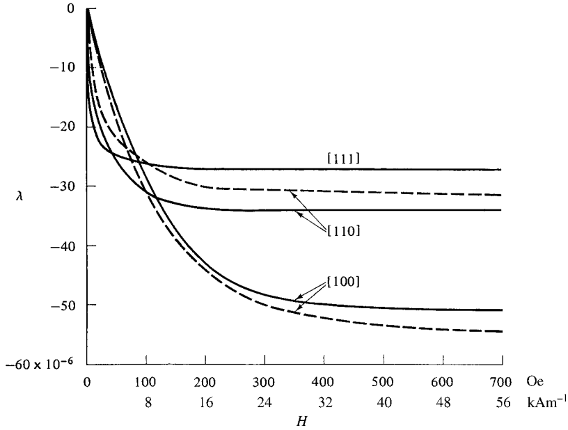
Fig. 8.6 Magnetostriction as a function of field and crystal direction for nickel single crystal. Samples were planetary (oblate) spheroids. Solid lines, {011} disk; dashed lines, {001} disk. [Y. Masiyama, Sci. Rep. Tohoku Univ. , 17 (1928) p. 947.]
