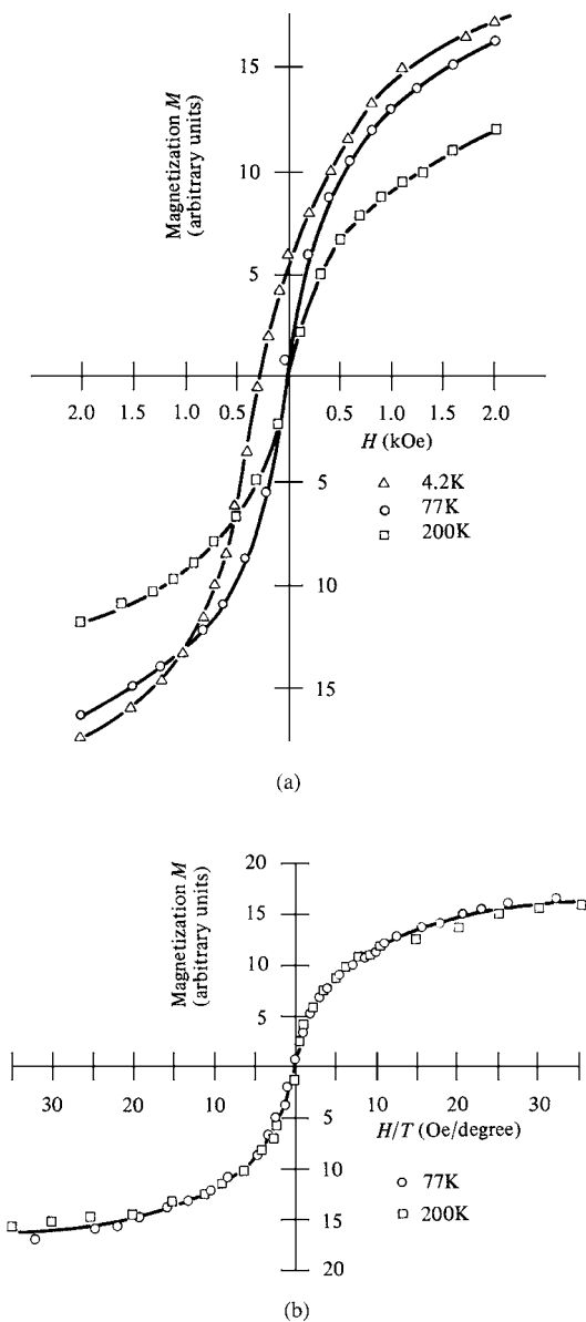
Fig. 11.18 Magnetization curves of iron particles 44 Å in diameter. [I. S. Jacobs and C. P. Bean, Magnetism , Volume 3, G. T. Rado and H. Suhl, eds., Academic Press (1966).]
