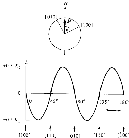
Fig. 7.13 Variation of torque L with angle \theta in the \{001\} plane of a cubic crystal for K_1 > 0 .
