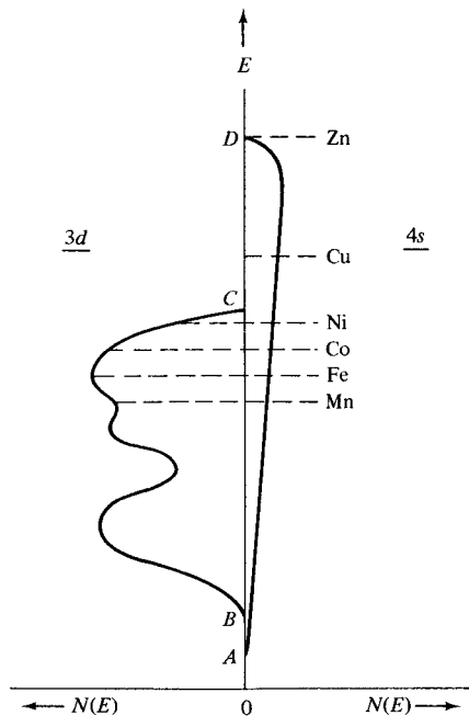
Fig. 4.16 Density of levels in the 3 d and 4 s bands (schematic).
