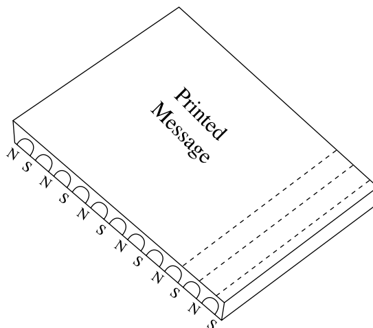
Fig. 14.14 “One-sided” magnet. Only the nonprinted side will stick to a steel surface.
