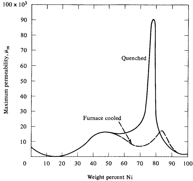
Fig. 13.20 Maximum permeabilities of iron–nickel alloys.
