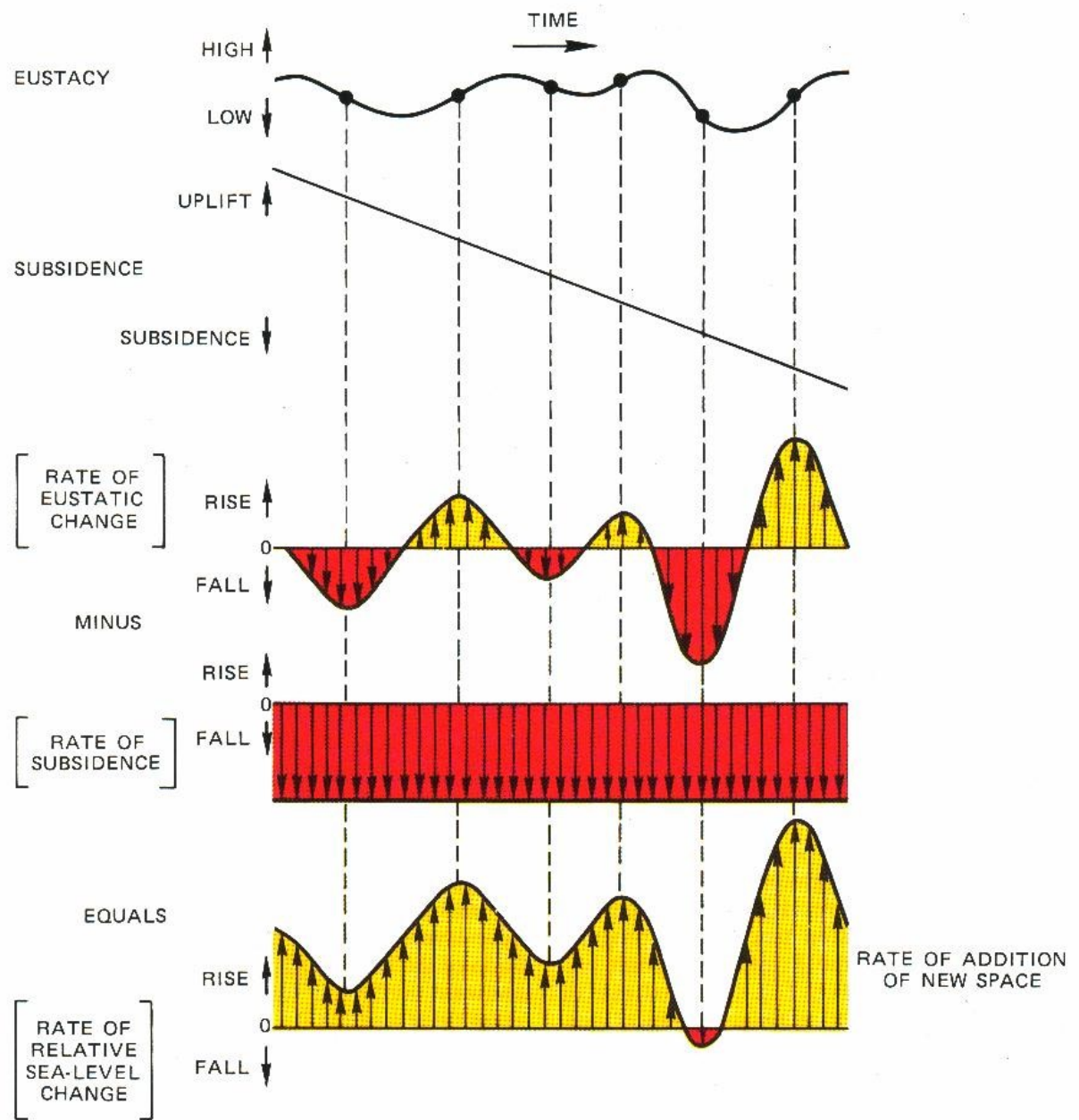
FIG. 10.—Relative sea level as a function of eustacy and subsidence.
