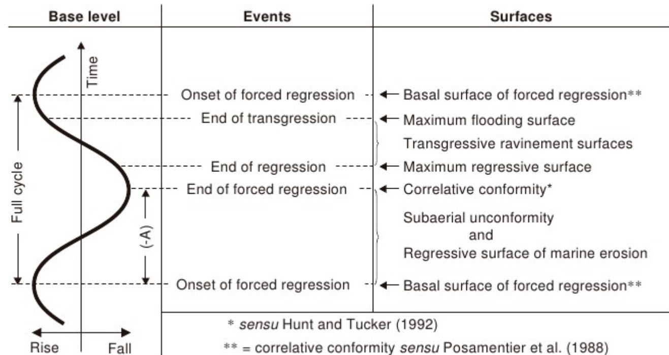
FIGURE 4.7 Timing of sequence stratigraphic surfaces relative to the main events of the base-level cycle (modified from Catuneanu et al. , 1998b, and Embry and Catuneanu, 2002). (-A)—negative accommodation. Each of these seven surfaces of sequence stratigraphy can serve, at least in part, as systems tract boundaries. The ‘transgressive ravinement surfaces’ include a pair of wave- and tidal- ravinement surfaces, which are often superimposed, especially in open shoreline settings. In river-mouth settings, the two transgressive ravinement surfaces may be separated by estuary-mouth complex deposits.
