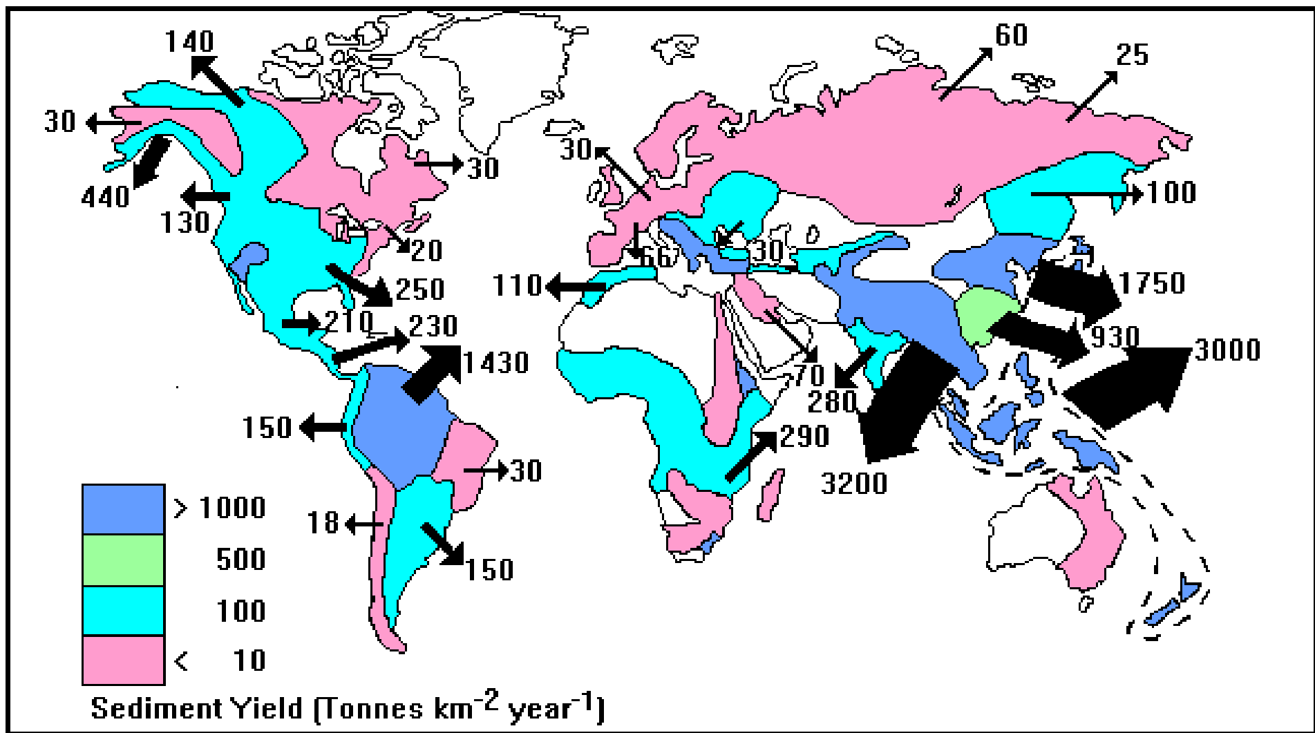
Figure 5 Global pattern of sediment yield, with river output of sediment to the oceans (tonnes x10 6 ) (Ref. 6). (Reproduced by permission)
