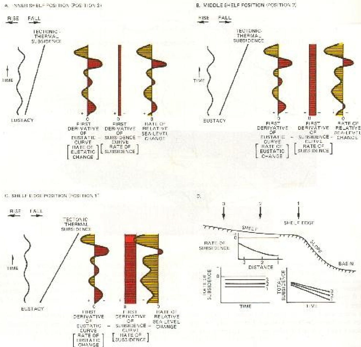
Fig. 13.— Response of relative sea level to differential tectonic thermal subsidence.
