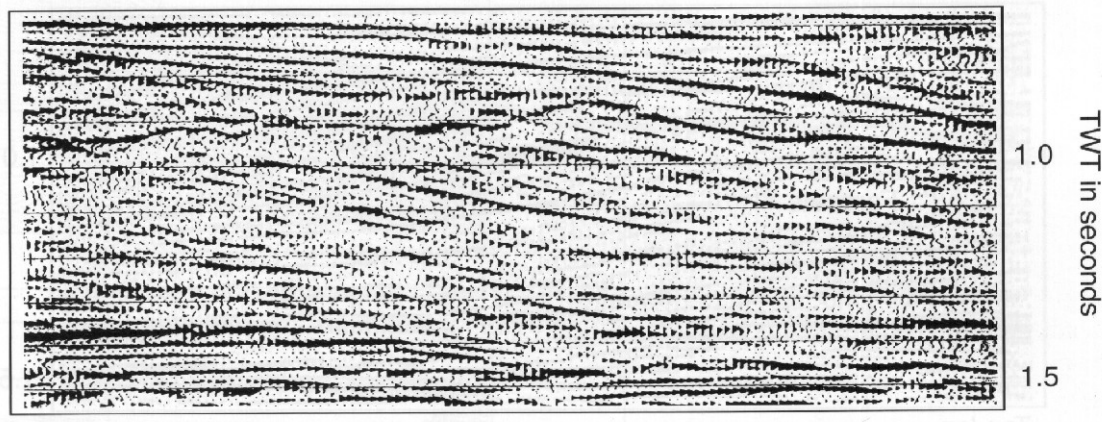
Erosional truncation
