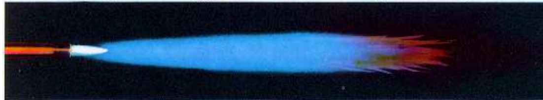
Neutral Flame (Acetylene and oxygen.) Temp. 5600 F. For fusion welding of steel and cast iron.
