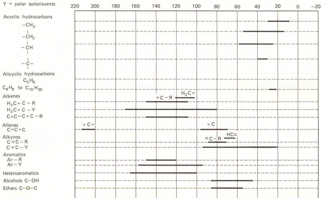
^{13}\text{C} Correlation Chart for Chemical Classes
