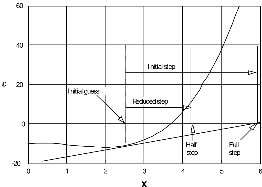
Figure 2: Use step-halving for improving the convergence
