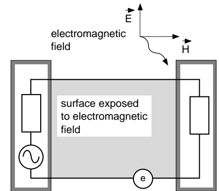
fig. 9: an example of differential mode field to wire coupling.
