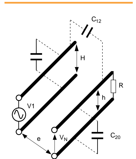
fig. 13: a rapid change in V1 creates a field which at a short distance can be assumed to be purely electric and induces a voltage V N in another wire-like structure which runs in parallel; this mode of coupling is called capacitive crosstalk.
