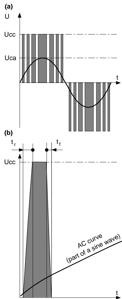
fig. 4: a source of disturbances in power electronics: pulse width modulation. a: principle, b: even with the time scale not well chosen for this type of phenomenon t_r \approx 2 to 3 t_f (10 ns to 1 \mu\text{s} ) while the sine wave covers 20 ms.
