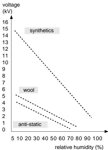
fig 22: the effect of relative humidity on the electrostatic discharge voltage for three types of floor materials.
