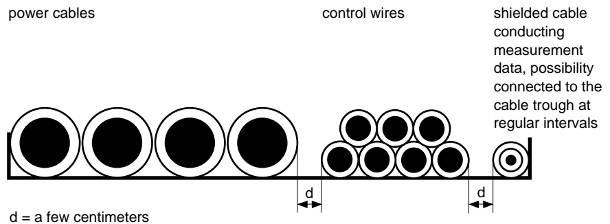
fig. 20: cable routing example.
