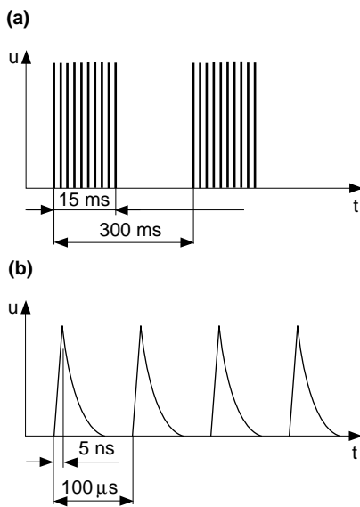
fig. 25: shape of the bursts (a) and their fast transients (b).
