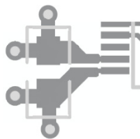
Good Bypassing
