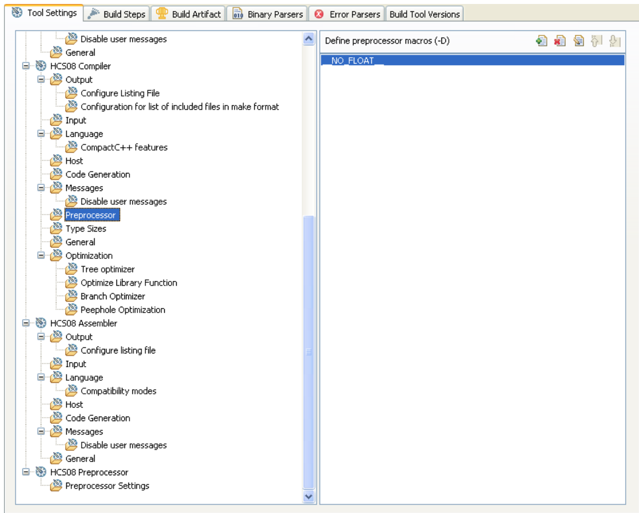
Figure 3-38. Tool Settings - HCS08 Compiler > Preprocessor
