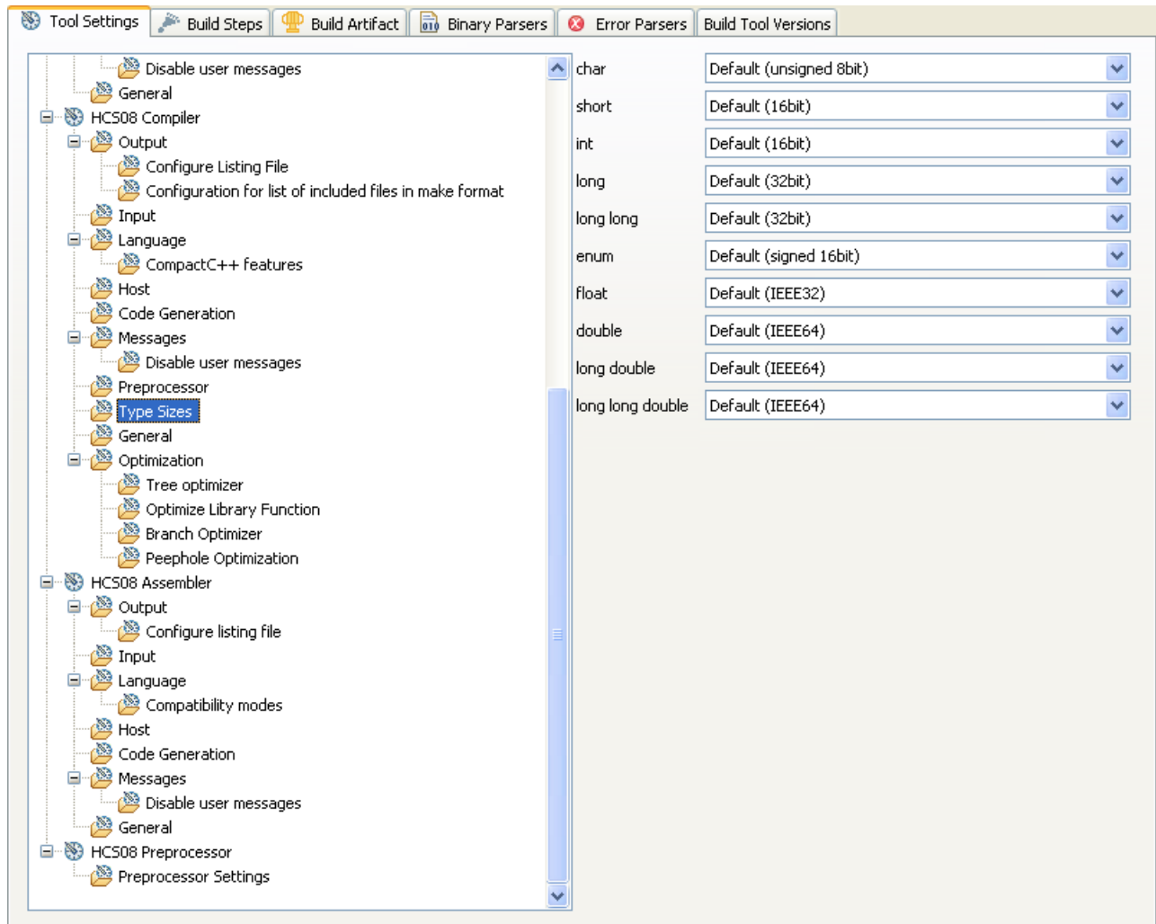
Figure 3-41. Tool Settings - HCS08 Compiler > Type Sizes
