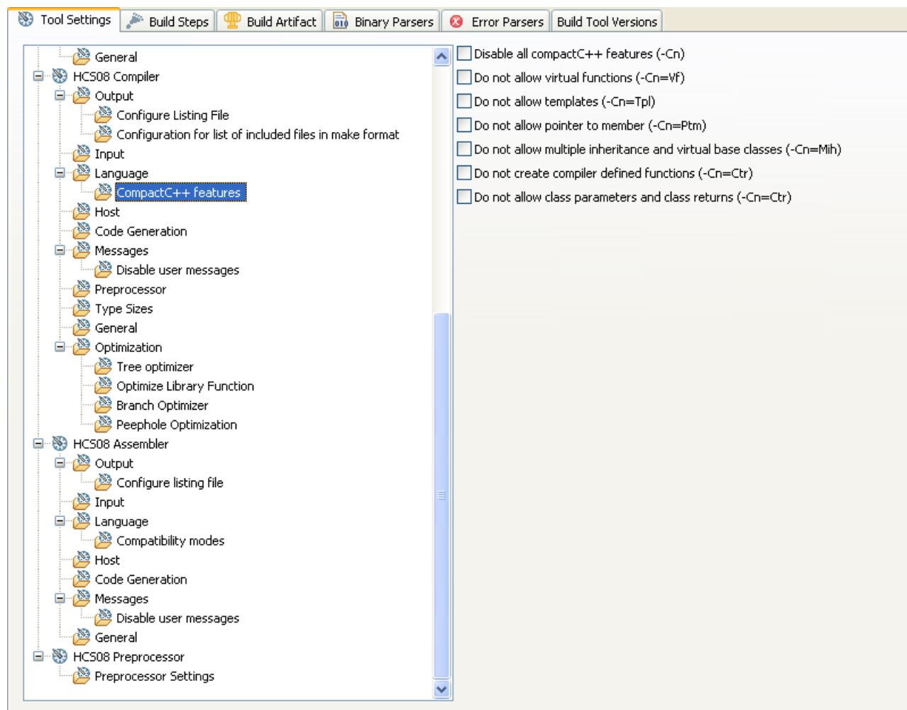
Figure 3-33. Tool Settings - HCS08 Compiler > Language > CompactC++ Features
