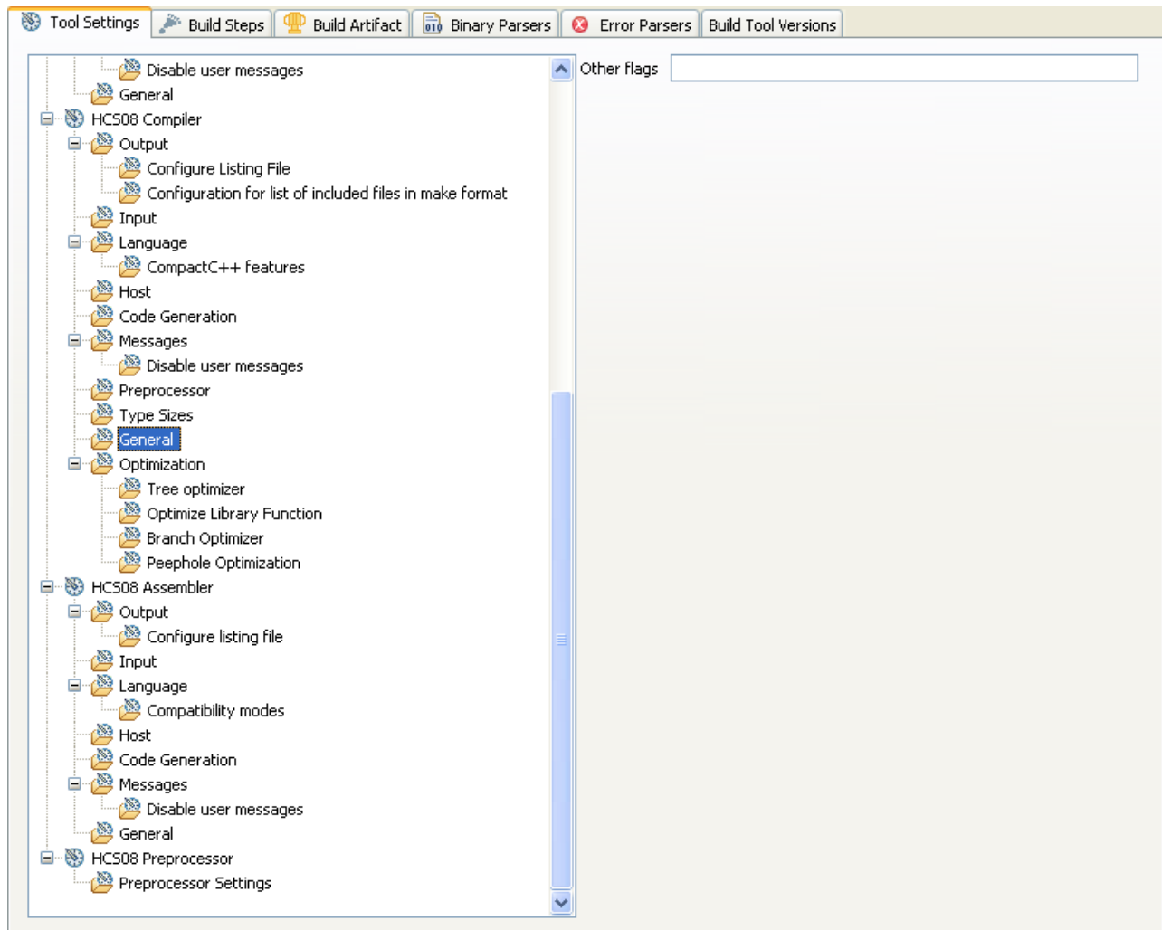
Figure 3-42. Tool Settings - HCS08 Compiler > General
