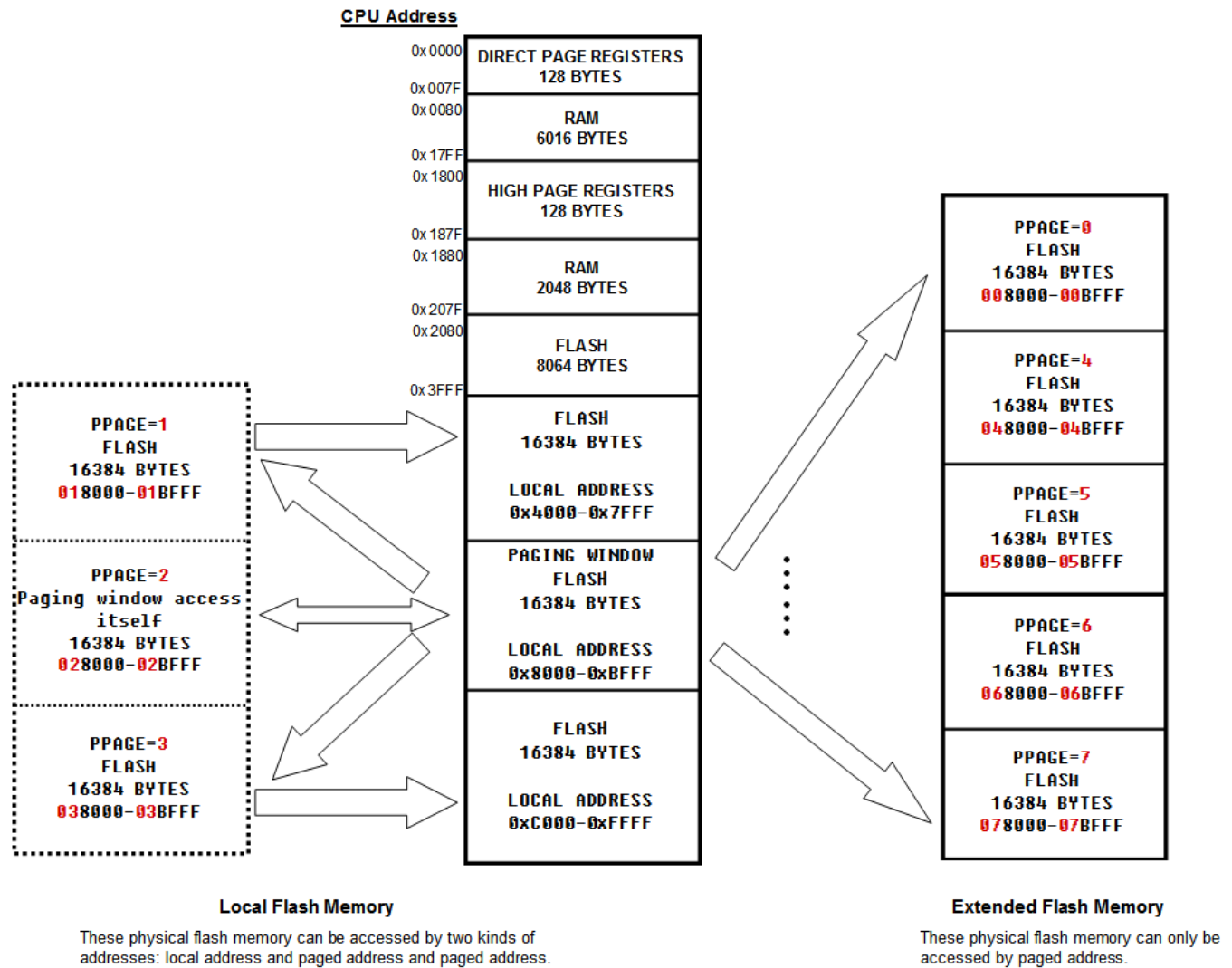
Figure 25-2. MC9S08QE128 Memory Map
