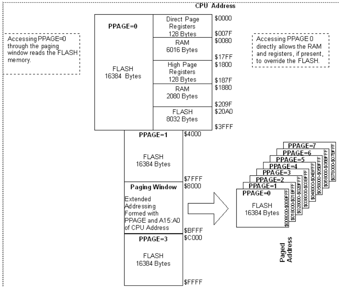
Figure 12-1. Example of Paging Mechanism
