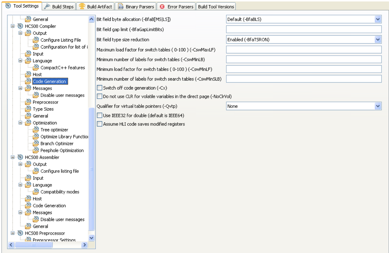
Figure 3-35. Tool Settings - HCS08 Compiler > Code Generation
