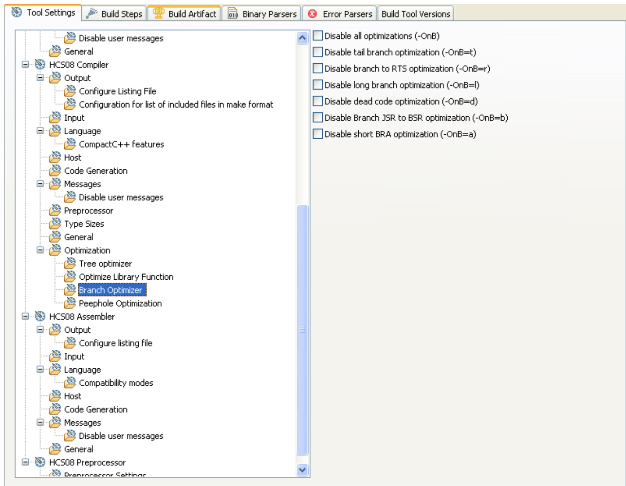
Figure 3-46. Tool Settings - HCS08 Compiler > Optimization > Branch Optimizer
