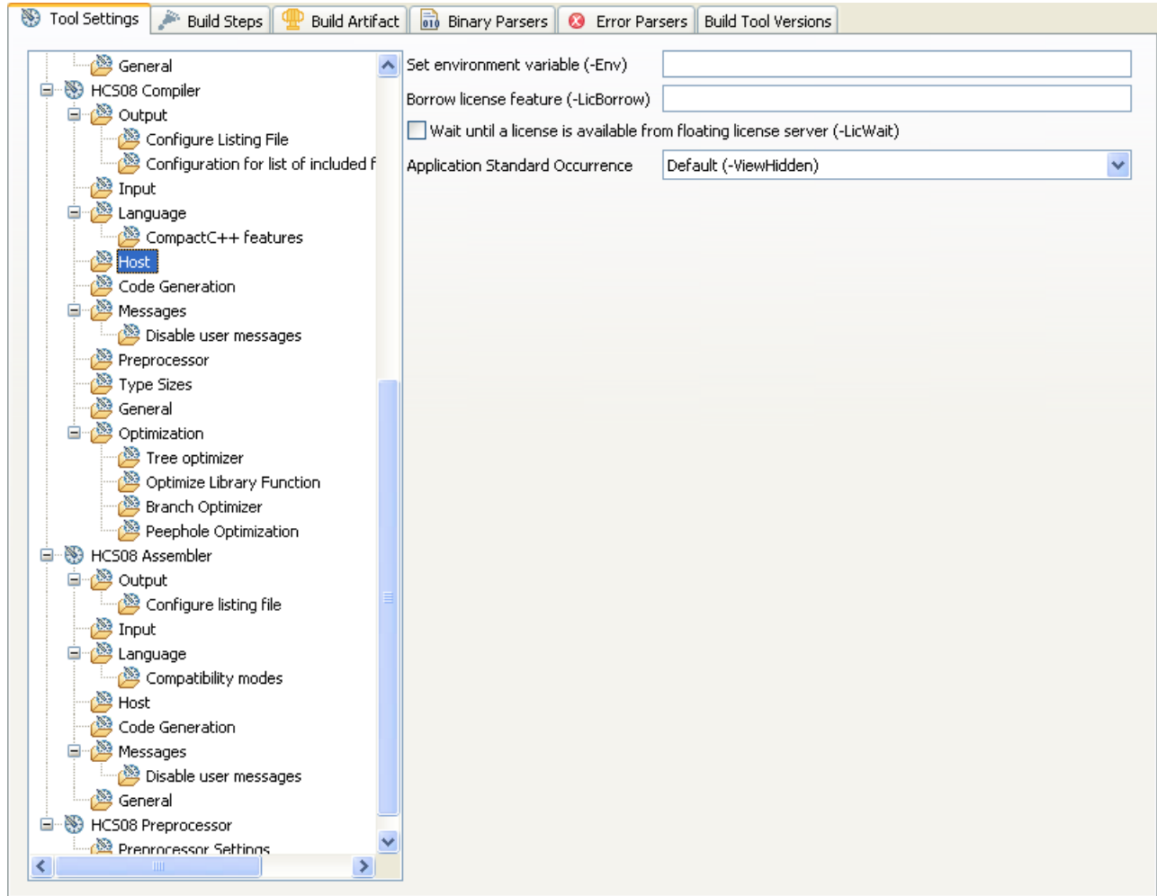
Figure 3-34. Tool Settings - HCS08 Compiler > Host
