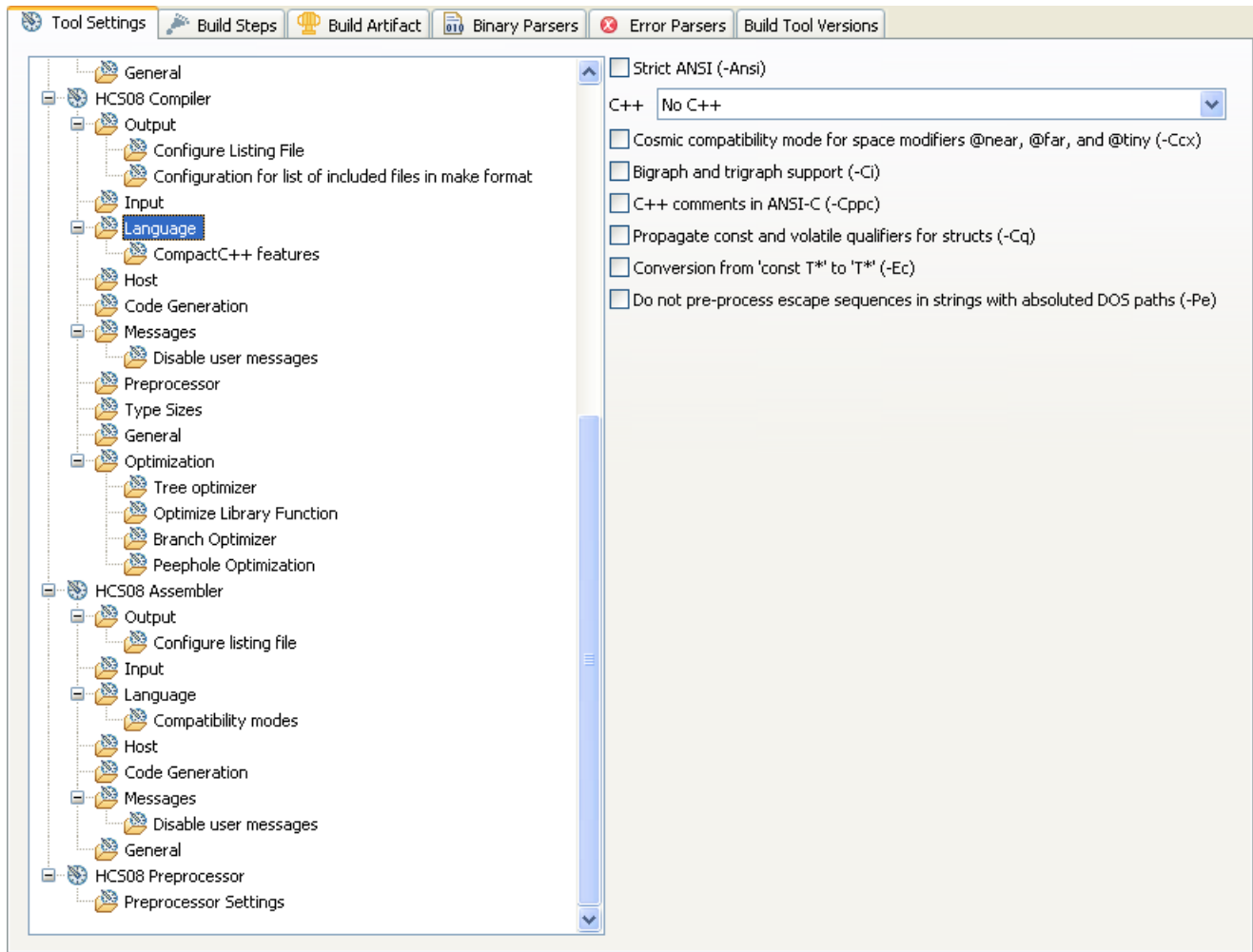
Figure 3-32. Tool Settings - HCS08 Compiler > Language
