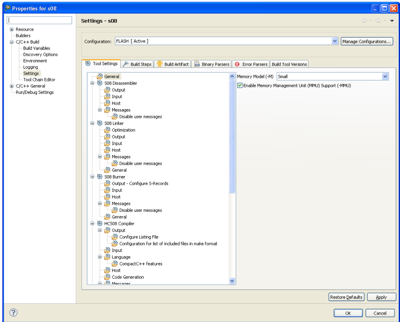
Figure 3-23. Project Properties Window
