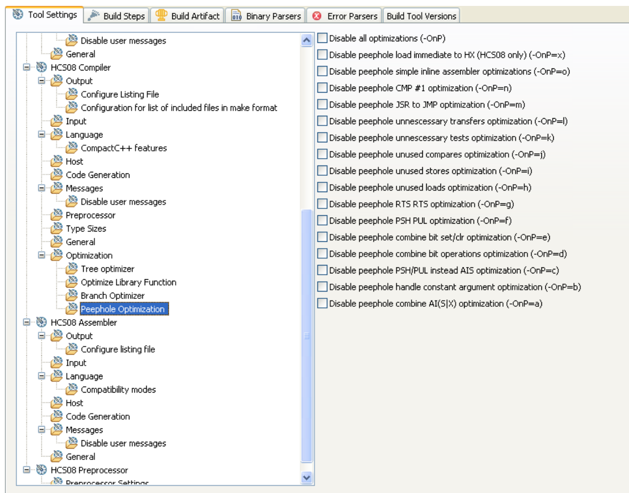
Figure 3-47. Tool Settings - HCS08 Compiler > Optimization > Peephole Optimization
