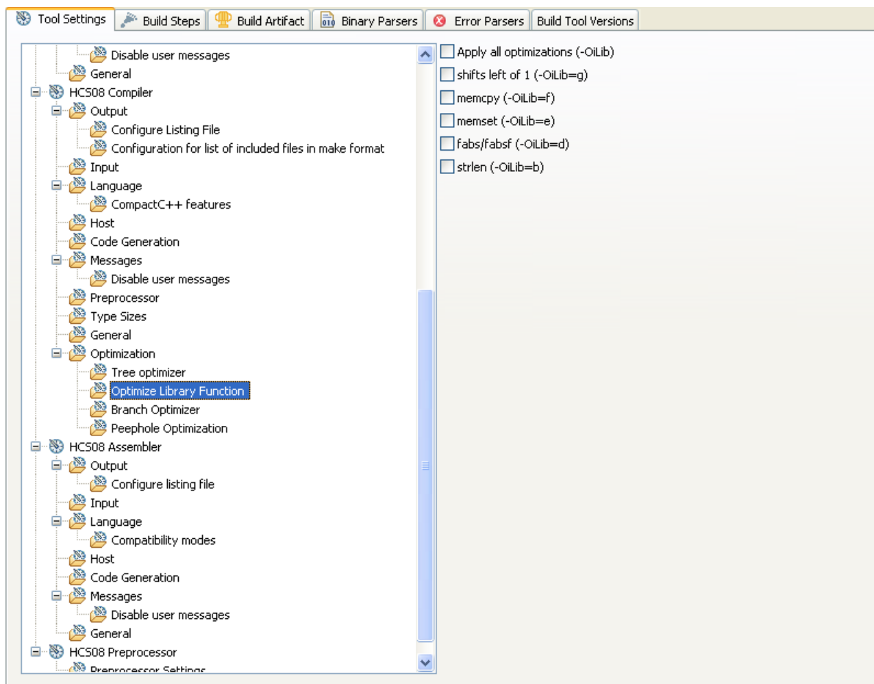
Figure 3-45. Tool Settings - HCS08 Compiler > Optimization > Optimize Library Function
