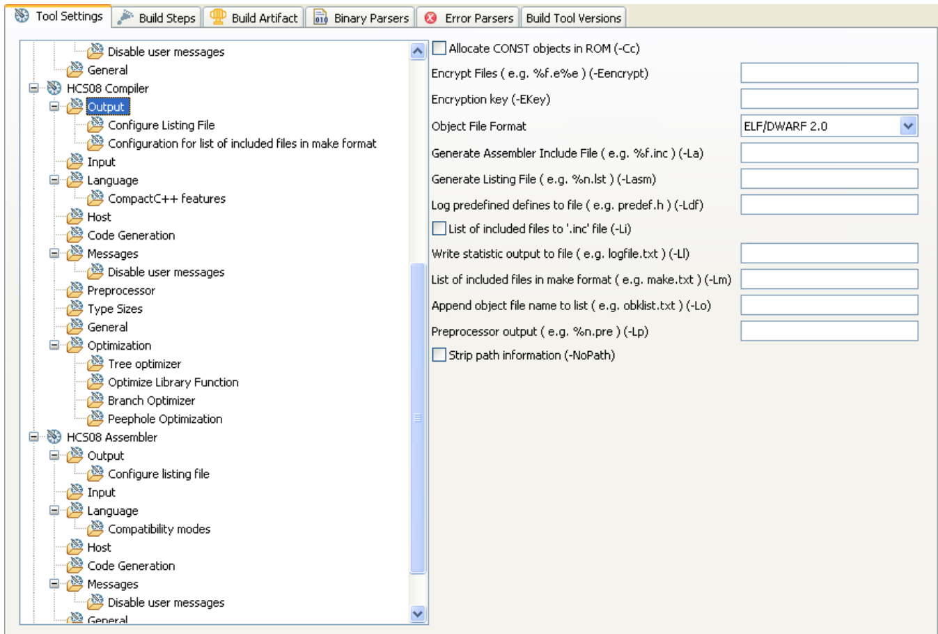
Figure 3-25. Tool Settings - HCS08 Compiler > Output
