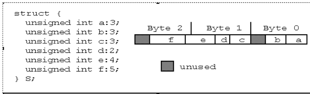
Figure 12-2. Allocation of Six Bitfields
