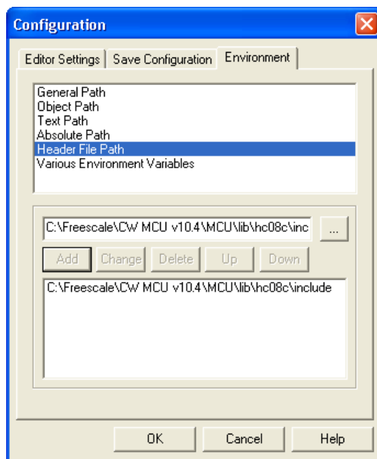
Figure 3-16. Adding Header File Path
