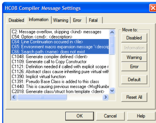
Figure 4-2. HC08 Compiler Message Settings Dialog Box
