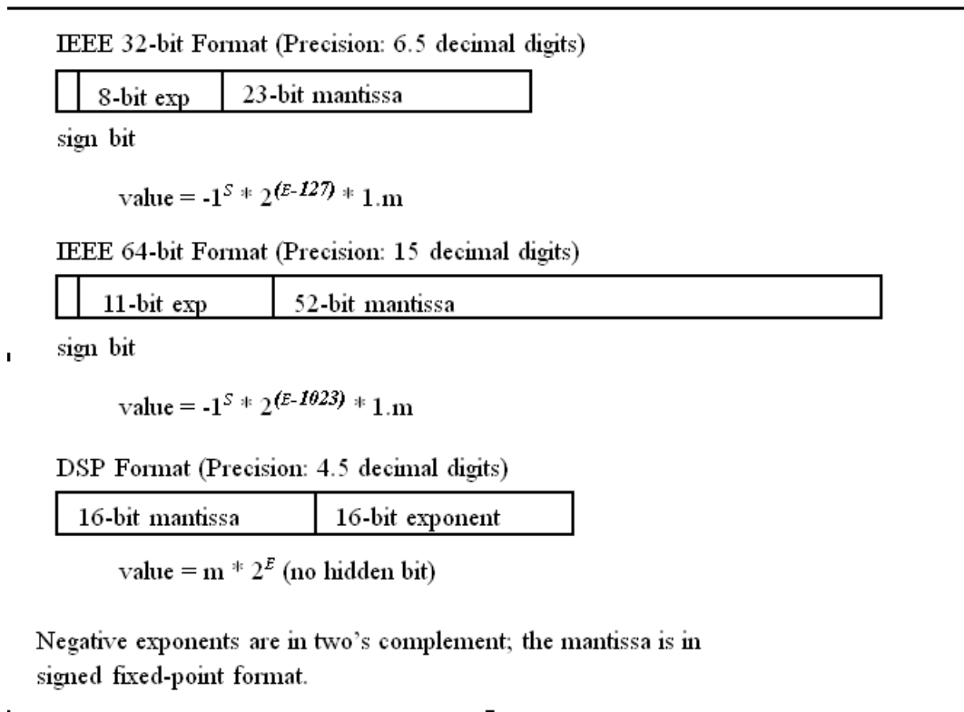
Figure 10-1. Floating-Point Formats
