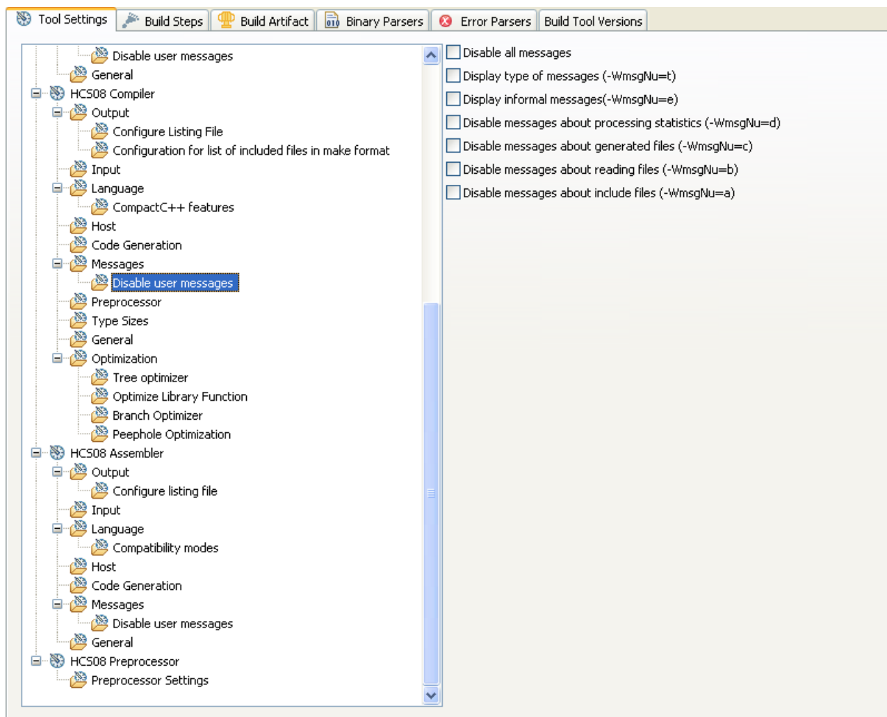
Figure 3-37. Tool Settings - HCS08 Compiler > Messages > Disable user messages
