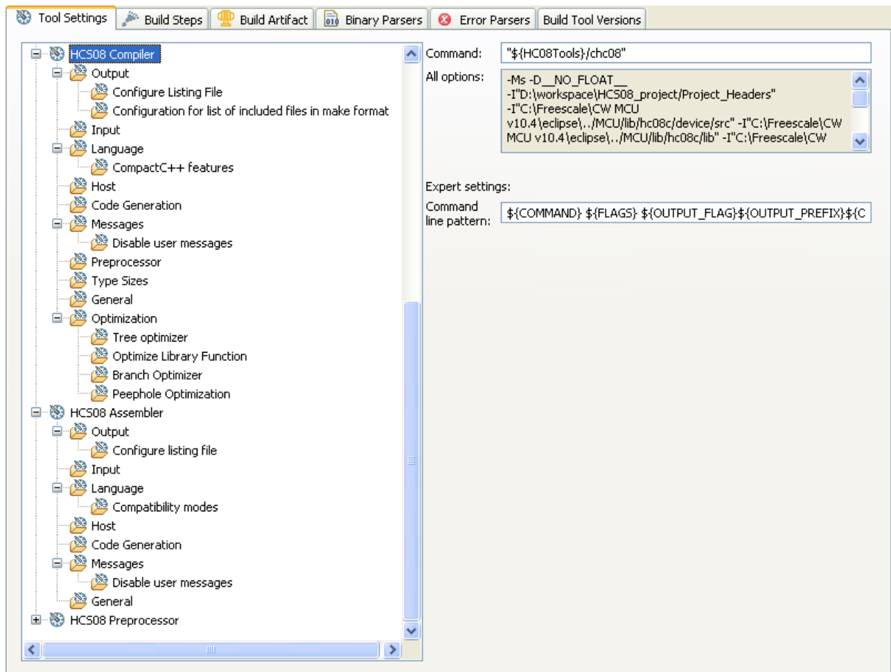
Figure 3-24. Tool Settings - HCS08 Compiler
