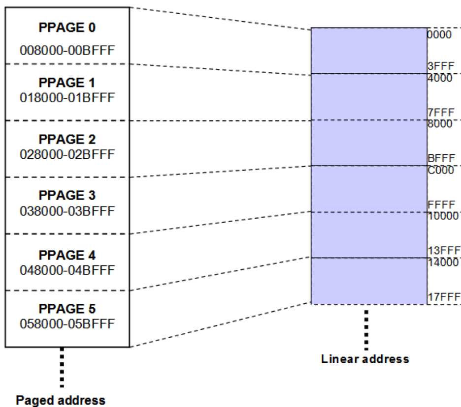
Figure 25-3. Paged/Linear Address Equivalence for MC9S08QE128 Derivative
