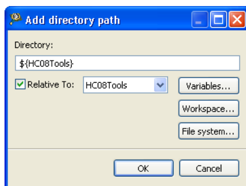
Figure 3-28. Tool Settings - HCS08 Compiler > Input - Add Directory Path Dialog Box
