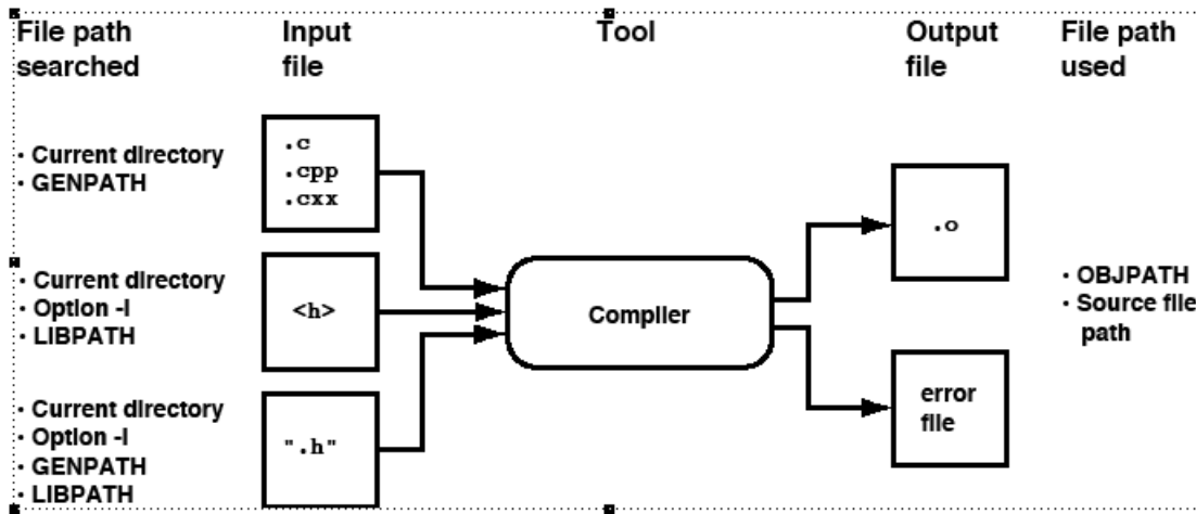
Figure 6-1. Files Used with the Compiler
