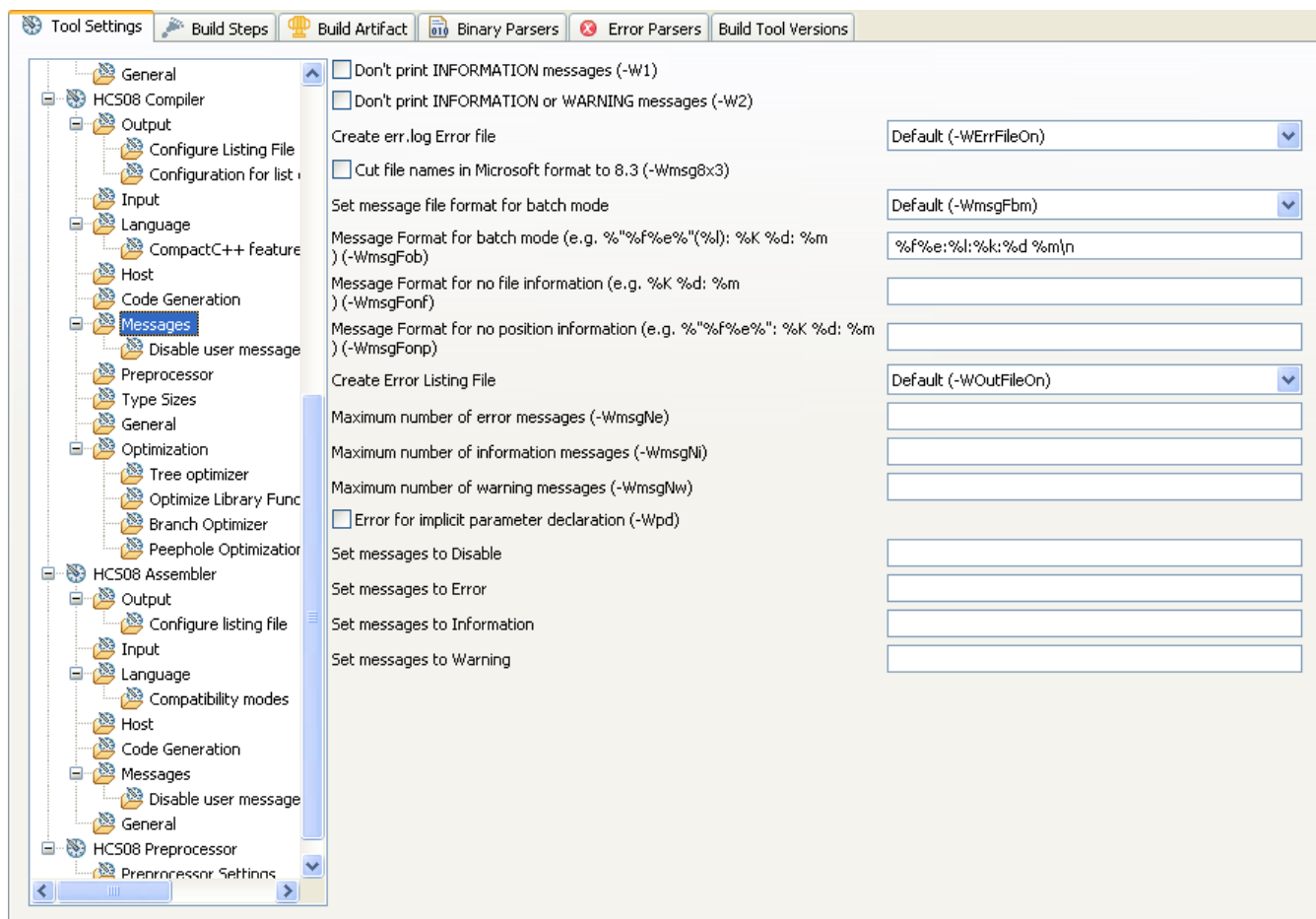
Figure 3-36. Tool Settings - HCS08 Compiler > Messages
