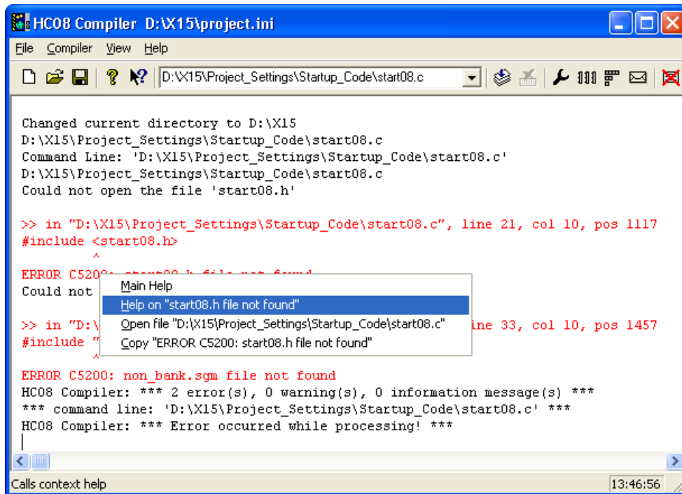
Figure 3-13. HC08 Compiler Window - Context Menu
