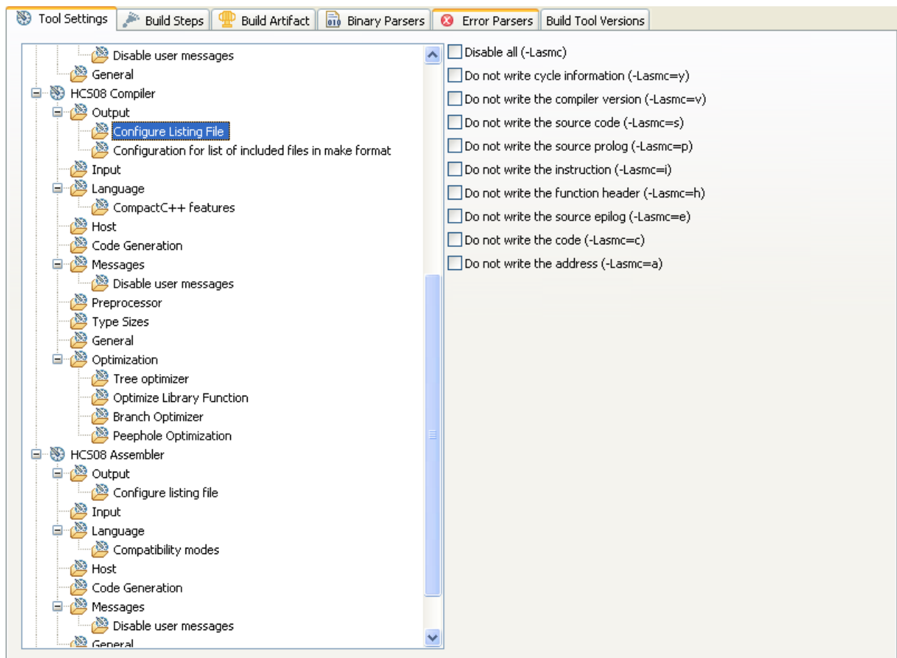
Figure 3-26. Tool Settings - HCS08 Compiler > Output > Configure Listing File
