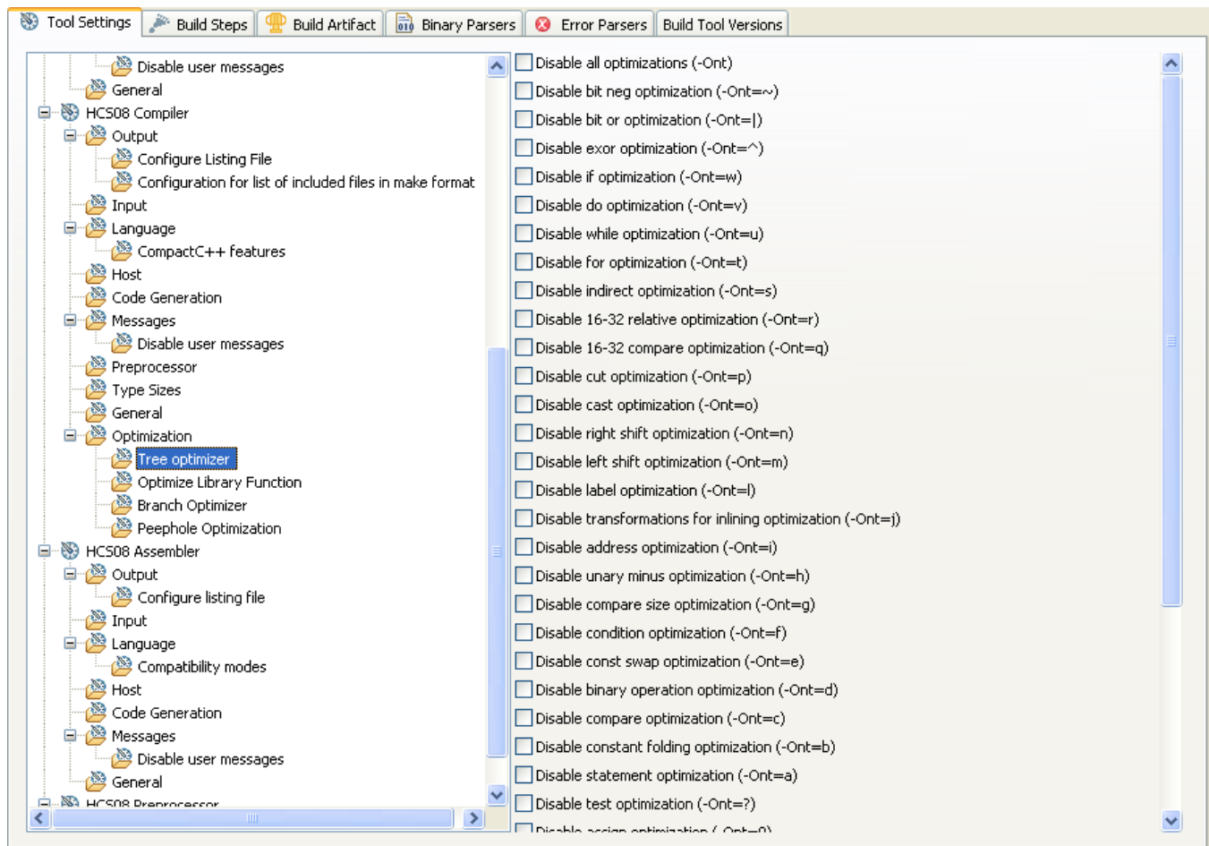
Figure 3-44. Tool Settings - HCS08 Compiler > Optimization > Tree optimizer
