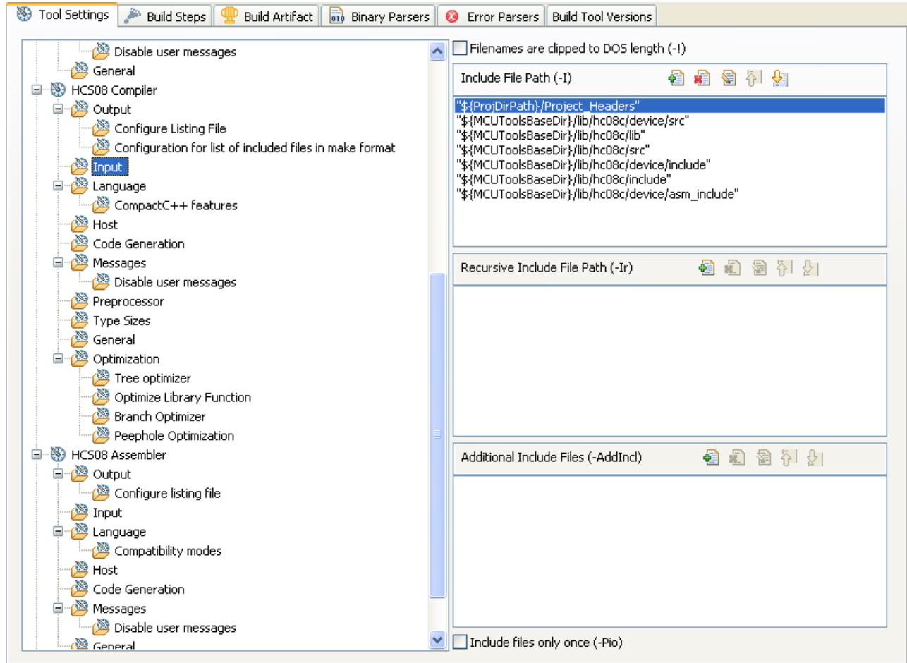
Figure 3-27. Tool Settings - HCS08 Compiler > Input
