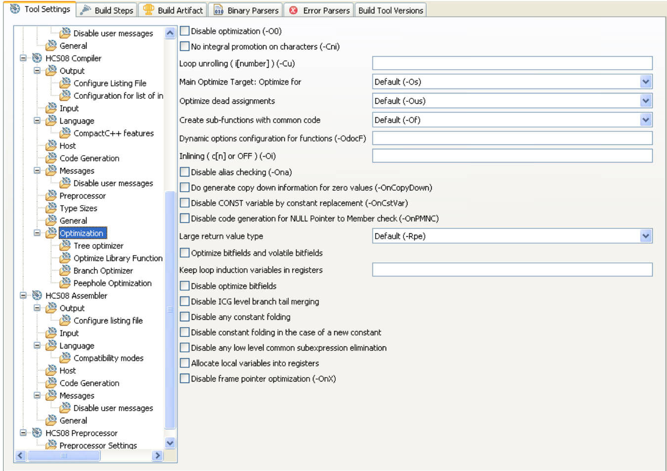
Figure 3-43. Tool Settings - HCS08 Compiler > Optimization
