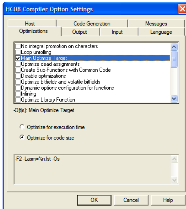
Figure 7-1. HC08 Compiler Option Settings Dialog Box
