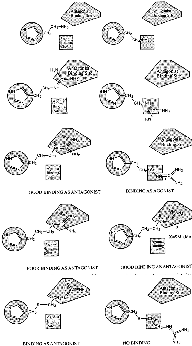
Fig. 13.33 Four-carbon unit chain.
