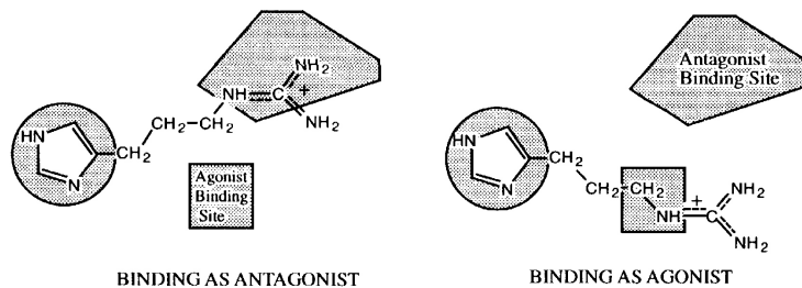
Fig. 13.34 Three-carbon unit chain.
