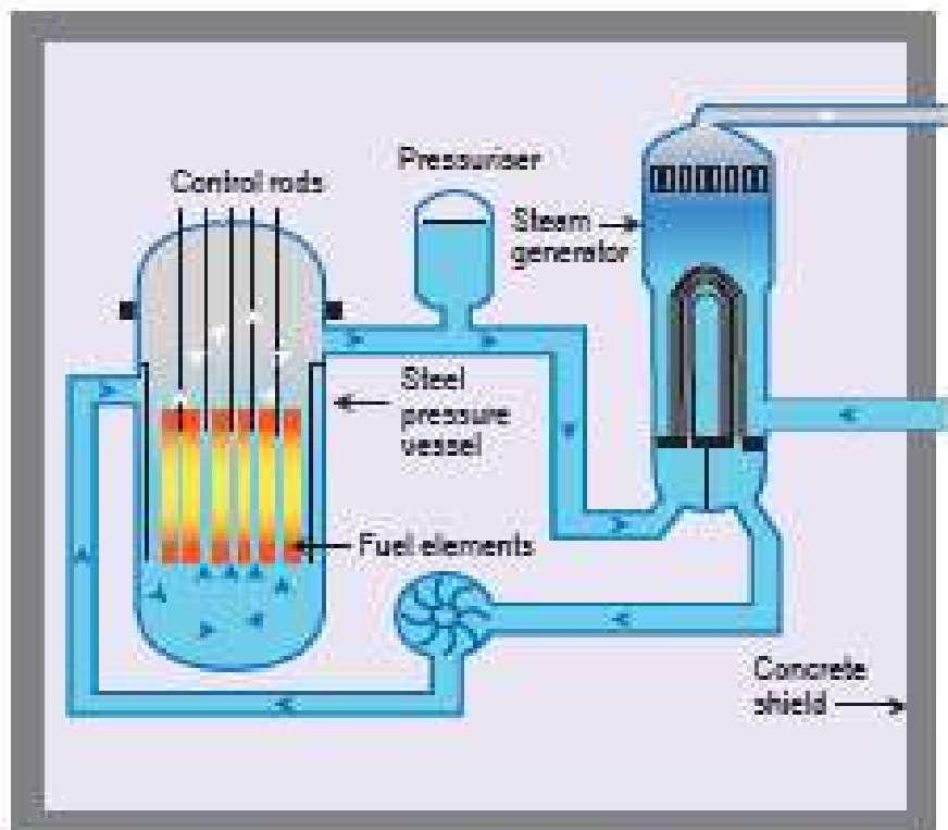
A typical Pressurised Water Reactor (PWR)
