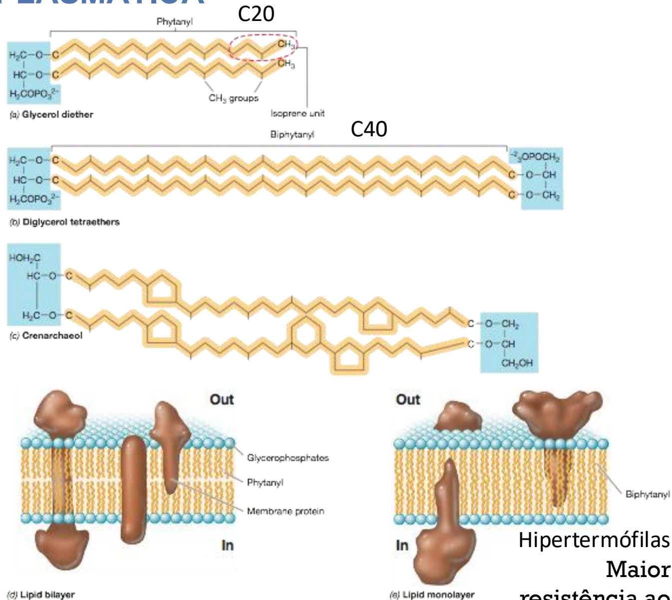
Figure 3.7 Major lipids of Archaea and the architecture of archaeal membranes. (a, b) Note that the hydrocarbon of the lipid is attached to the glycerol by an ether linkage in both cases. The hydrocarbon is phytanyl (C 20 ) in part a and biphytanyl (C 40 ) in part b. (c) A major lipid of Crenarchaeota is crenarchaeol, a lipid containing 5- and 6-carbon rings. (d, e) Membrane structure in Archaea may be bilayer or monolayer (or a mix of both).
